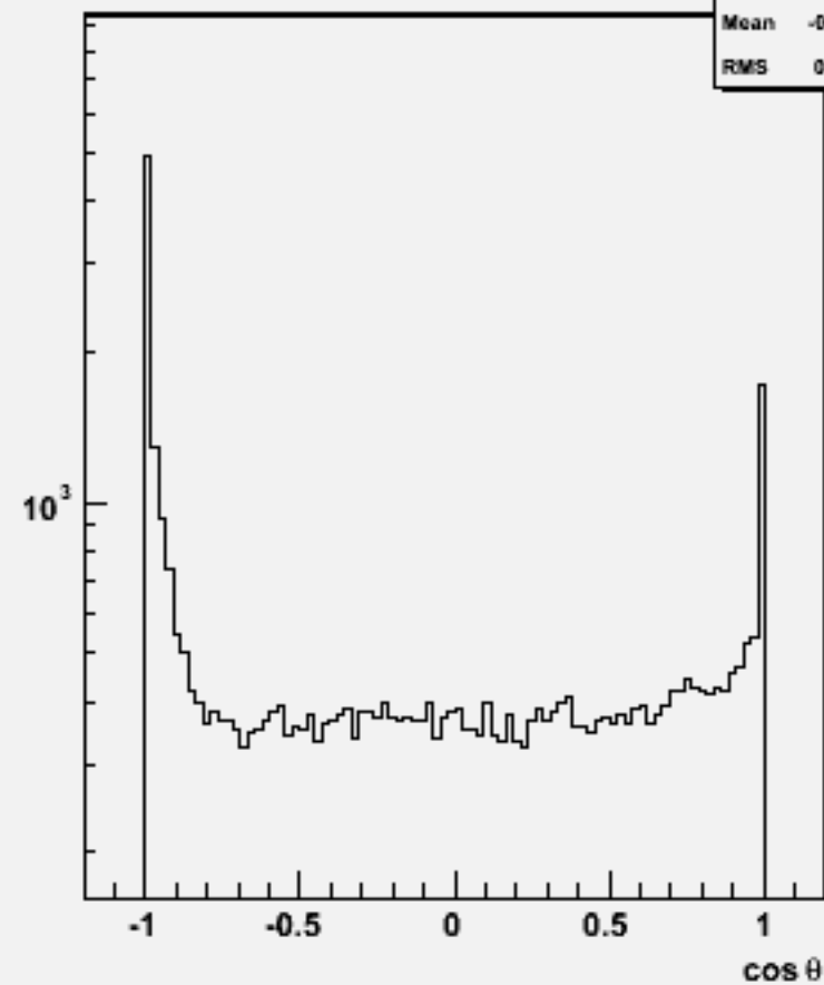
Jet cos \theta (All jets)w103026 e1a_n1ccsc_o
