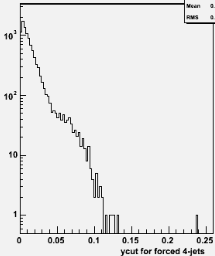
Ycut for 4-jets :w103026 e1a_n1ccsc_o
