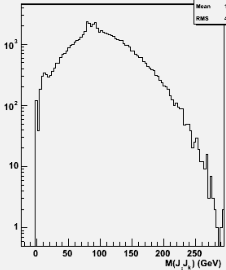
2jets mass(All comb)w103026 e1a_n1ccsc_o
