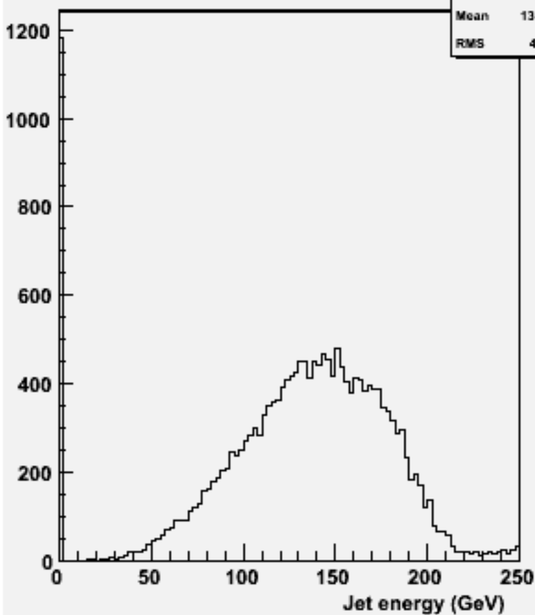
energy for 2-jets :w103022 e1a_n1ccdu_o
