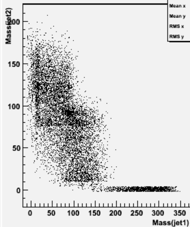
Jet mass for forced 2-jets : w103022 e1a_n1ccdu_o
