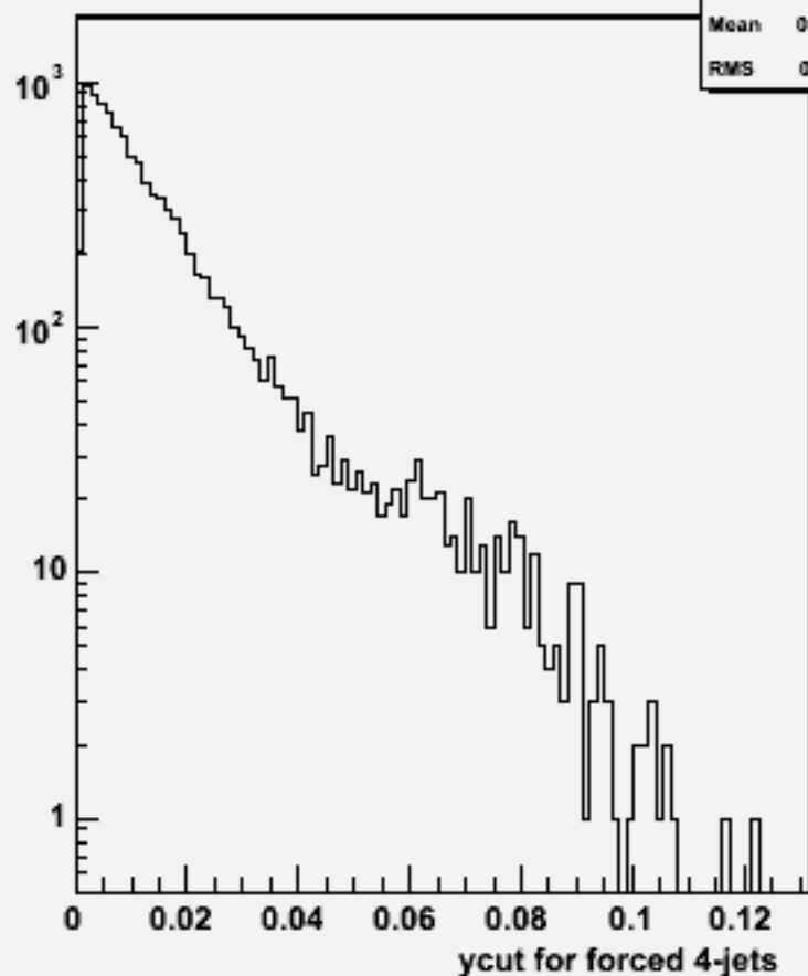
Ycut for 4-jets :w103022 e1a_n1ccdu_o
