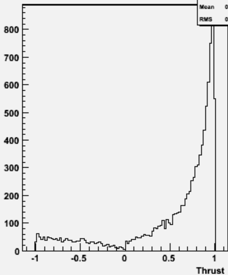
cos \Theta (thrust) w103022 e1a_n1ccdu_o
