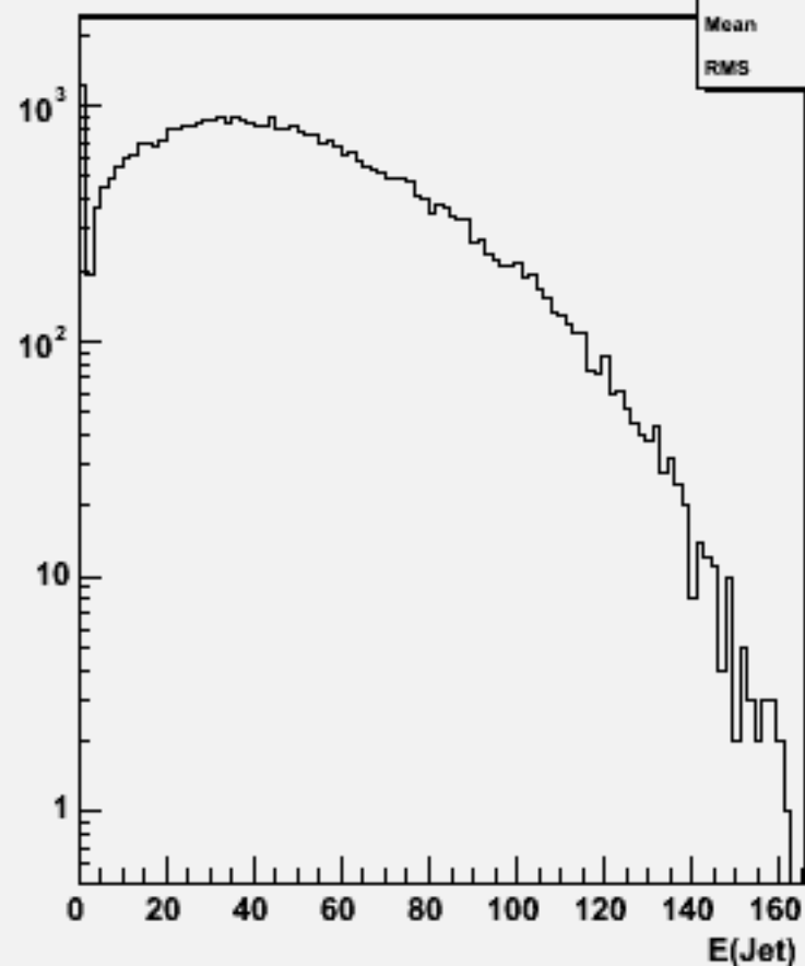
Jet energies(All jets)w103018 e1a_n1cce3n3_o
