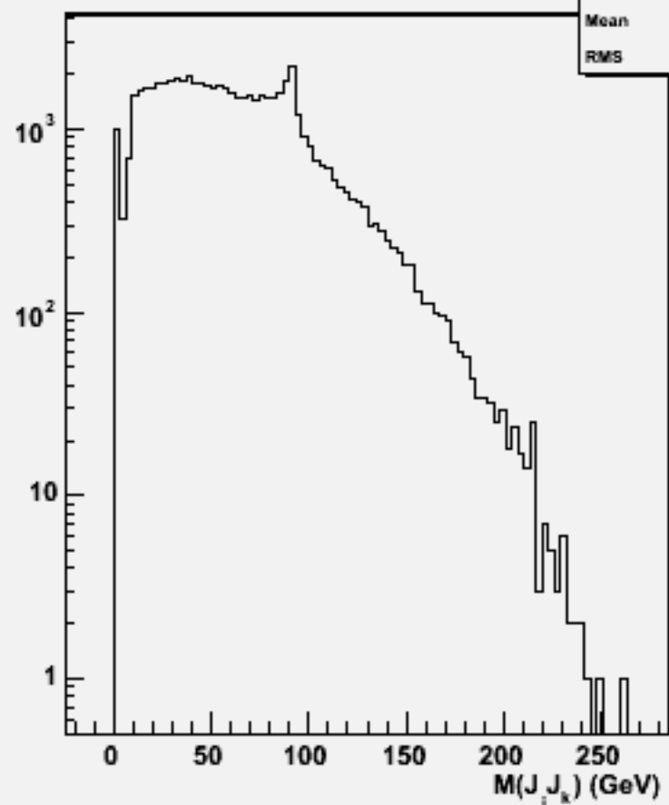
2jets mass(All comb)w103018 e1a_n1cce3n3_o
