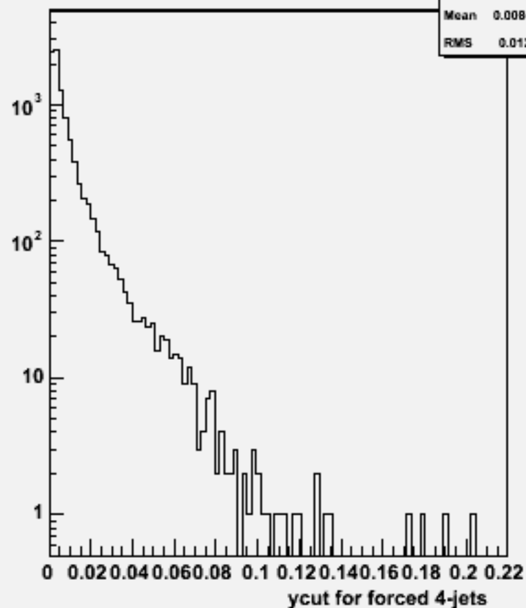
Ycut for 4-jets :w103018 e1a_n1cce3n3_o
