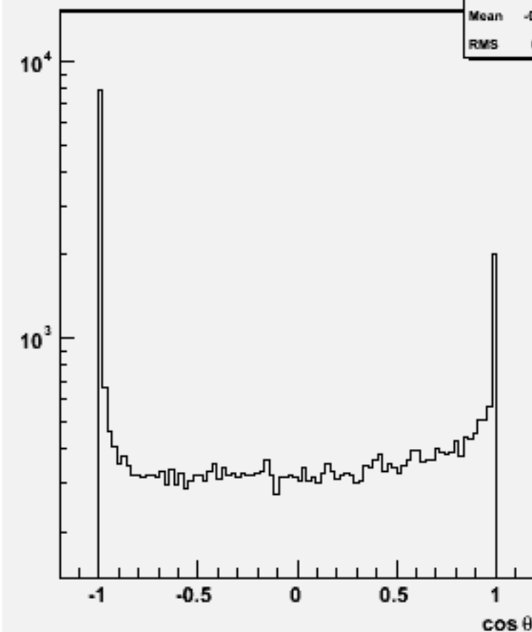
Jet cos \theta (All jets)w103018 e1a_n1cce3n3_o
