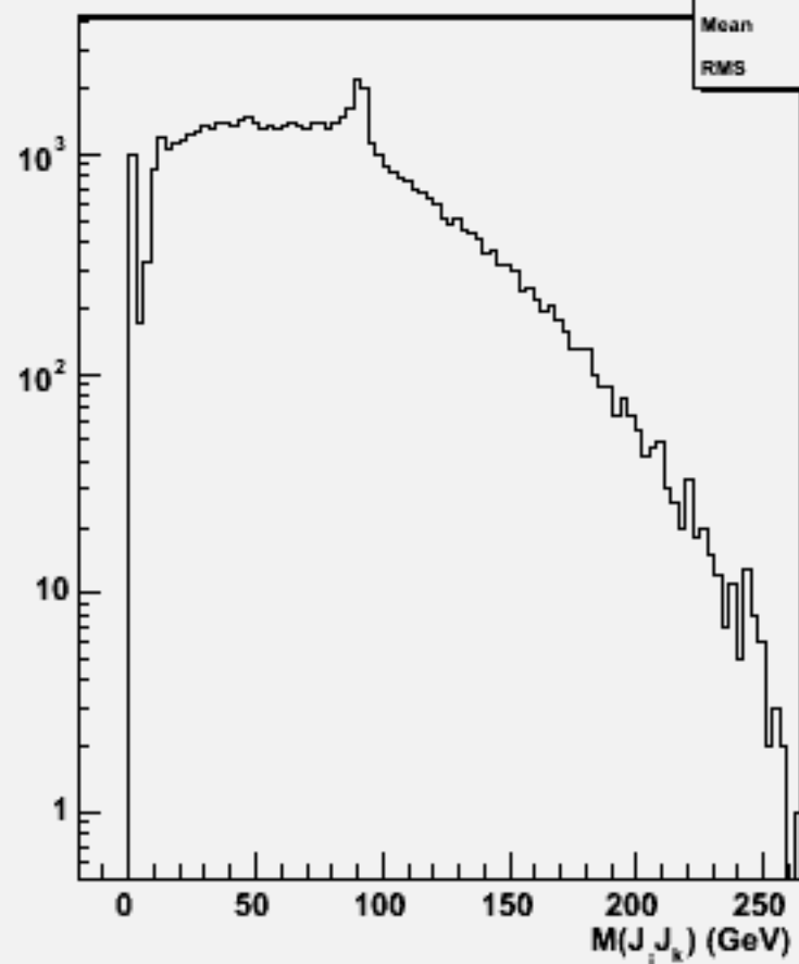
2jets mass(All comb)w103014 e1a_n1cce2n2_o
