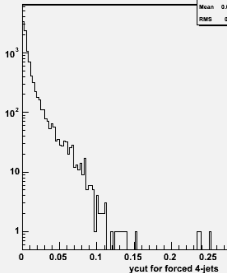
Ycut for 4-jets :w103014 e1a_n1cce2n2_o
