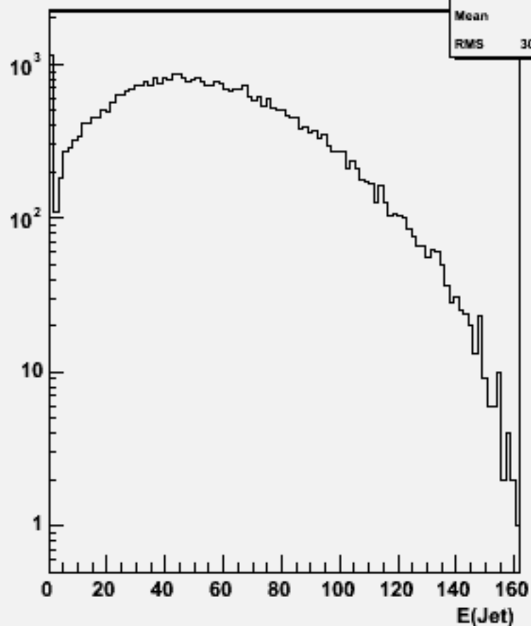
Jet energies(All jets)w103014 e1a_n1cce2n2_o
