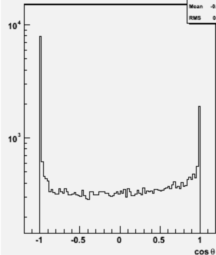
Jet cos \theta (All jets)w103014 e1a_n1cce2n2_o
