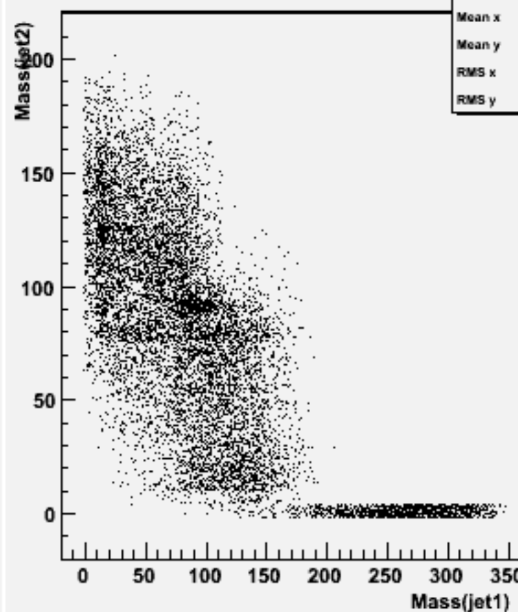
Jet mass for forced 2-jets : w103006 e1a_n1uusc_o
