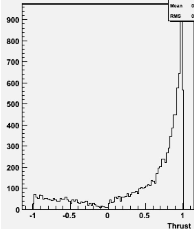
cos \Theta (thrust) w103006 e1a_n1uusc_o
