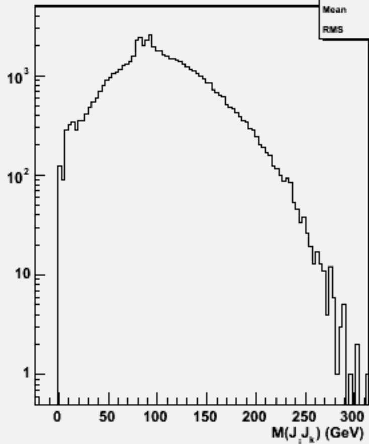
2jets mass(All comb)w103002 e1a_n1uu1du_o
