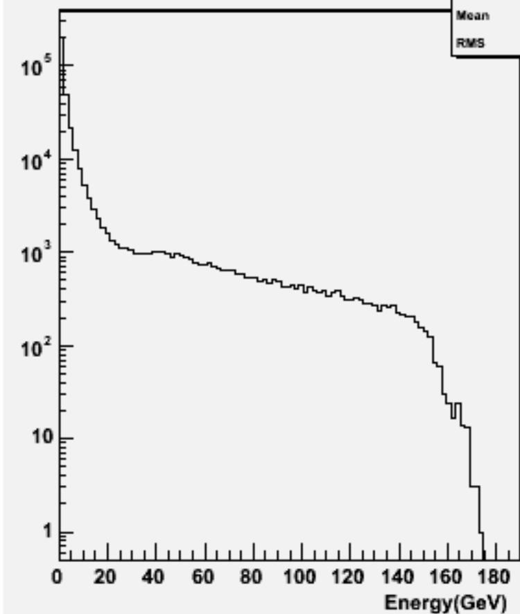
Particle Energy : w102992 e1a_n1uue1n1_o
