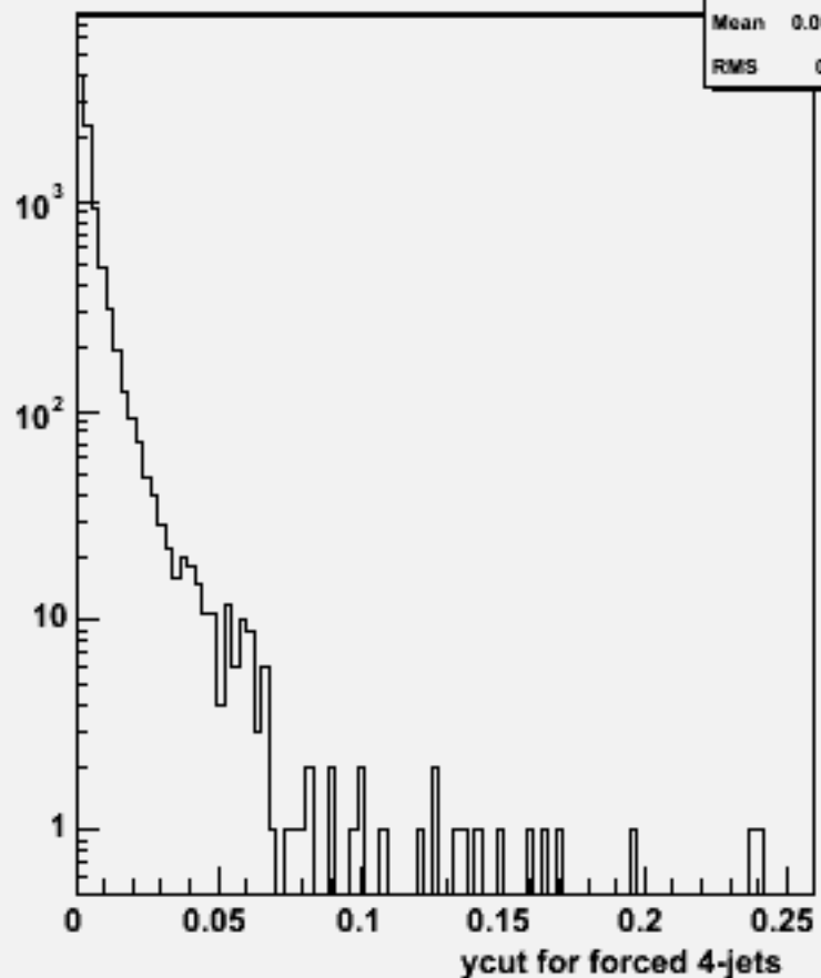
Ycut for 4-jets :w102992 e1a_n1uue1n1_o
