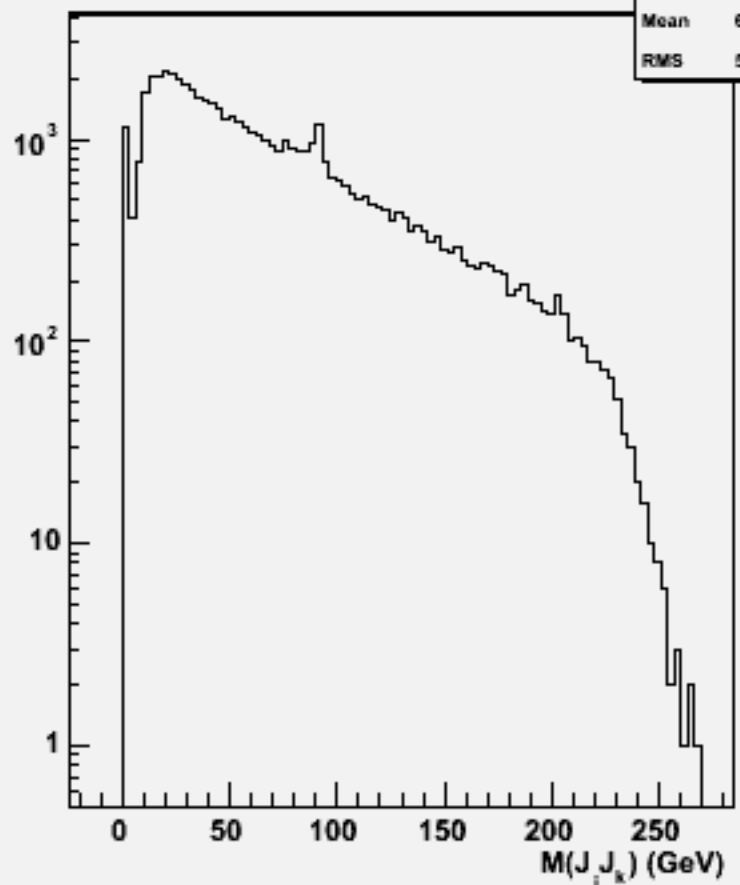
2jets mass(All comb)w102992 e1a_n1uue1n1_o
