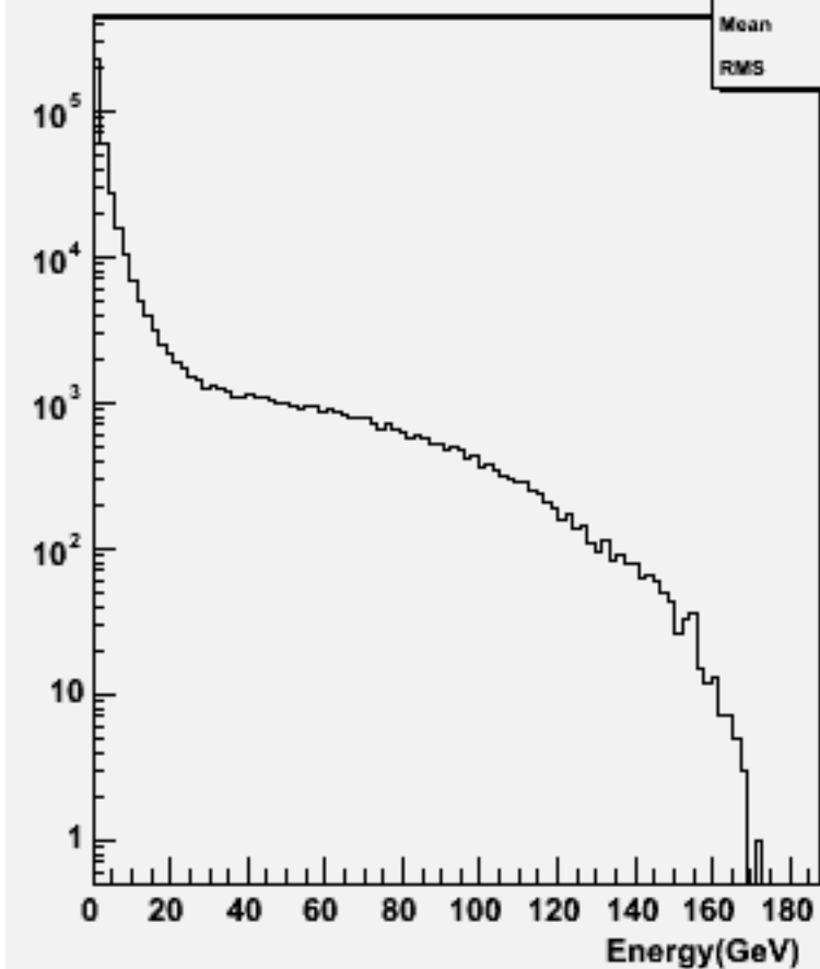
Particle Energy : w102990 e1a_n1uue1n1_o
