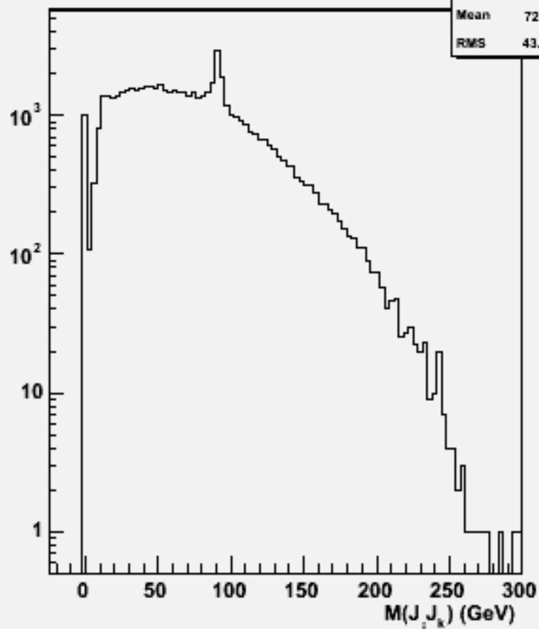
2jets mass(All comb)w102990 e1a_n1uue1n1_o
