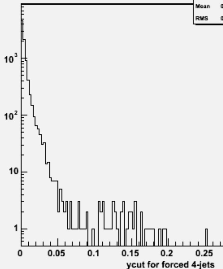
Ycut for 4-jets :w102986 e1a_n1n3n3sc_o
