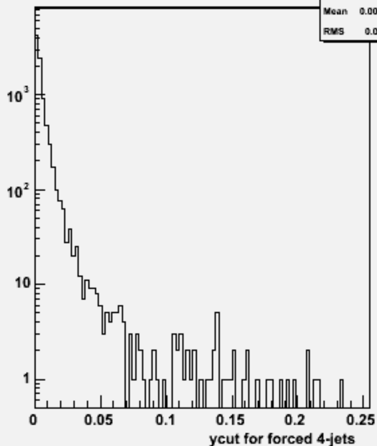
Ycut for 4-jets :w102982 e1a_n1n3n3du_o
