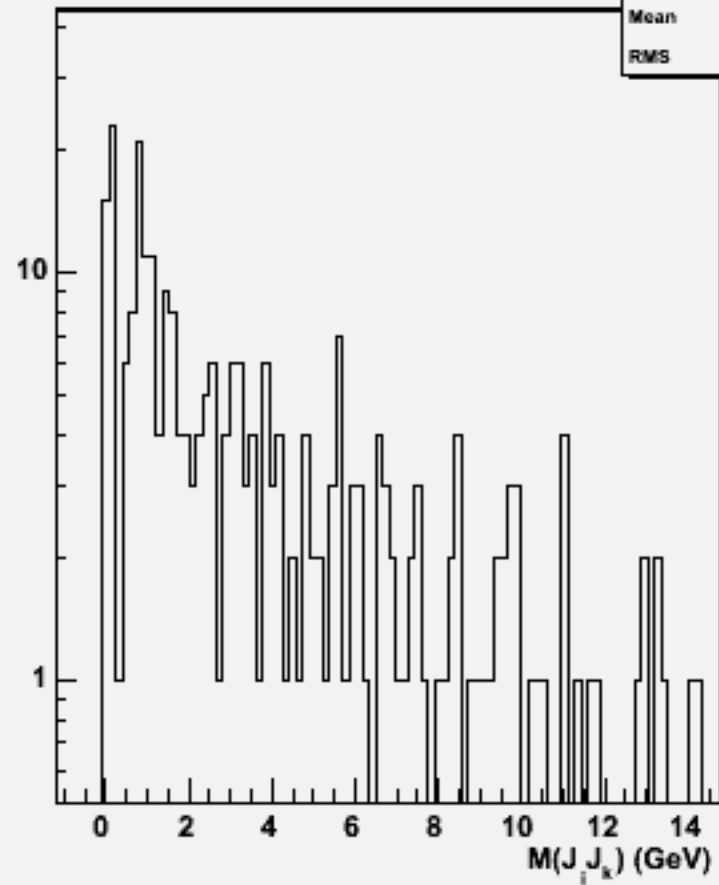
2jets mass(All comb)w102978 e1a_n1n3n3e3n3_o
