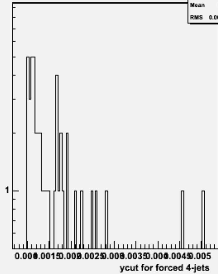
Ycut for 4-jets :w102978 e1a_n1n3n3e3n3_o
