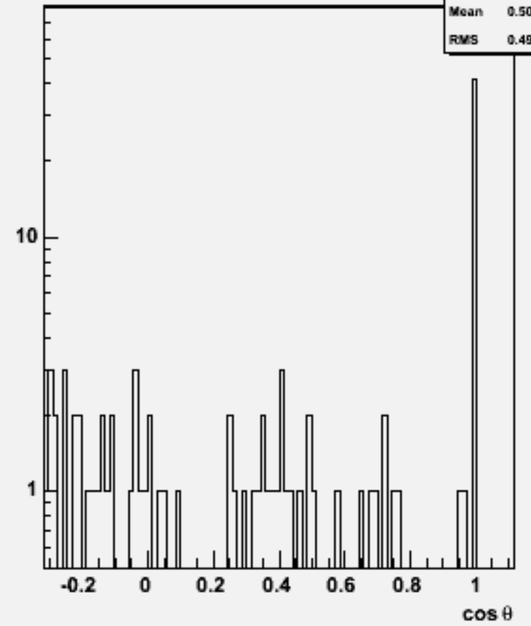
Jet cos \theta (All jets)w102978 e1a_n1n3n3e3n3_o
