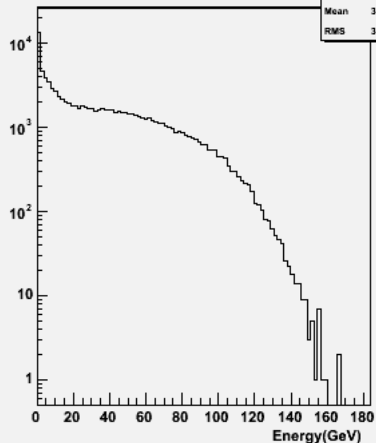
Particle Energy : w102938 e1a_n1n1n1e3n3_o
