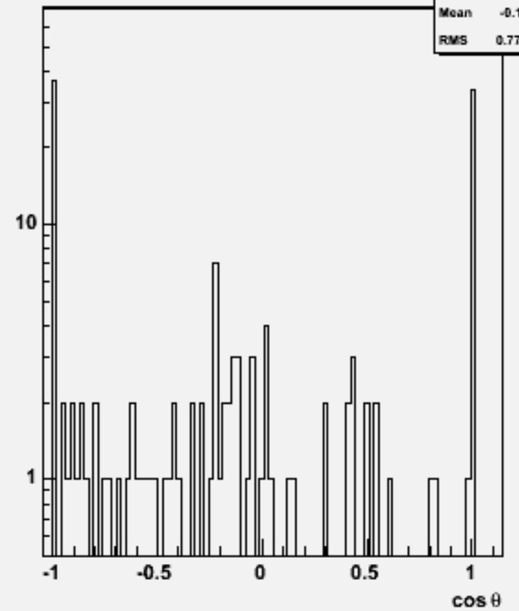
Jet cos \theta (All jets)w102938 e1a_n1n1n1e3n3_o
