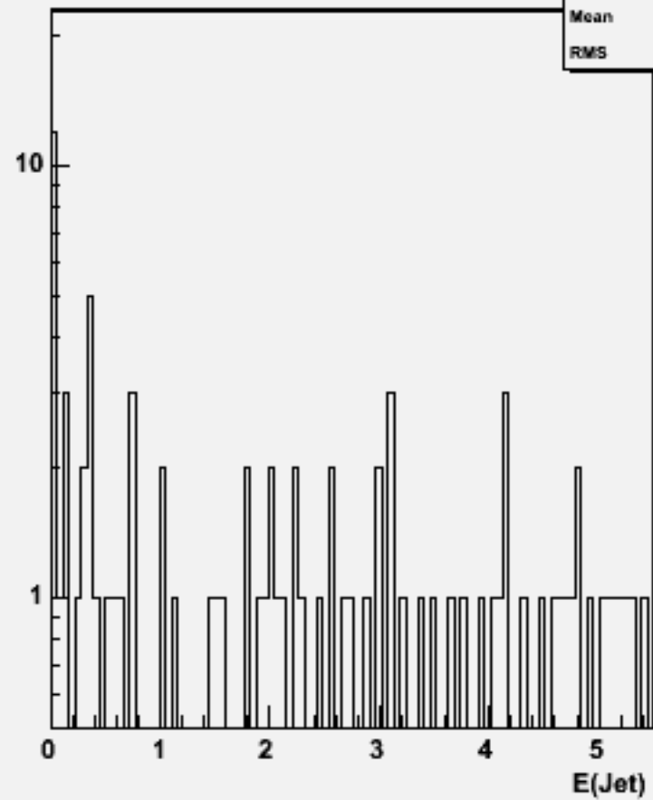
Jet energies(All jets)w102938 e1a_n1n1n1e3n3_o
