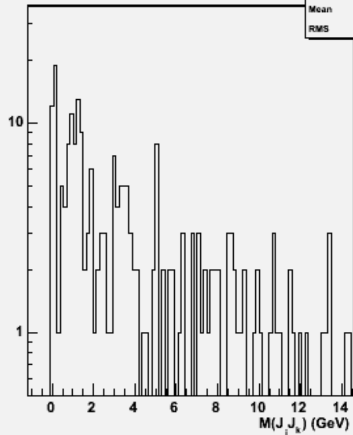
2jets mass(All comb)w102938 e1a_n1n1n1e3n3_o
