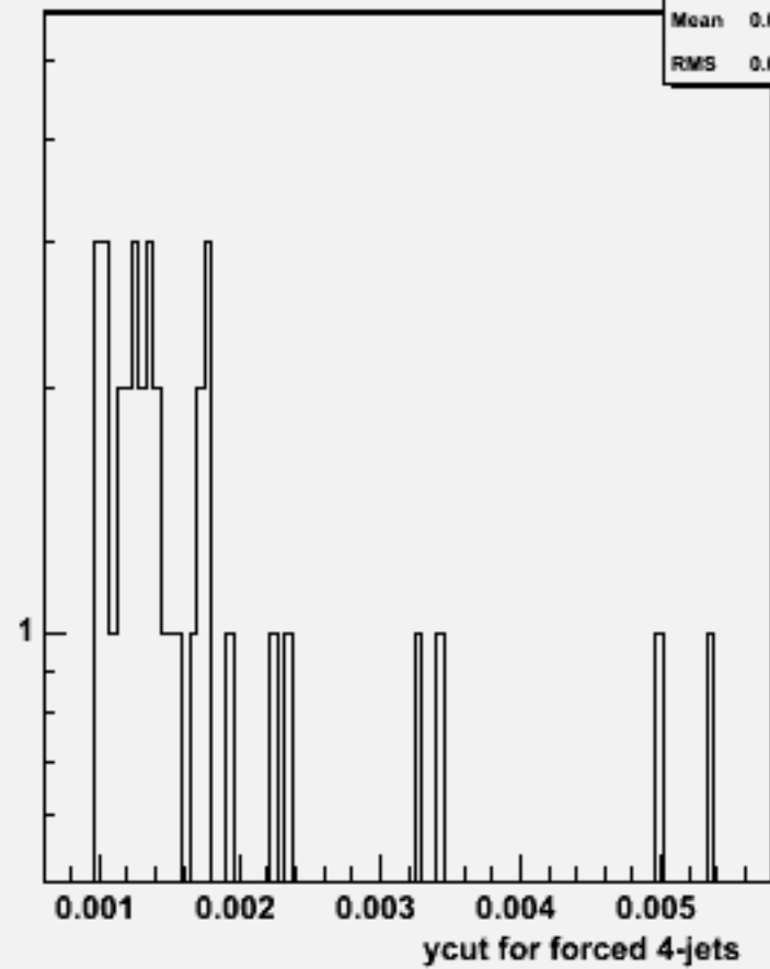
Ycut for 4-jets :w102938 e1a_n1n1n1e3n3_o
