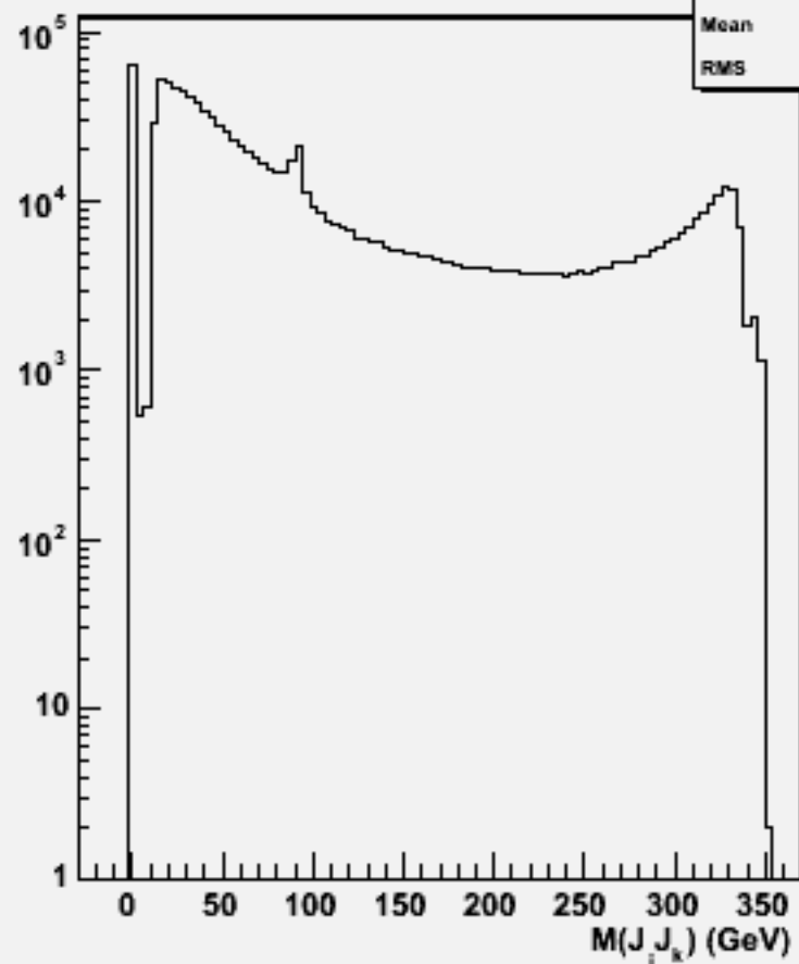
2jets mass(All comb)w102855 e1a_e1dd_o
