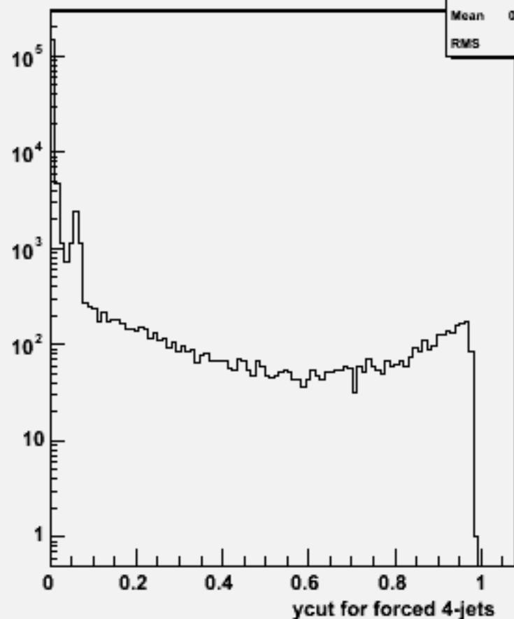
Ycut for 4-jets :w102855 e1a_e1dd_o
