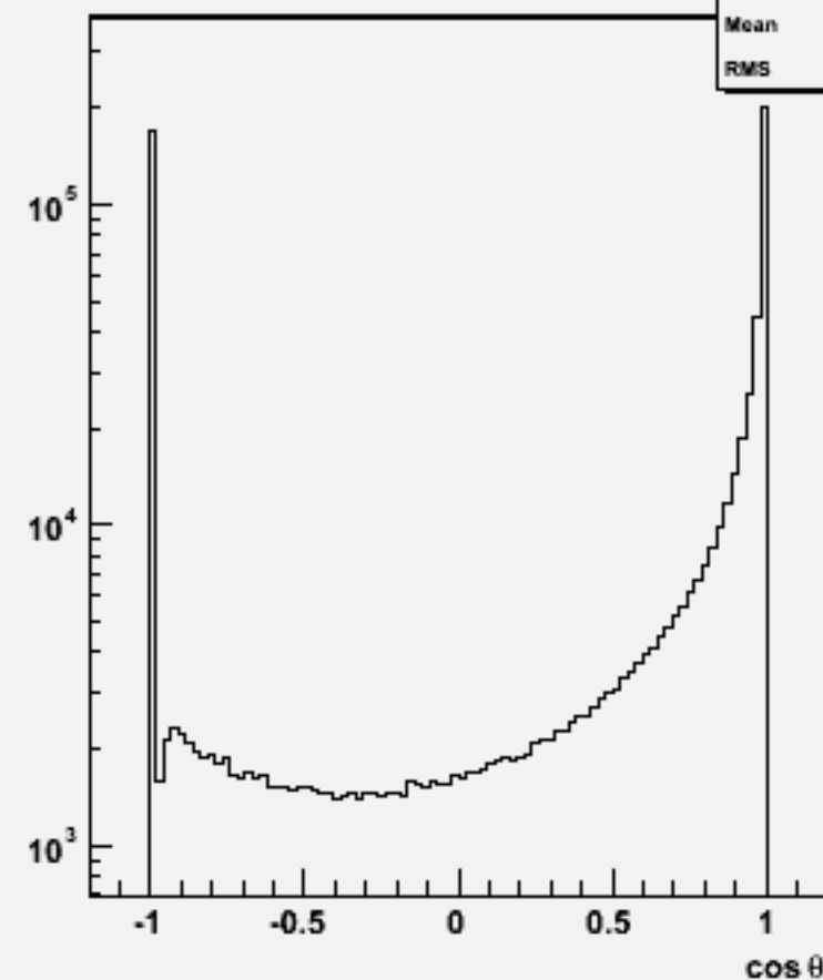
Jet cos \theta (All jets)w102855 e1a_e1dd_o
