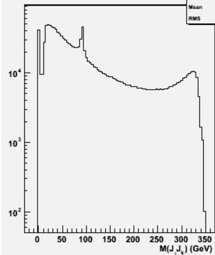
2jets mass(All comb)w102854 e1a_e1dd_o
