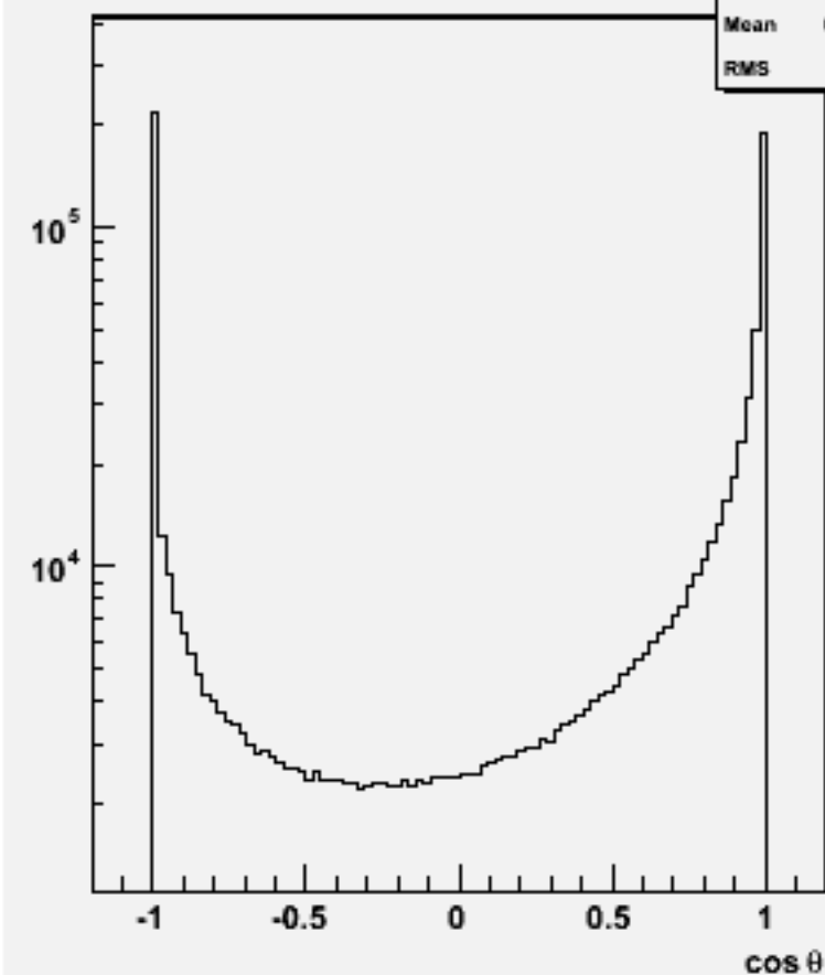
Jet cosθ (All jets)w102854 e1a_e1dd_o
