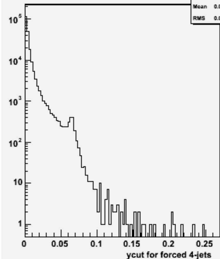
Ycut for 4-jets :w102854 e1a_e1dd_o
