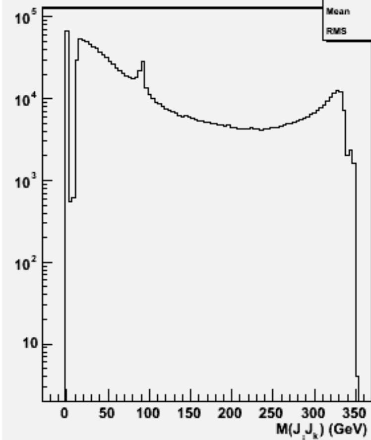
2jets mass(All comb)w102853 e1a_e1dd_o
