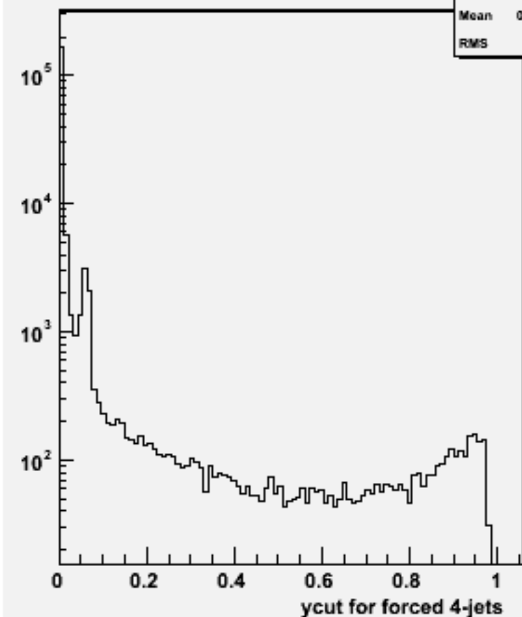
Ycut for 4-jets :w102853 e1a_e1dd_o
