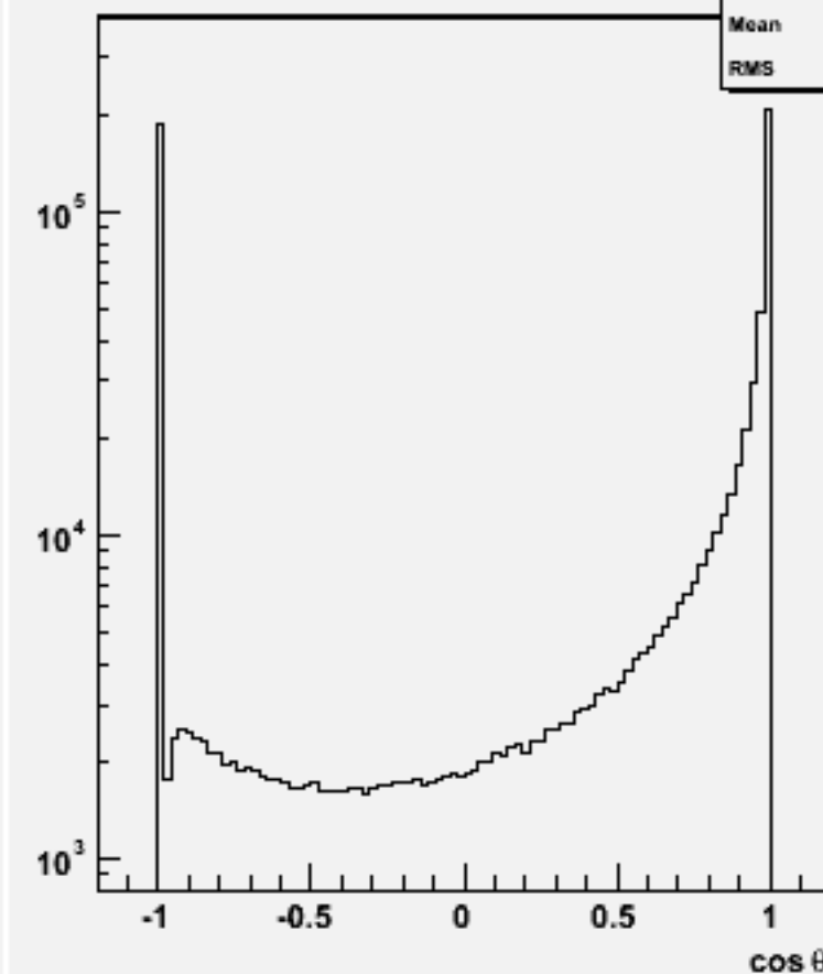
Jet cosθ (All jets)w102853 e1a_e1dd_o
