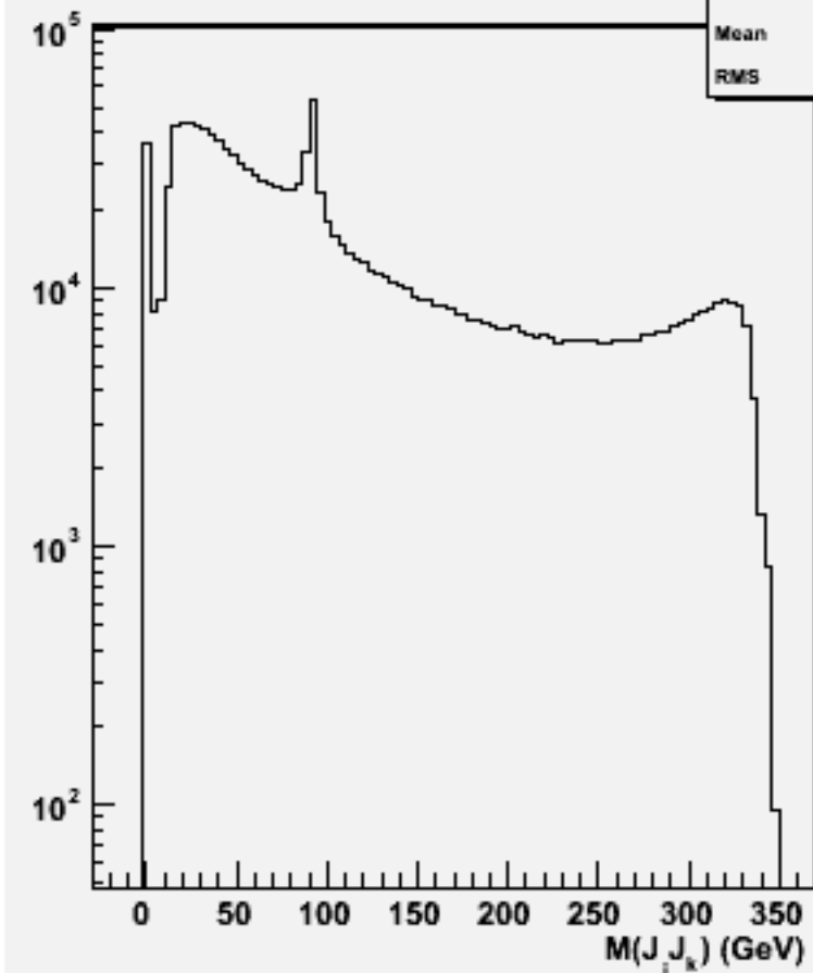
2jets mass(All comb)w102852 e1a_e1dd_o
