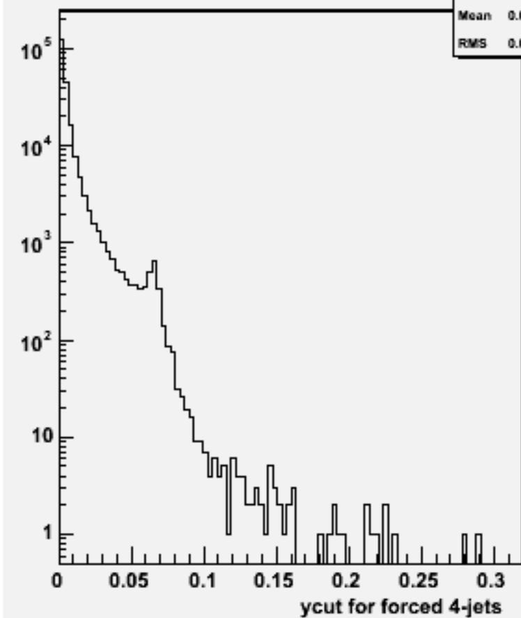
Ycut for 4-jets :w102852 e1a_e1dd_o
