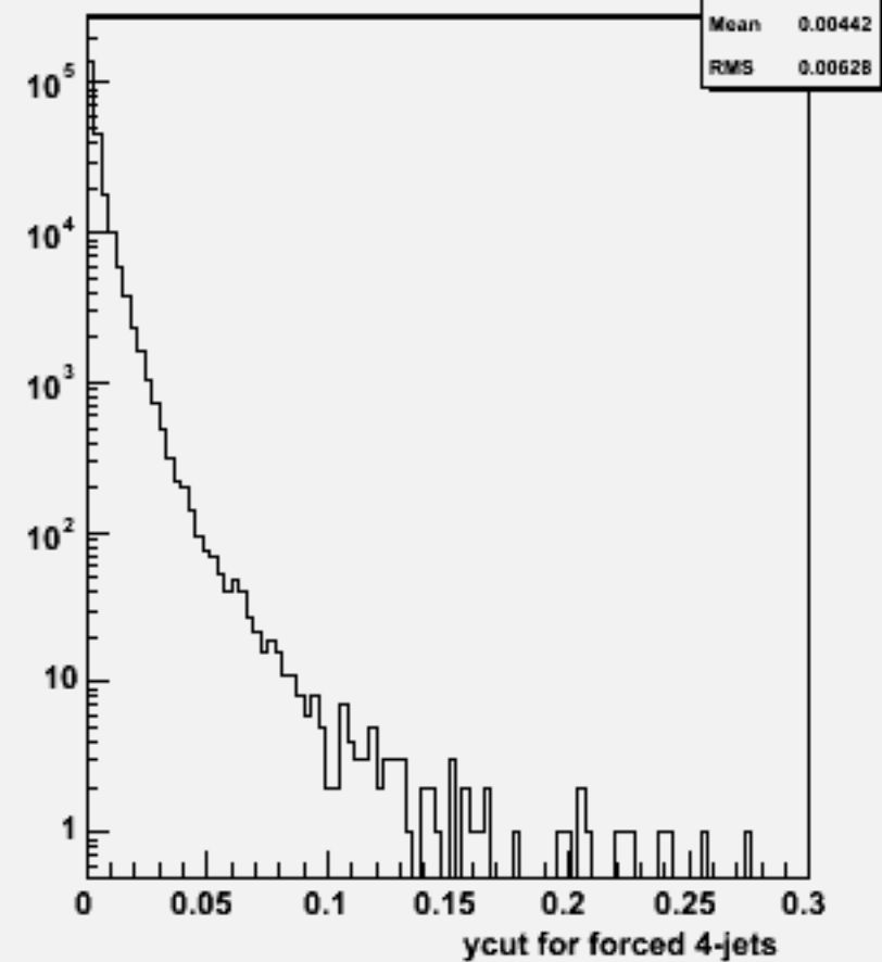
Ycut for 4-jets :w102850 e1a_e1e3e3_o
