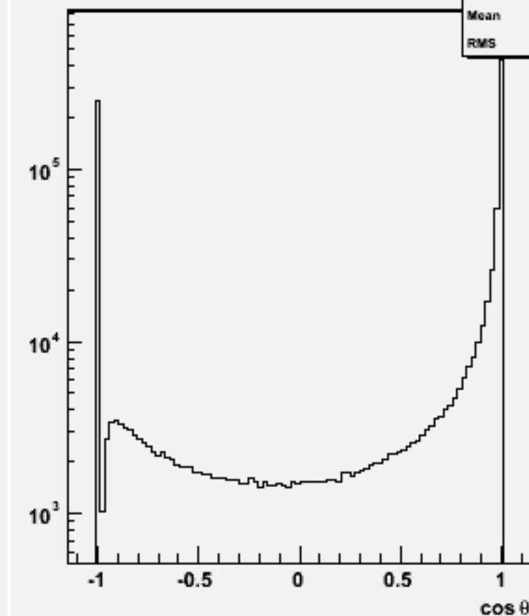
Jet cos \theta (All jets)w102849 e1a_e1e3e3_o
