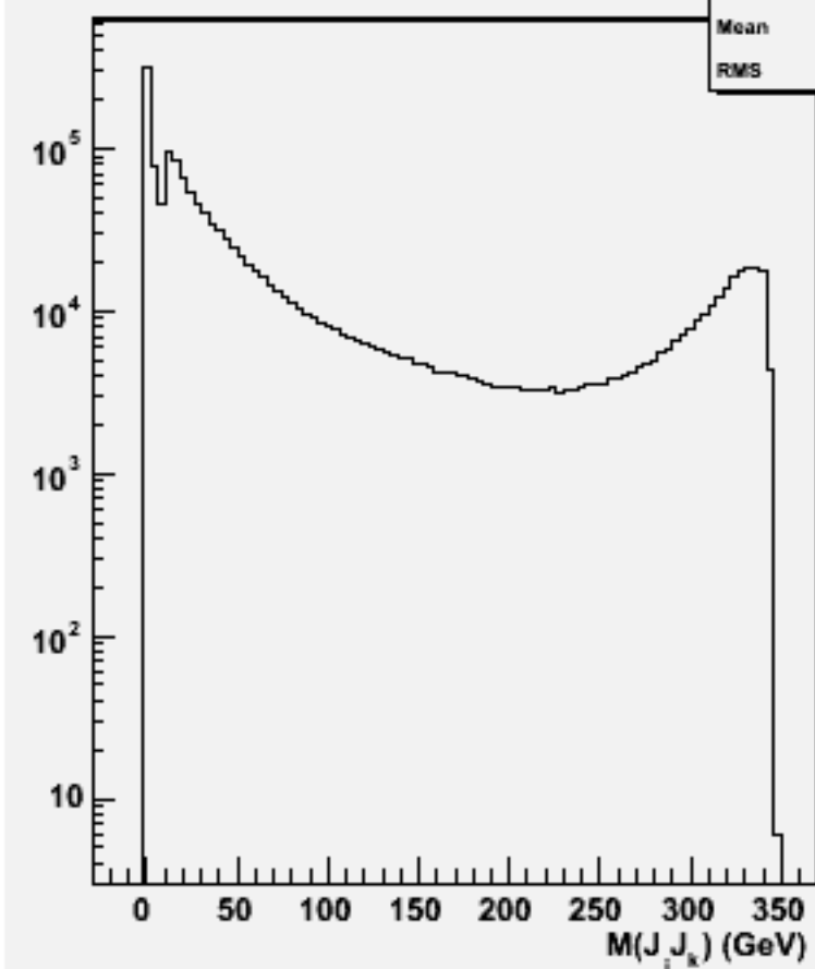
2jets mass(All comb)w102849 e1a_e1e3e3_o
