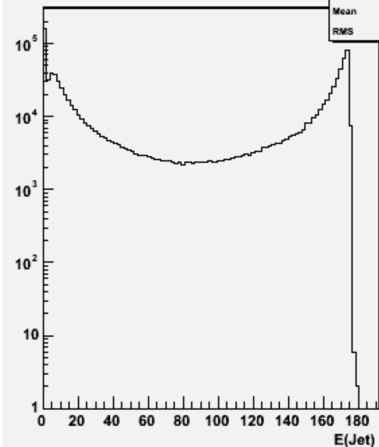
Jet energies(All jets)w102849 e1a_e1e3e3_o
