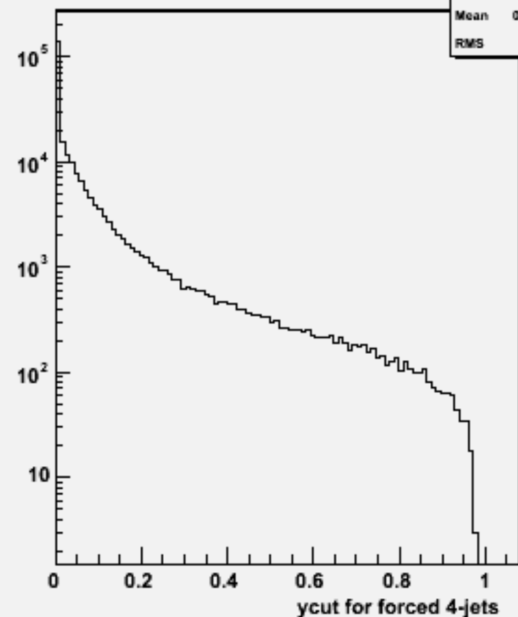
Ycut for 4-jets :w102849 e1a_e1e3e3_o
