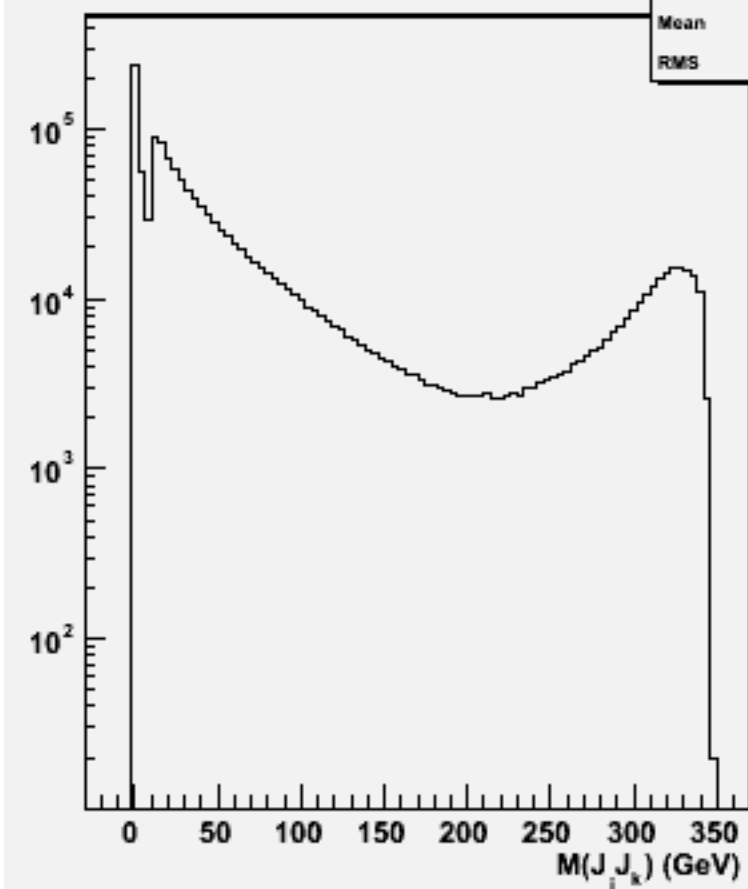
2jets mass(All comb)w102848 e1a_e1e3e3_o
