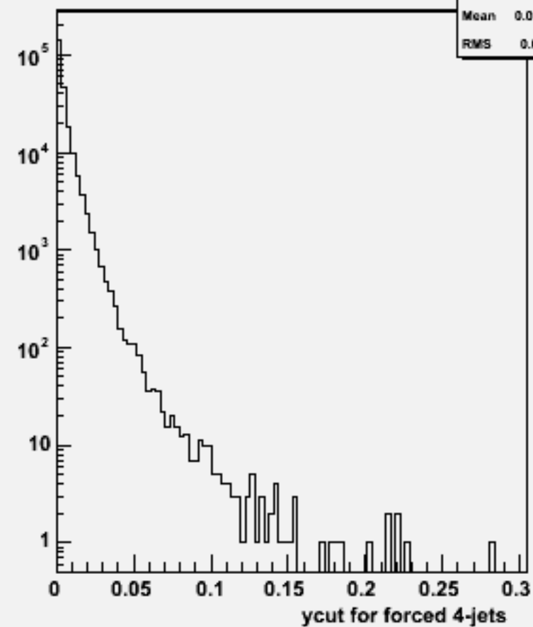
Ycut for 4-jets :w102848 e1a_e1e3e3_o
