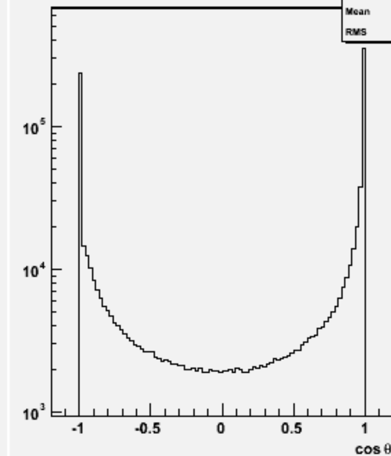
Jet cos \theta (All jets)w102848 e1a_e1e3e3_o
