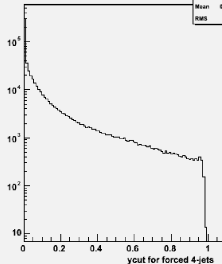
Ycut for 4-jets :w102845 e1a_e1e2e2_o
