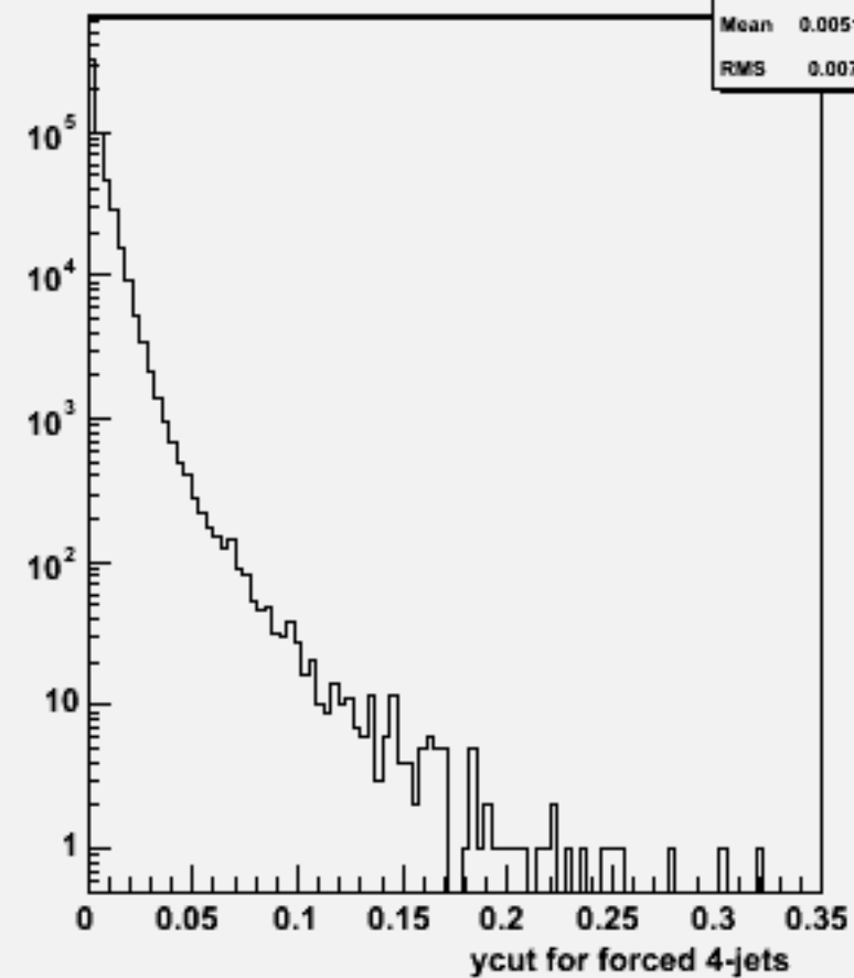
Ycut for 4-jets :w102844 e1a_e1e2e2_o
