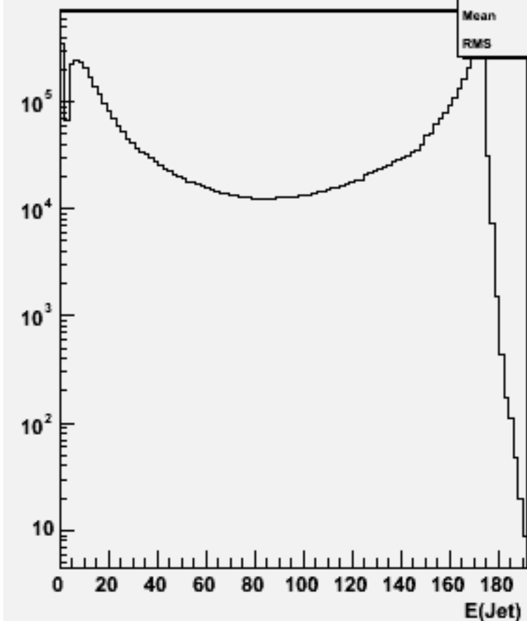
Jet energies(All jets)w102843 e1a_e1e1e1_o
