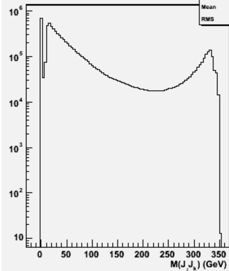
2jets mass(All comb)w102843 e1a_e1e1e1_o
