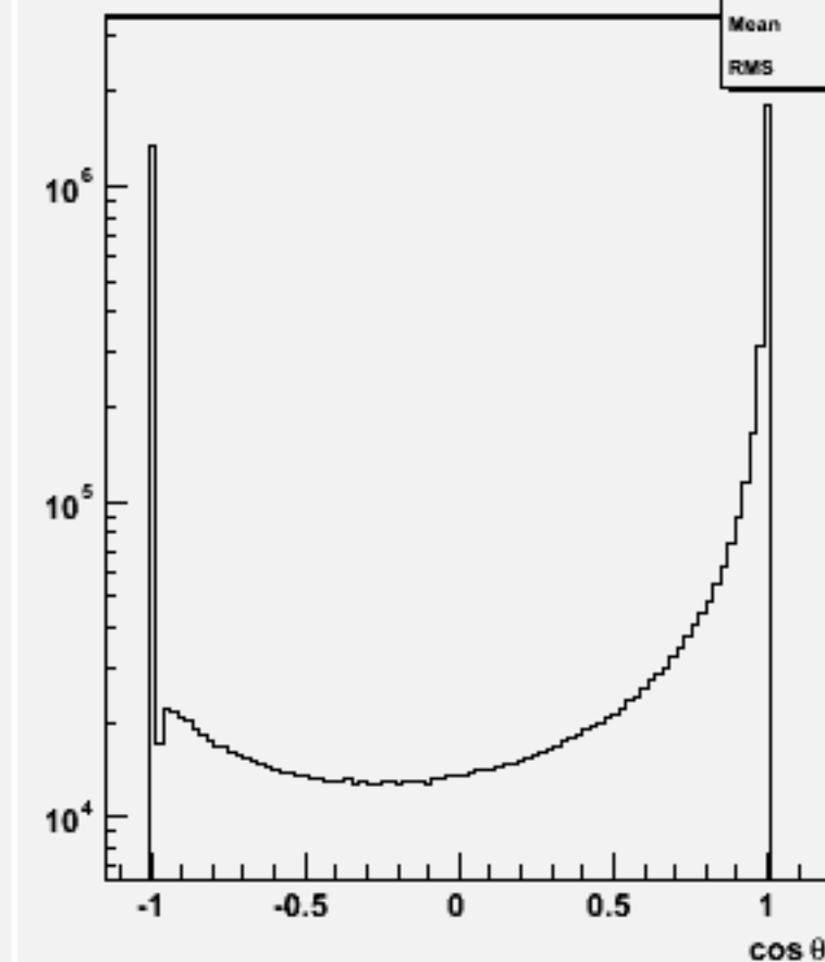
Jet cos \theta (All jets)w102843 e1a_e1e1e1_o
