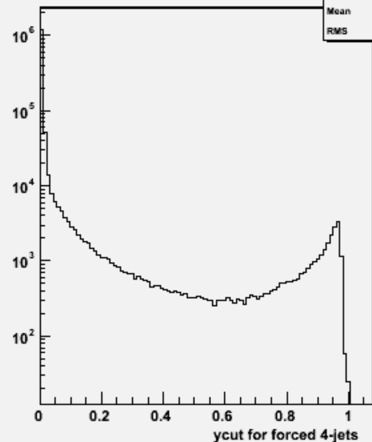
Ycut for 4-jets :w102843 e1a_e1e1e1_o
