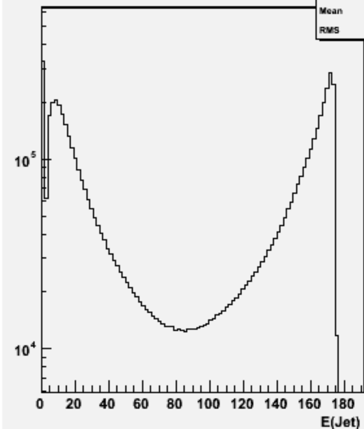
Jet energies(All jets)w102840 e1a_e1e1e1_o
