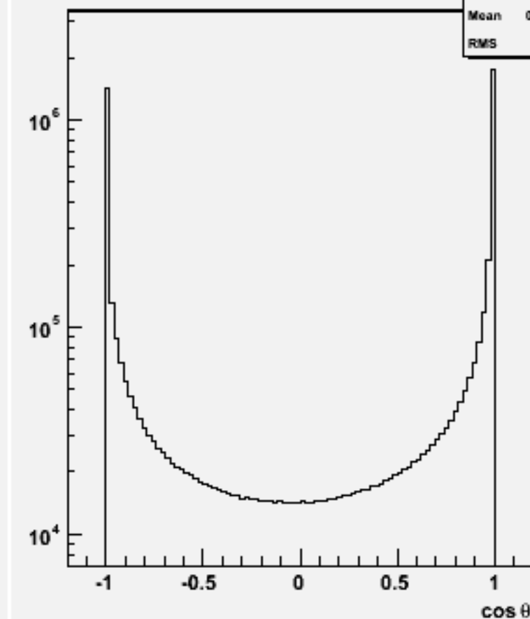
Jet cos \theta (All jets)w102840 e1a_e1e1e1_o
