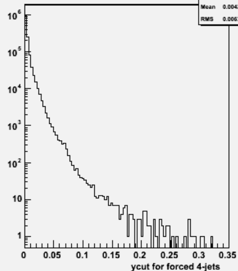
Ycut for 4-jets :w102840 e1a_e1e1e1_o
