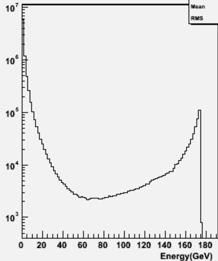
Particle Energy : w102839 e1a_e1cc_o
