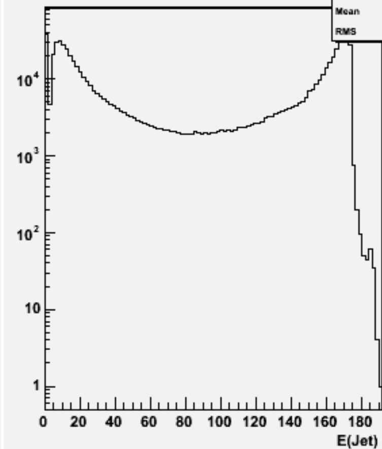
Jet energies(All jets)w102839 e1a_e1cc_o
