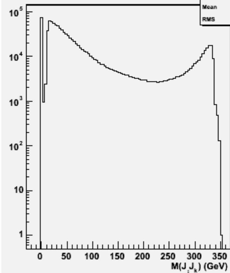
2jets mass(All comb)w102839 e1a_e1cc_o
