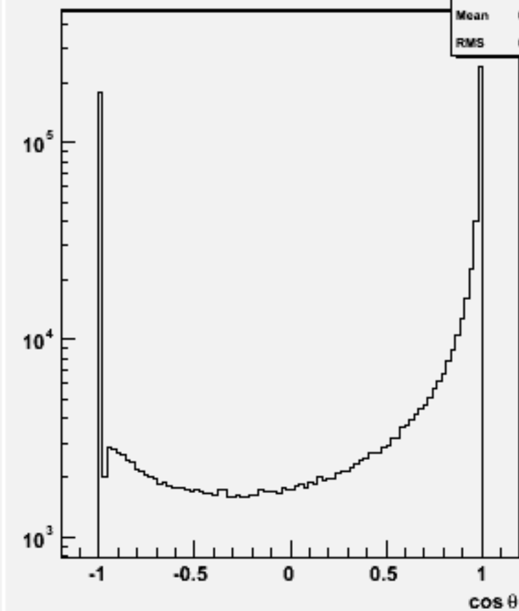
Jet cosθ (All jets)w102839 e1a_e1cc_o
