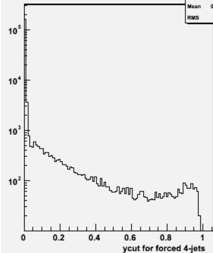
Ycut for 4-jets :w102839 e1a_e1cc_o
