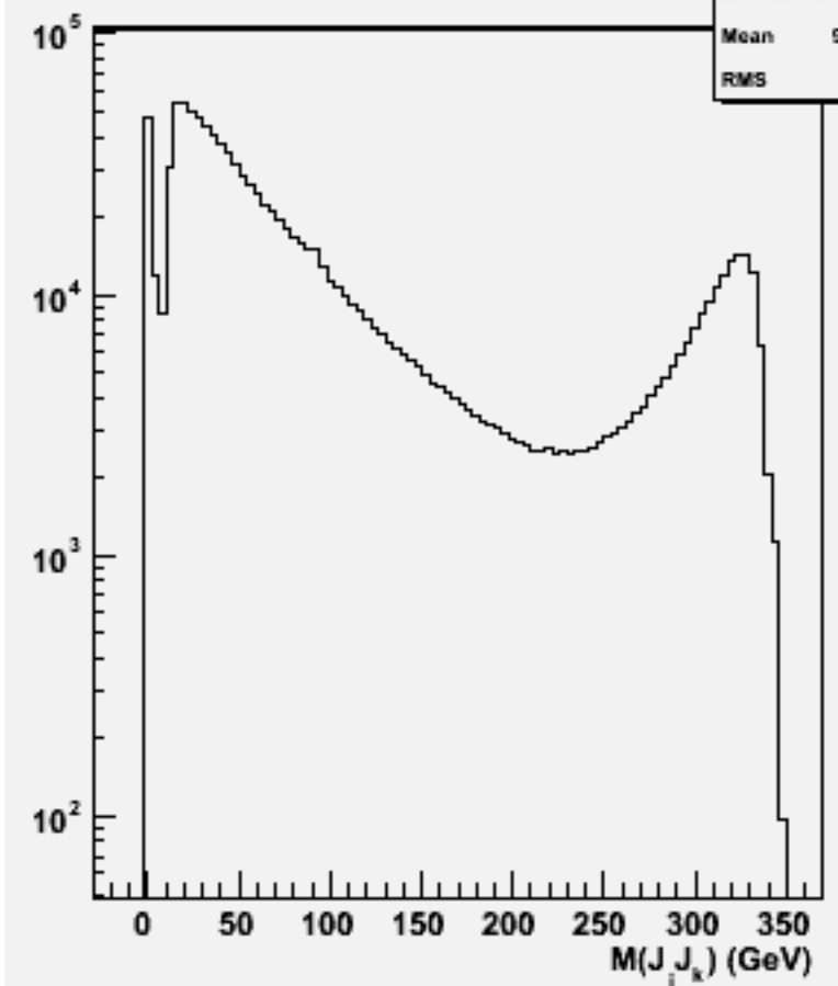
2jets mass(All comb)w102838 e1a_e1cc_o
