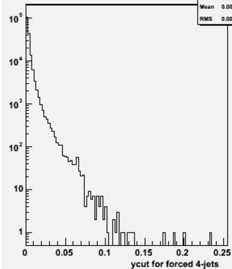
Ycut for 4-jets :w102838 e1a_e1cc_o
