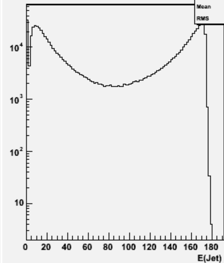
Jet energies(All jets)w102838 e1a_e1cc_o
