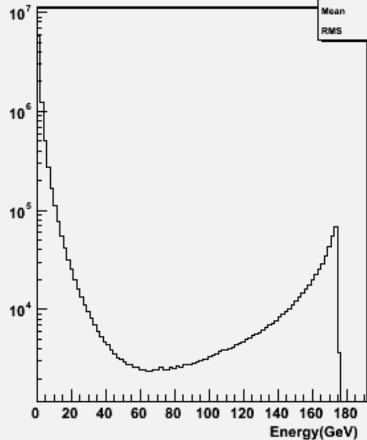
Particle Energy : w102838 e1a_e1cc_o
