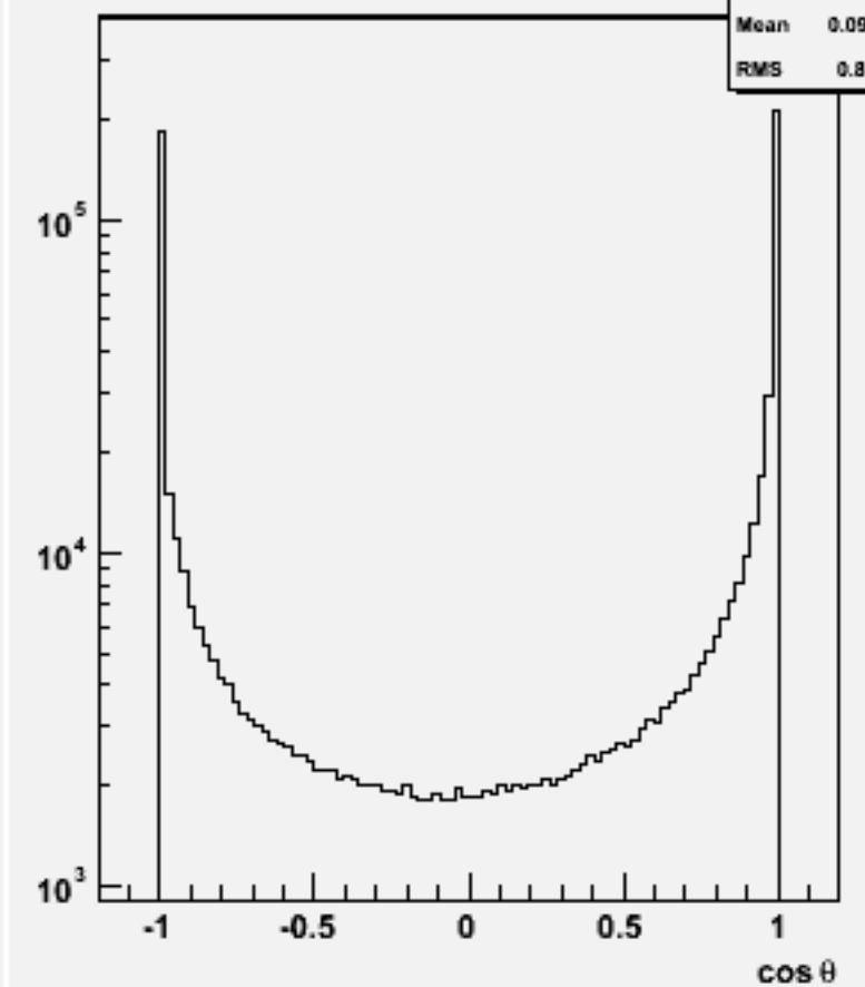
Jet cosθ (All jets)w102838 e1a_e1cc_o
