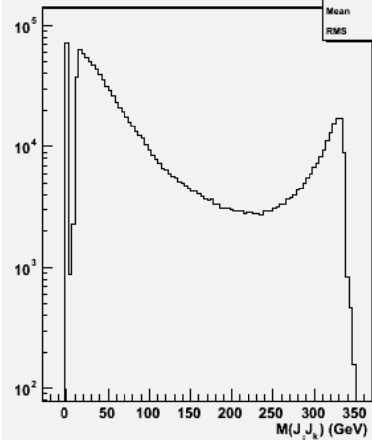
2jets mass(All comb)w102837 e1a_e1cc_o
