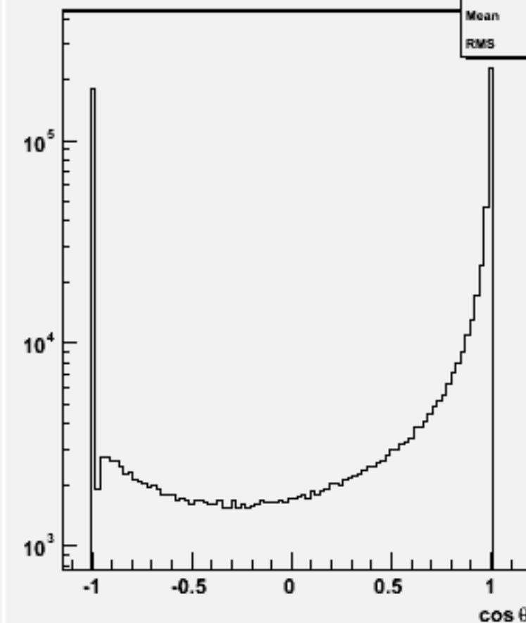
Jet cosθ (All jets)w102837 e1a_e1cc_o
