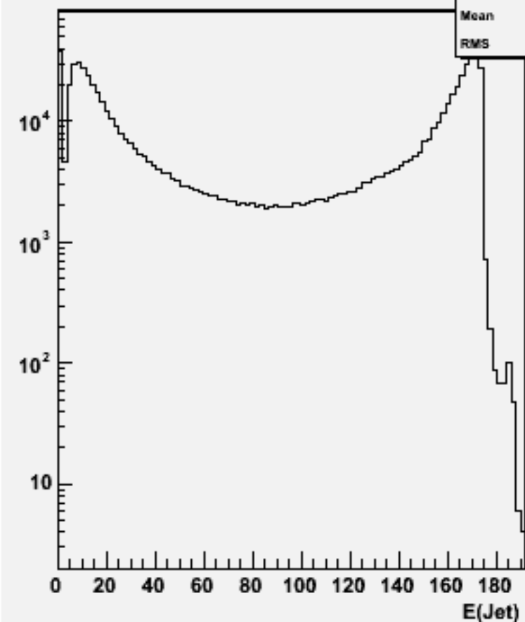
Jet energies(All jets)w102837 e1a_e1cc_o
