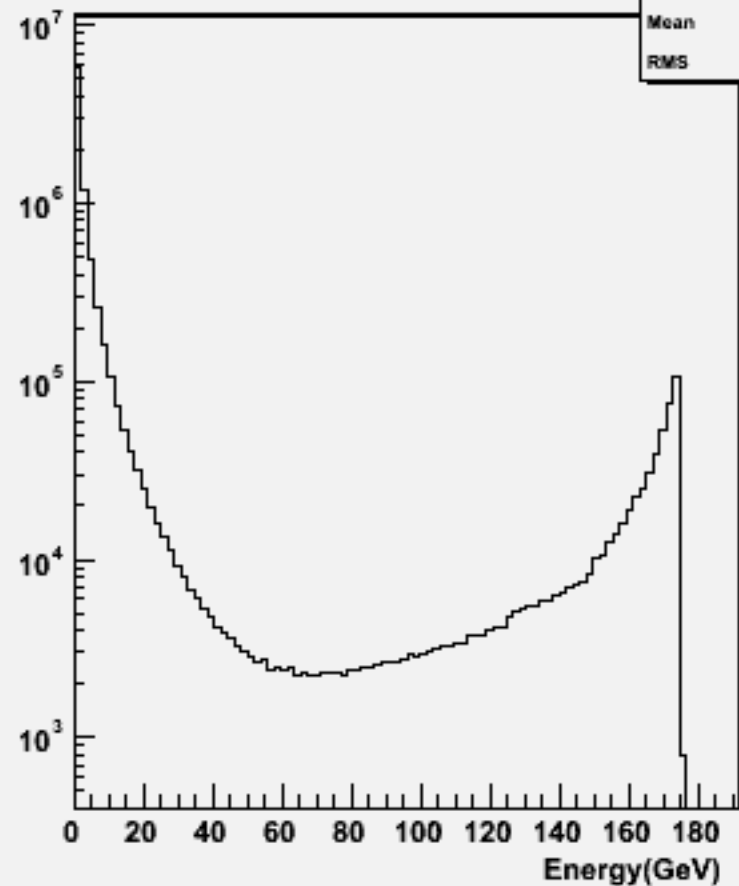
Particle Energy : w102837 e1a_e1cc_o
