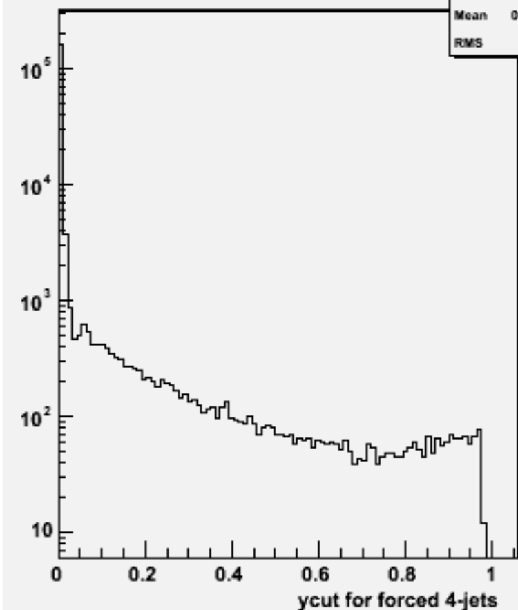
Ycut for 4-jets :w102837 e1a_e1cc_o
