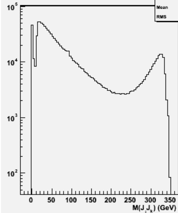
2jets mass(All comb)w102836 e1a_e1cc_o
