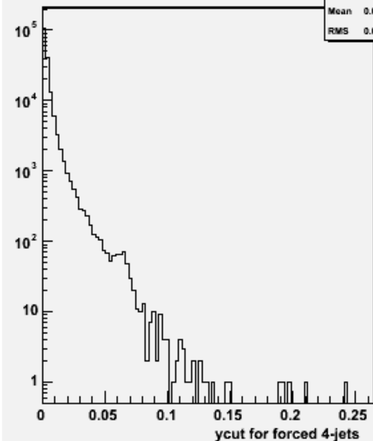
Ycut for 4-jets :w102836 e1a_e1cc_o
