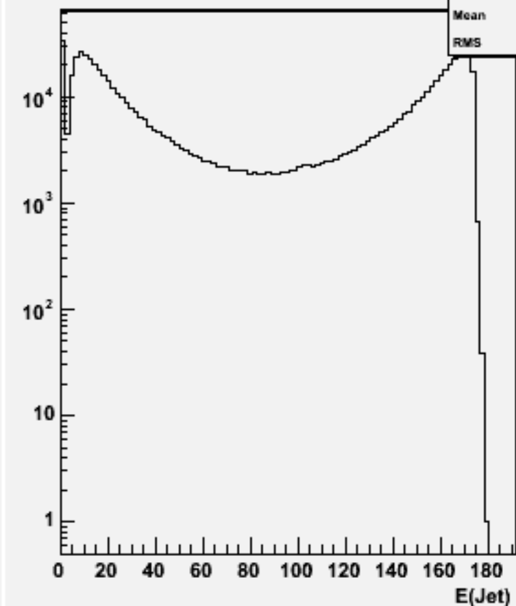
Jet energies(All jets)w102836 e1a_e1cc_o
