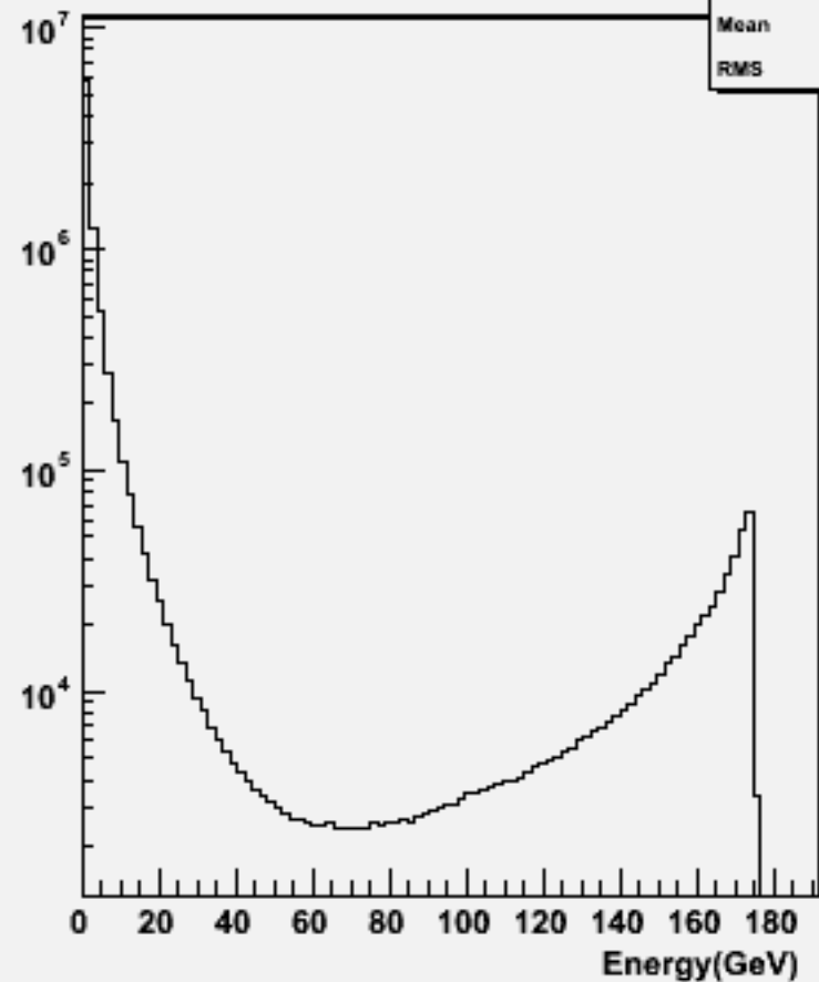
Particle Energy : w102836 e1a_e1cc_o
