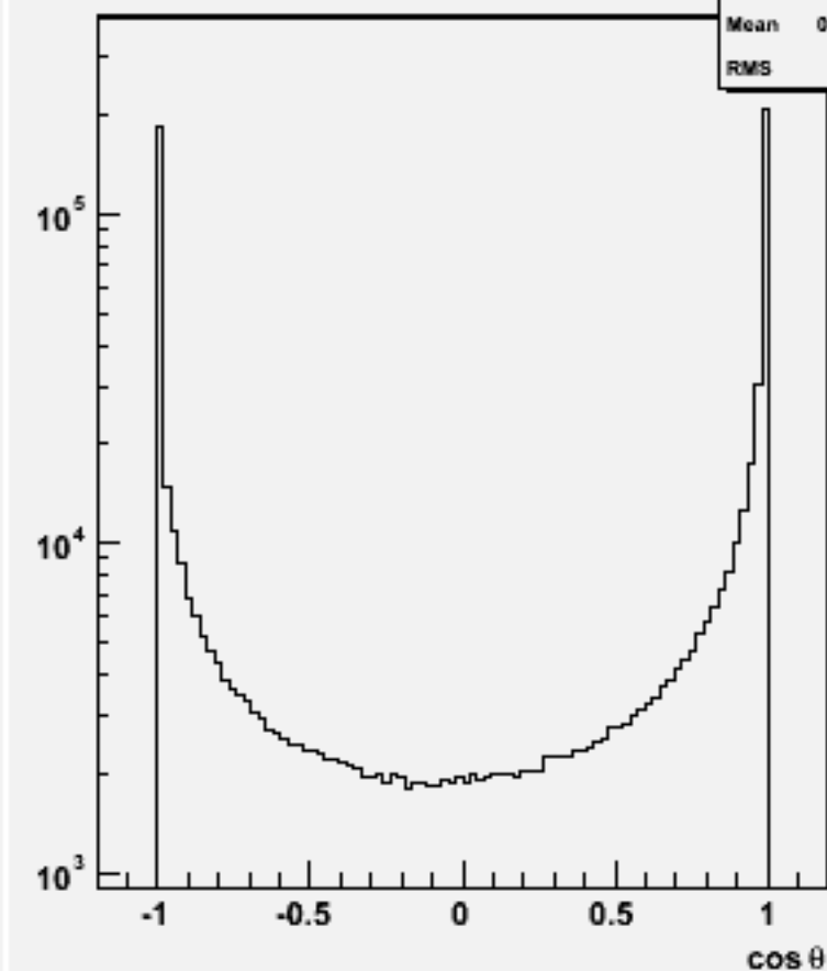
Jet cosθ (All jets)w102836 e1a_e1cc_o
