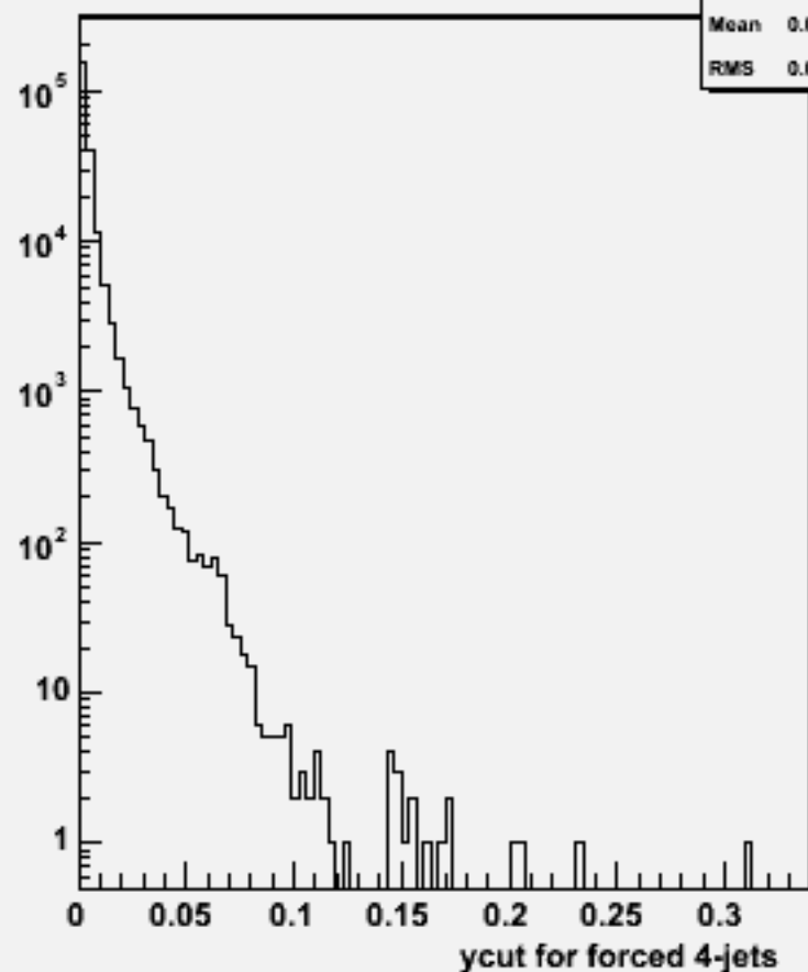
Ycut for 4-jets :w102834 e1a_e1uu_o
