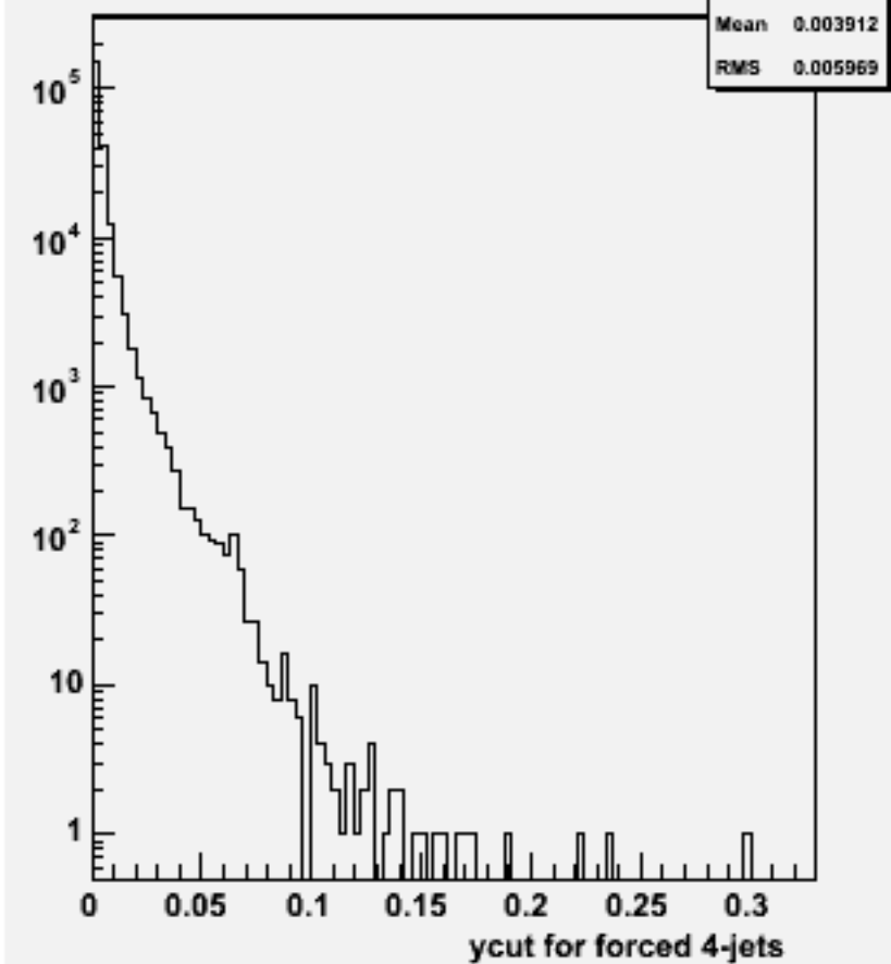
Ycut for 4-jets :w102832 e1a_e1uu_o
