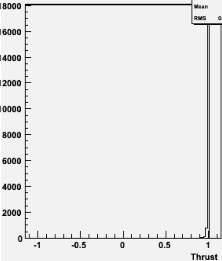
cos \Theta (thrust) w102831 e1a_e1n3n3_o
