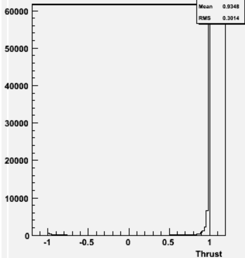
cos \Theta (thrust) w102828 e1a_e1n3n3_o
