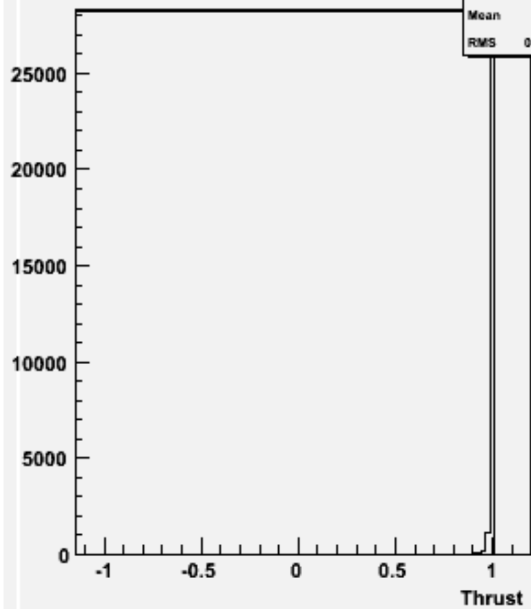
cos \Theta (thrust) w102825 e1a_e1n2n2_o
