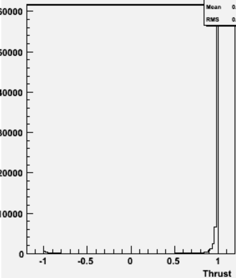
cos \Theta (thrust) w102824 e1a_e1n2n2_o
