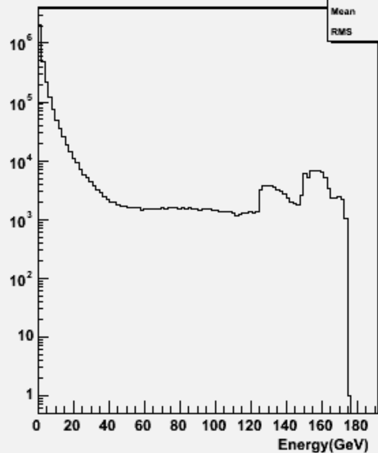
Particle Energy : w102821 e1a_n1sc_o
