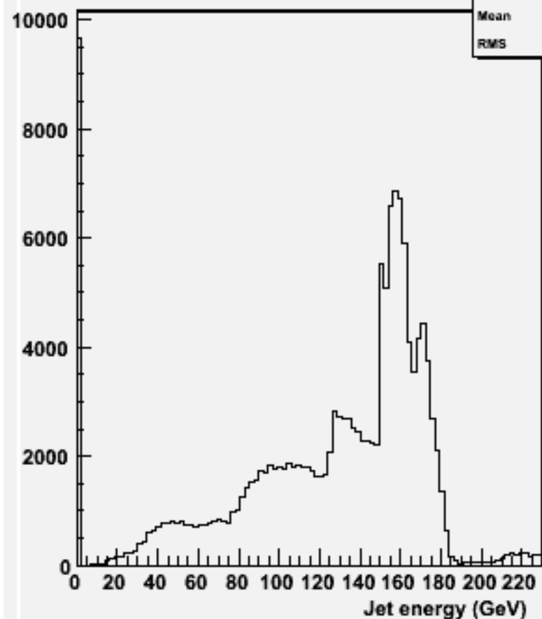
energy for 2-jets :w102821 e1a_n1sc_o
