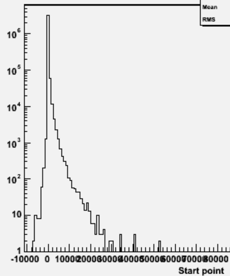
Start point Z : w102821 e1a_n1sc_o
