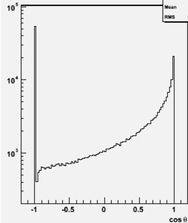
Jet cosθ (All jets)w102821 e1a_n1sc_o
