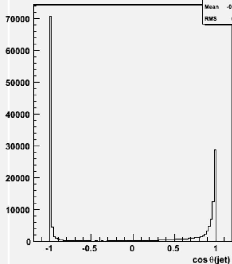
cos \theta for 2-jets :w102821 e1a_n1sc_o
