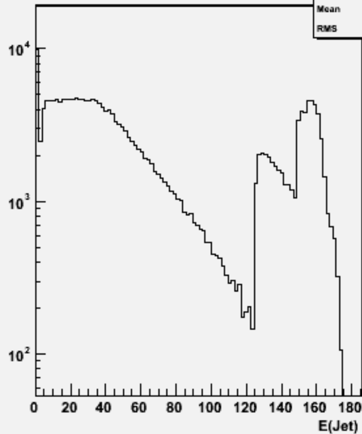
Jet energies(All jets)w102821 e1a_n1sc_o
