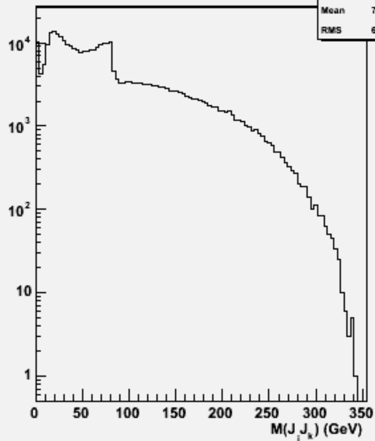
2jets mass(All comb)w102821 e1a_n1sc_o
