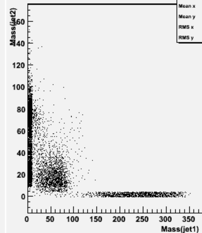
Jet mass for forced 2-jets : w102821 e1a_n1sc_o
