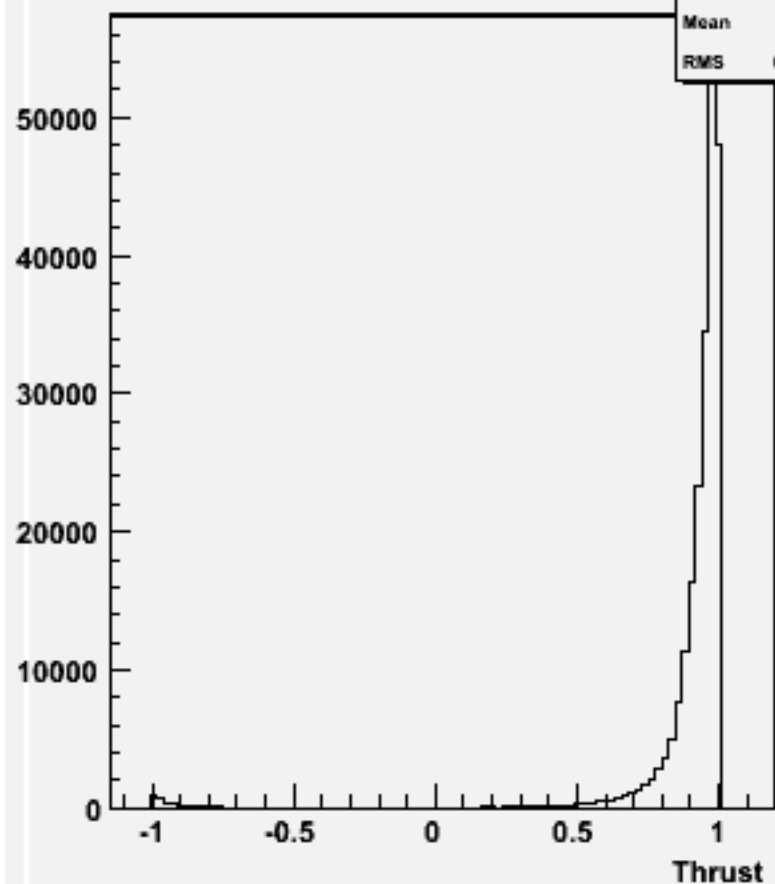
cos \Theta (thrust) w102820 e1a_n1sc_o
