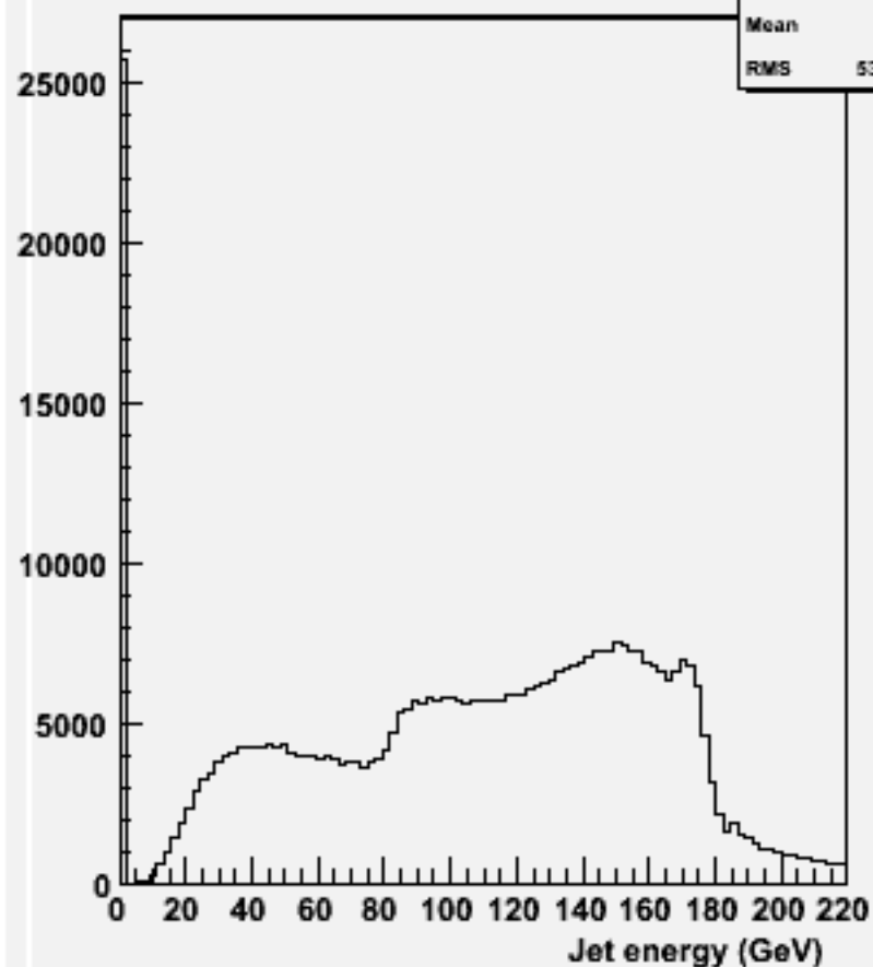
energy for 2-jets :w102820 e1a_n1sc_o
