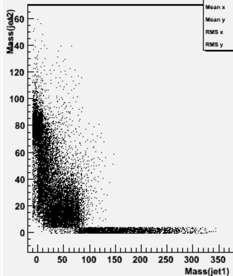
Jet mass for forced 2-jets : w102820 e1a_n1sc_o
