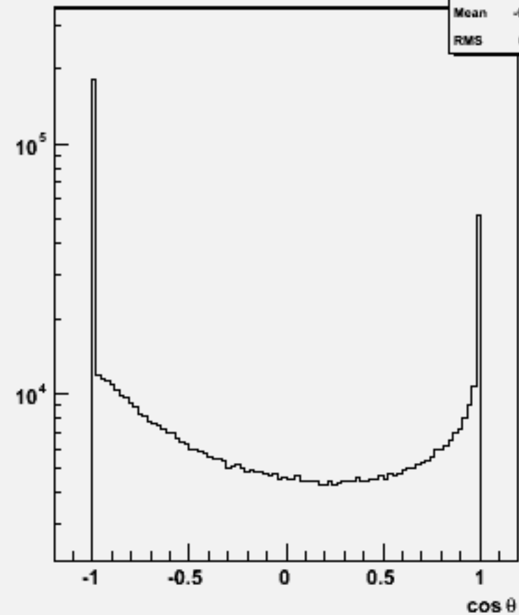
Jet cos \theta (All jets)w102820 e1a_n1sc_o
