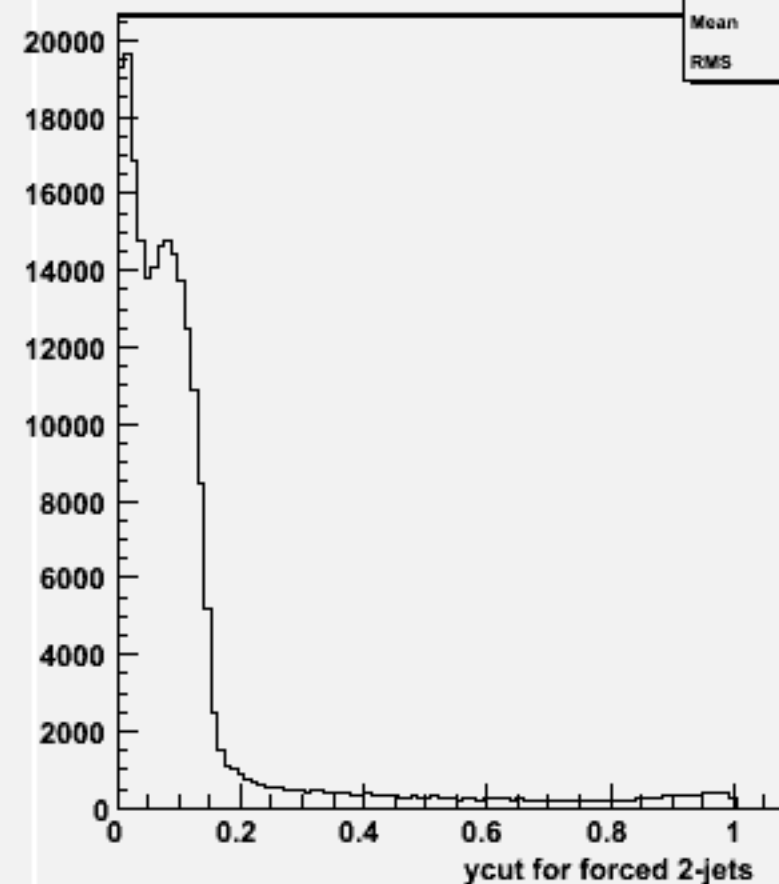
Ycut for 2-jets :w102820 e1a_n1sc_o
