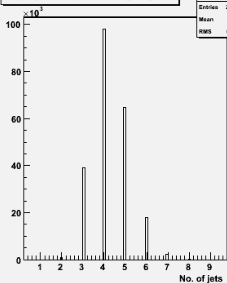
No. jets (ycut=0.001) : w102820 e1a_n1sc_o
