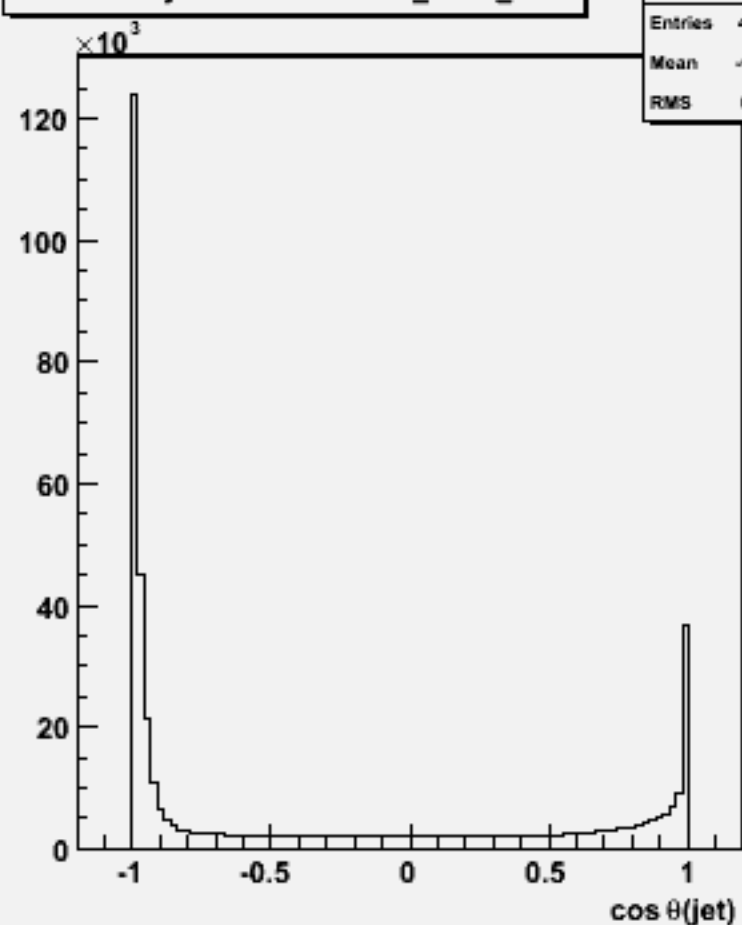
cos \theta for 2-jets :w102820 e1a_n1sc_o
