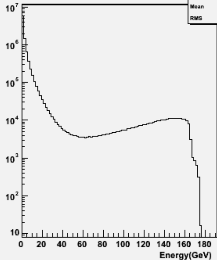
Particle Energy : w102820 e1a_n1sc_o
