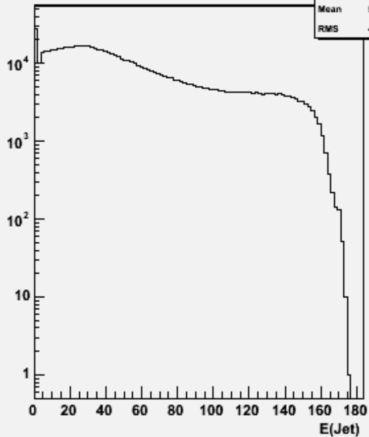
Jet energies(All jets)w102820 e1a_n1sc_o
