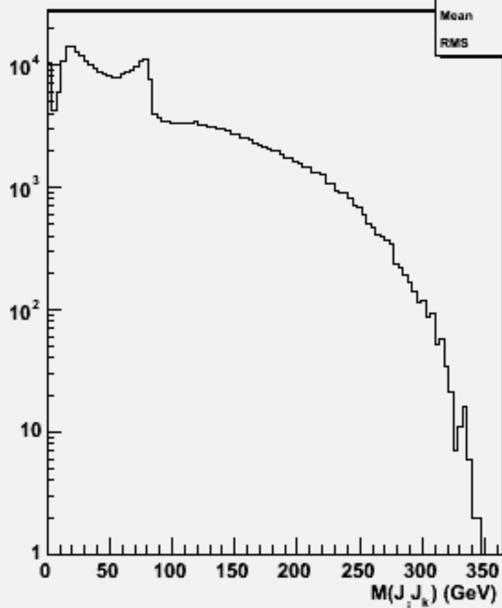
2jets mass(All comb)w102817 e1a_n1du_o
