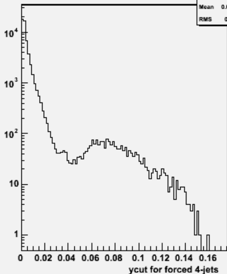
Ycut for 4-jets :w102817 e1a_n1du_o
