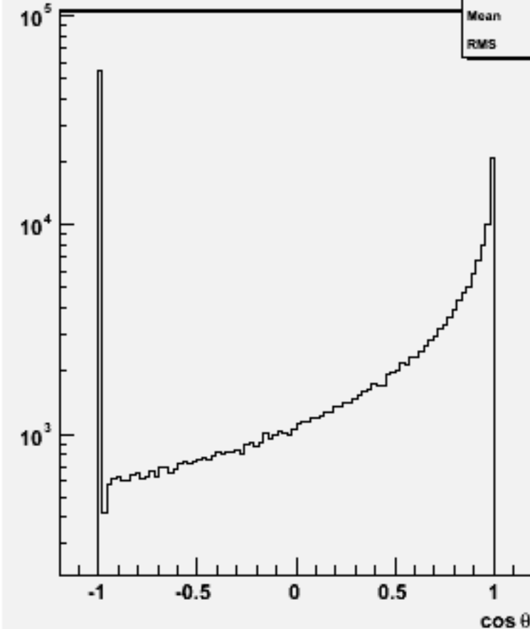
Jet cos \theta (All jets)w102817 e1a_n1du_o
