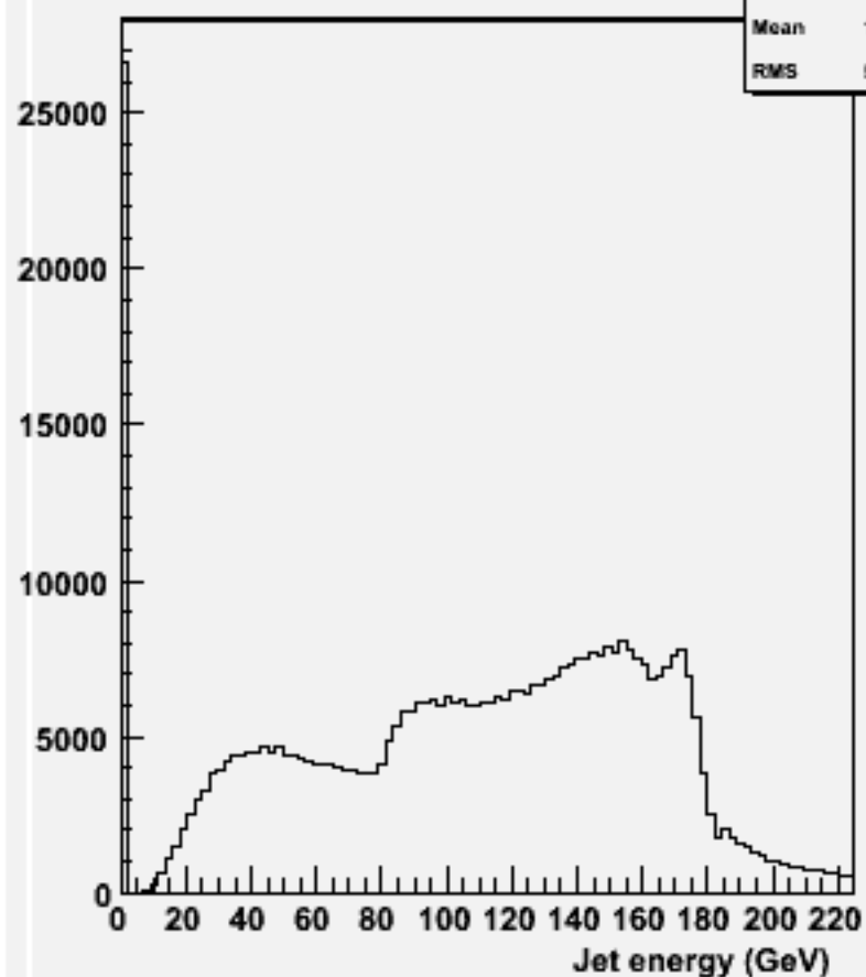
energy for 2-jets :w102816 e1a_n1du_o
