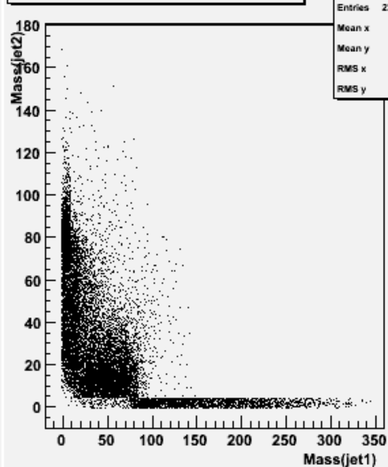
Jet mass for forced 2-jets : w102816 e1a_n1du_o
