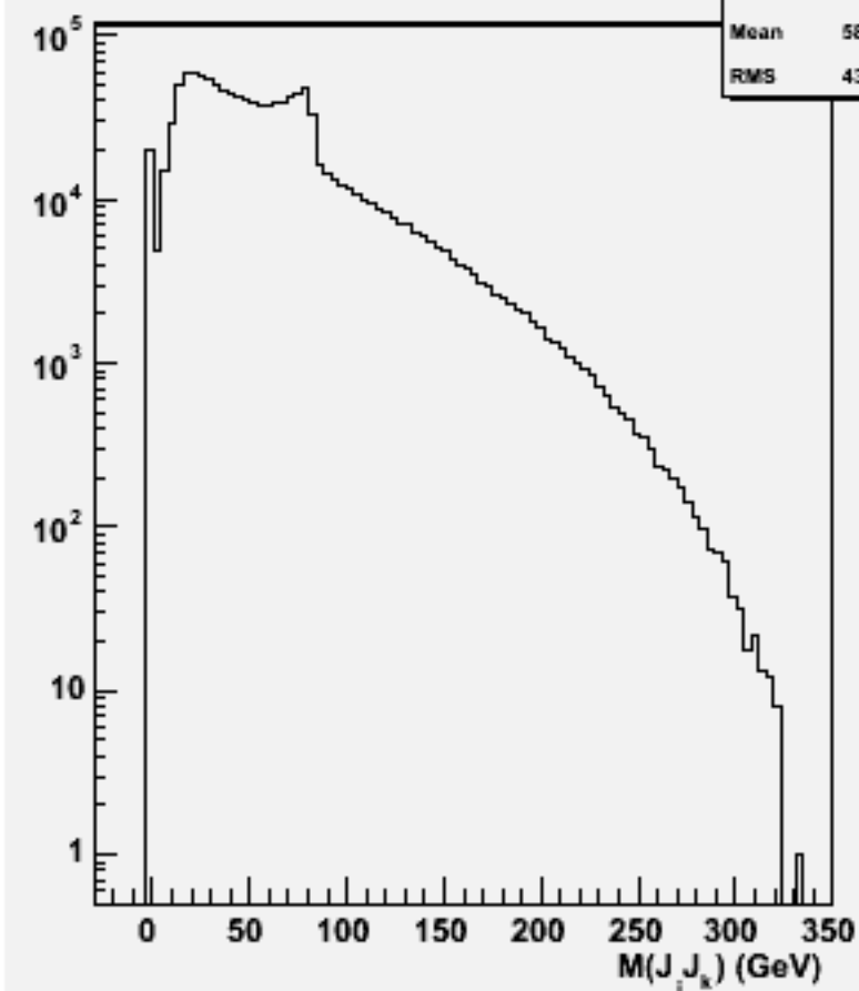
2jets mass(All comb)w102816 e1a_n1du_o
