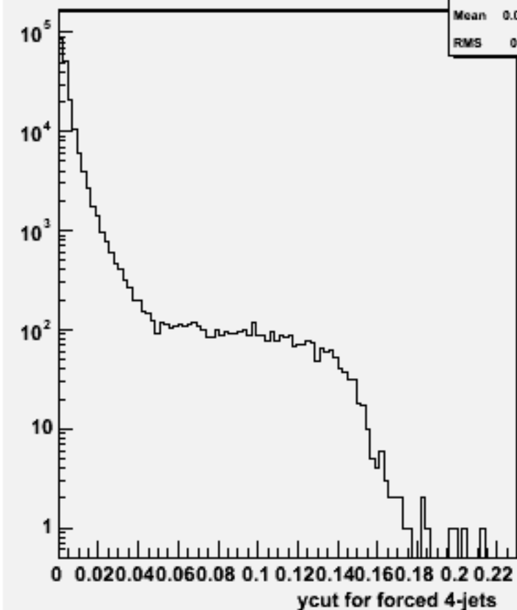
Ycut for 4-jets :w102816 e1a_n1du_o
