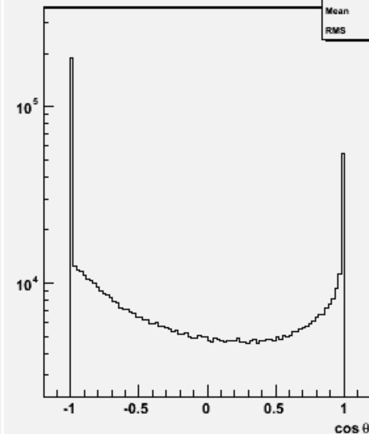
Jet cos \theta (All jets)w102816 e1a_n1du_o
