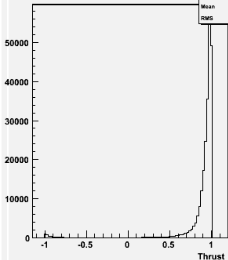
cos \Theta (thrust) w102816 e1a_n1du_o
