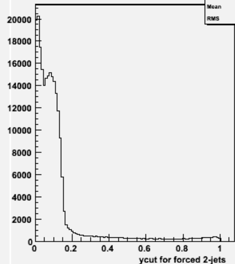
Ycut for 2-jets :w102816 e1a_n1du_o
