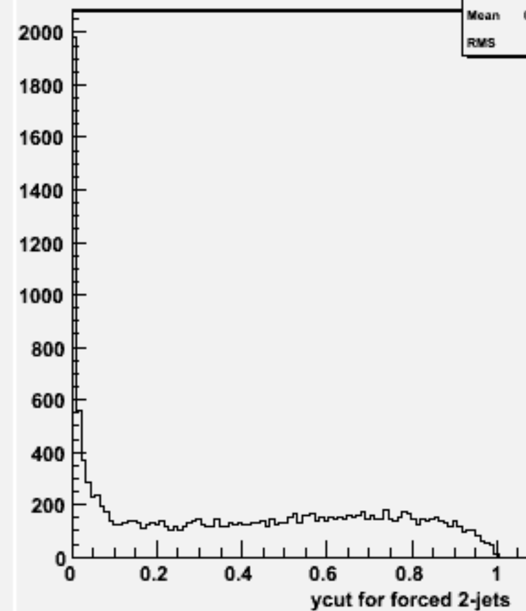
Ycut for 2-jets :w102813 e1a_n1e3n3_o
