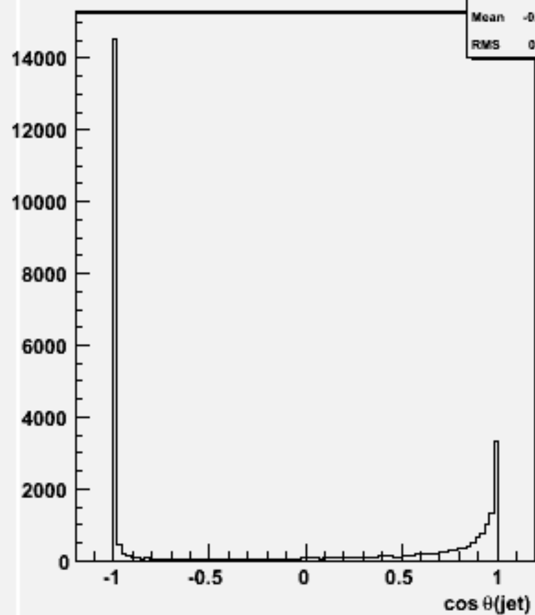
cos \theta for 2-jets :w102813 e1a_n1e3n3_o
