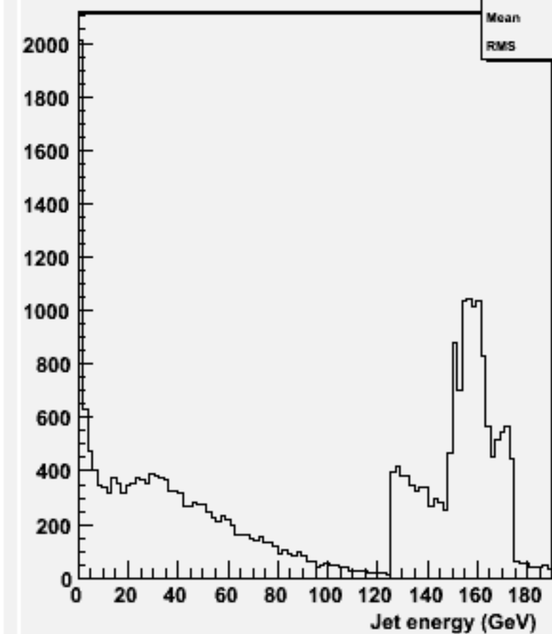
energy for 2-jets :w102813 e1a_n1e3n3_o
