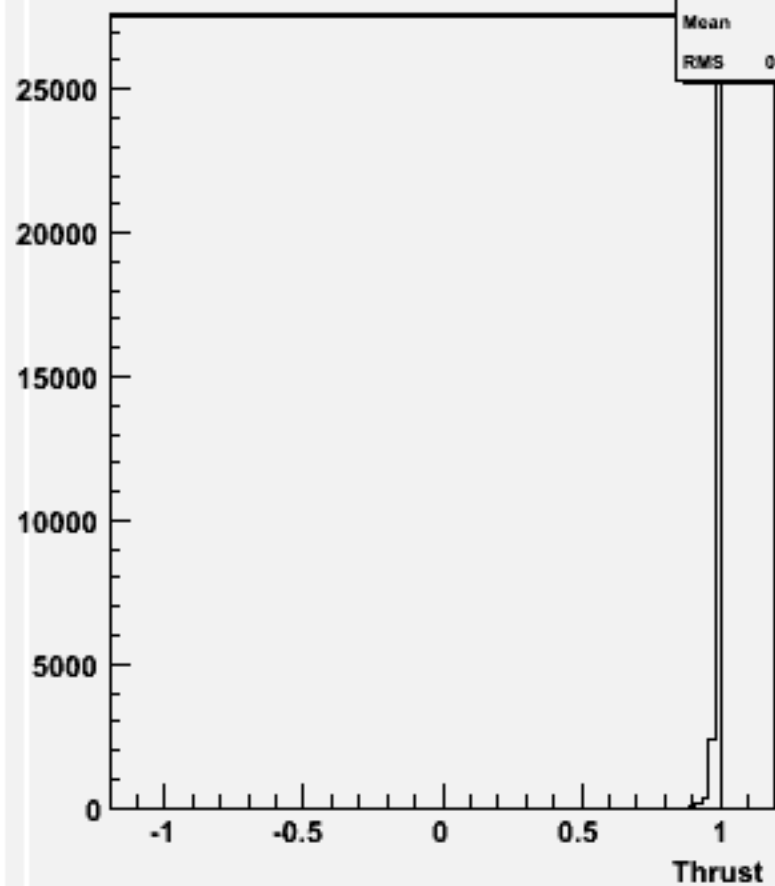
cos \Theta (thrust) w102813 e1a_n1e3n3_o
