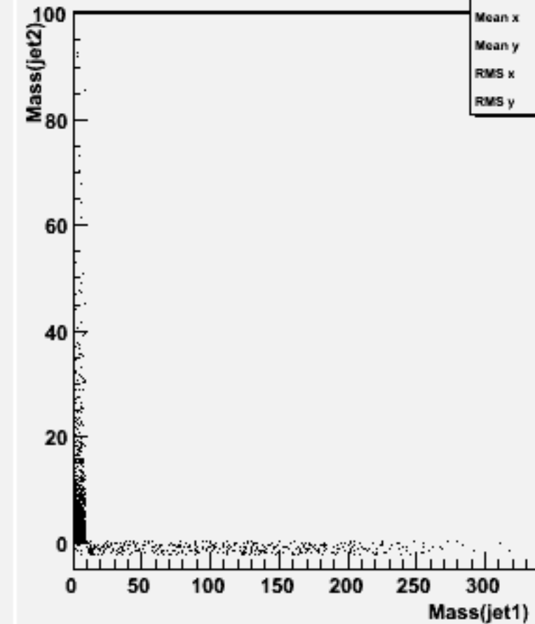
Jet mass for forced 2-jets : w102813 e1a_n1e3n3_o
