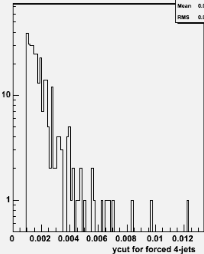
Ycut for 4-jets :w102812 e1a_n1e3n3_o
