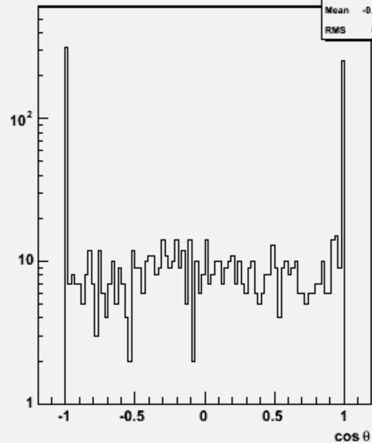
Jet cos \theta (All jets)w102812 e1a_n1e3n3_o
