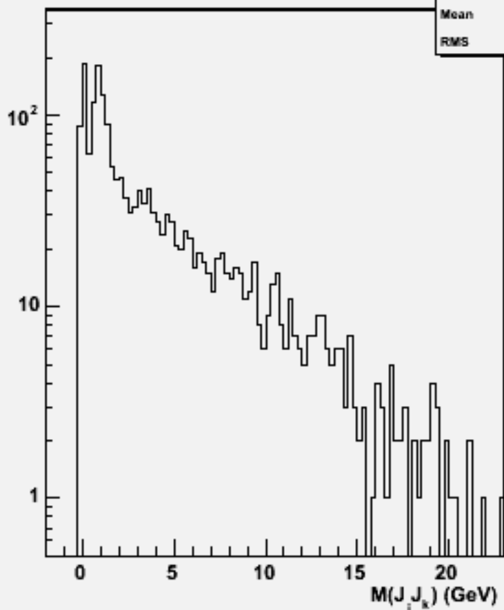
2jets mass(All comb)w102812 e1a_n1e3n3_o
