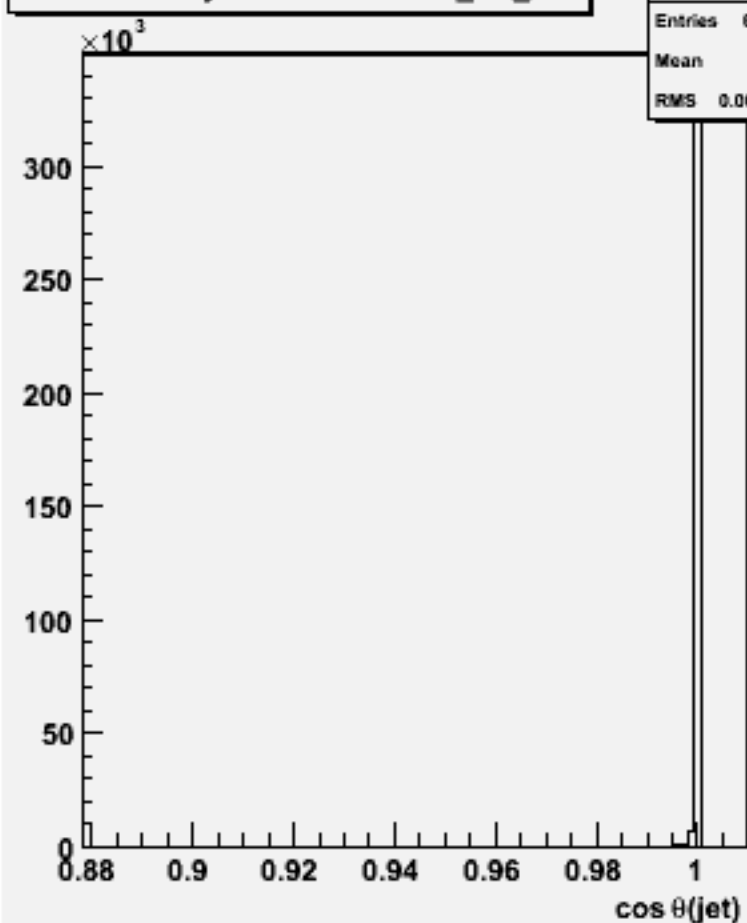
cos \theta for 2-jets :w102802 aa_bb_o
