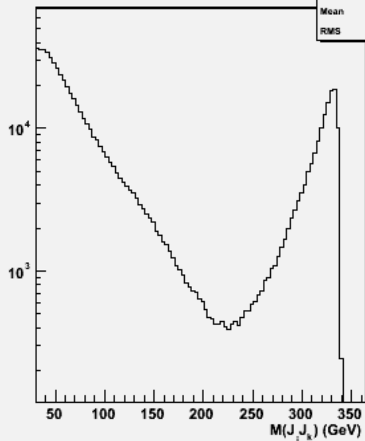
2jets mass(All comb)w102802 aa_bb_o
