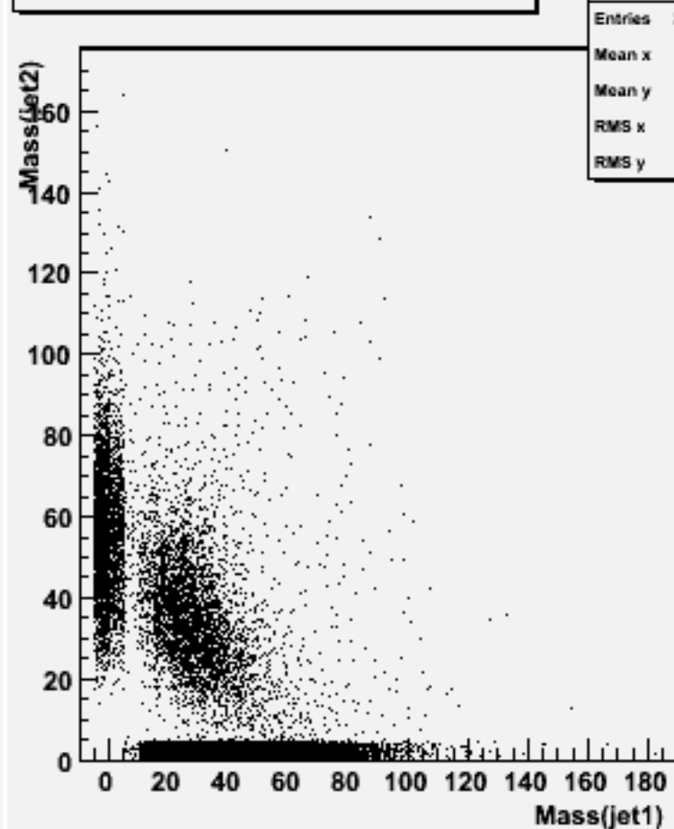
Jet mass for forced 2-jets : w102802 aa_bb_o
