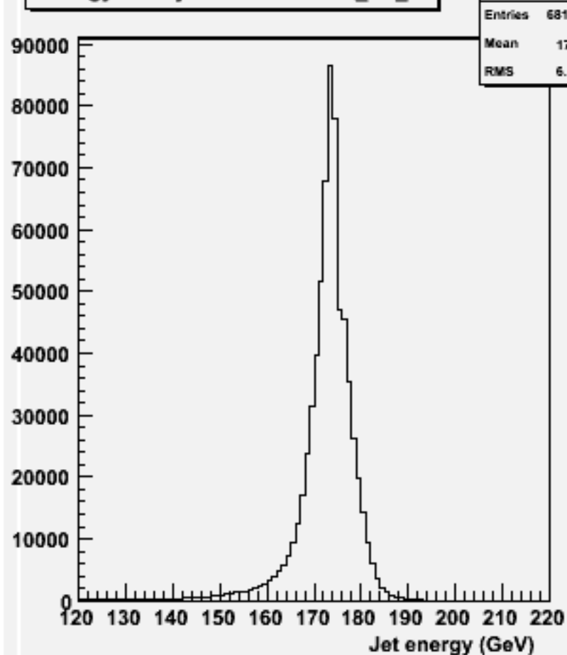
energy for 2-jets :w102802 aa_bb_o
