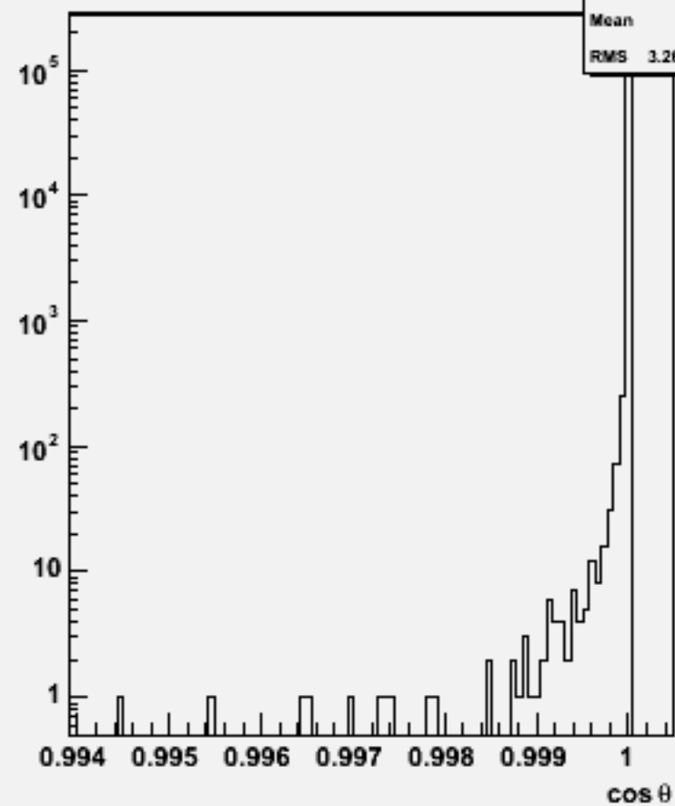
Jet cos \theta (All jets)w102802 aa_bb_o
