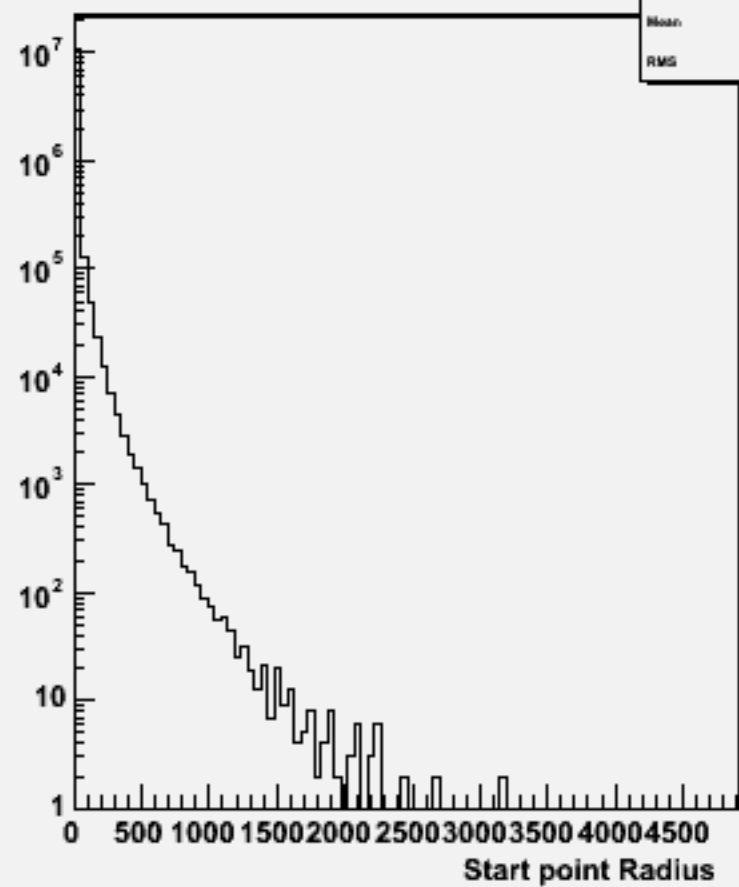
Start point R : w102802 aa_bb_o
