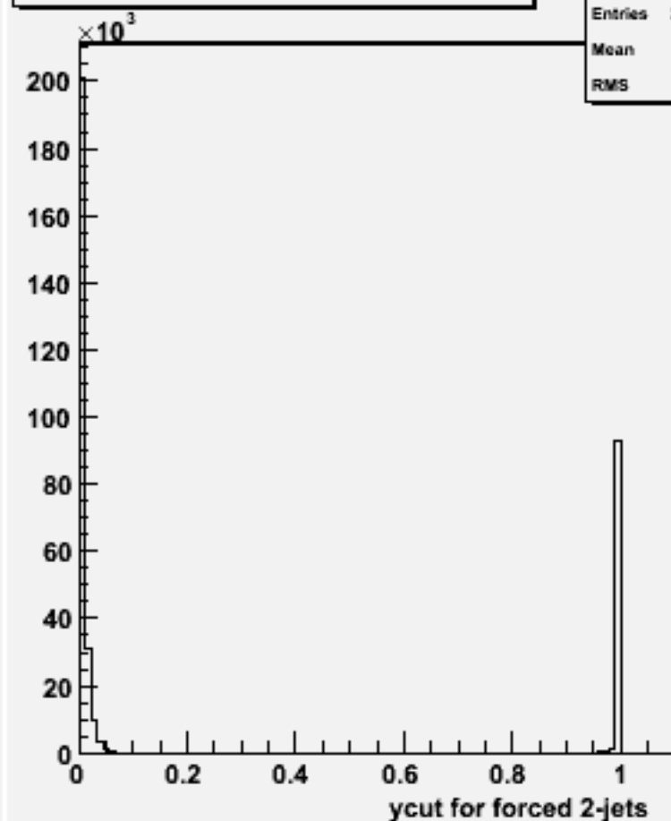
Ycut for 2-jets :w102802 aa_bb_o
