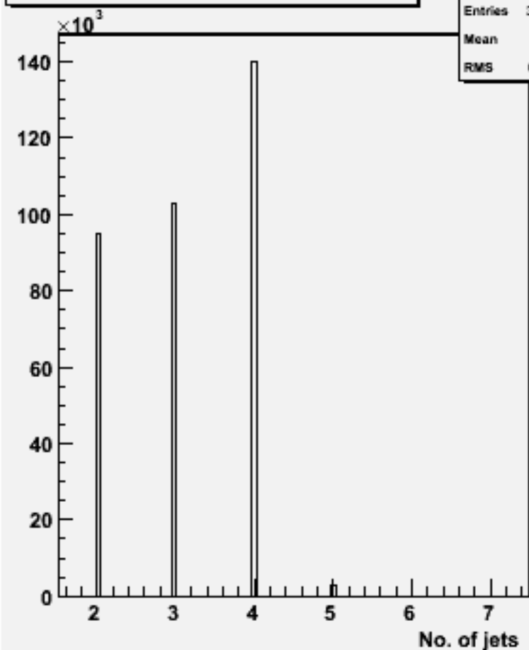
No. jets (ycut=0.001) : w102802 aa_bb_o
