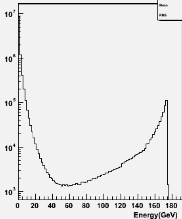
Particle Energy : w102802 aa_bb_o
