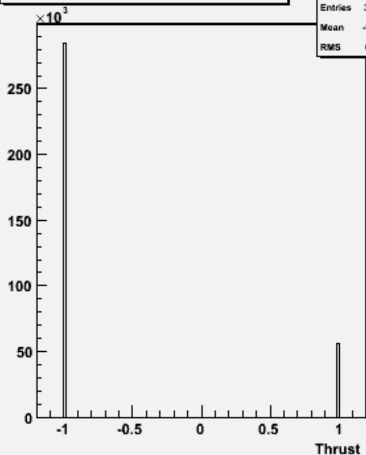
cos \Theta (thrust) w102802 aa_bb_o
