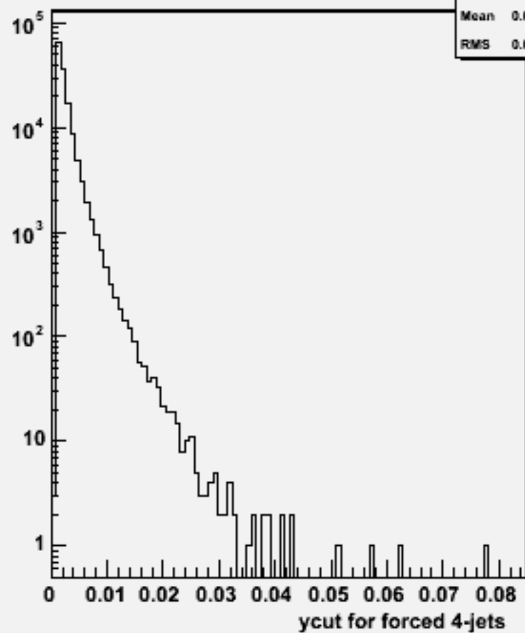
Ycut for 4-jets :w102802 aa_bb_o
