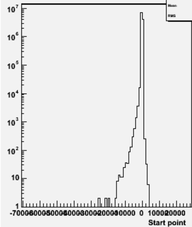
Start point Z : w102802 aa_bb_o
