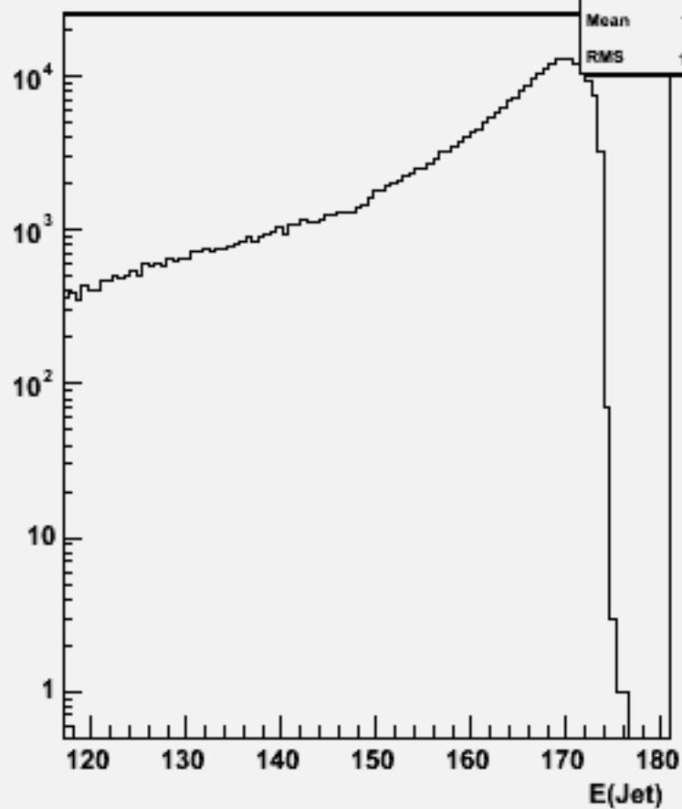
Jet energies(All jets)w102802 aa_bb_o
