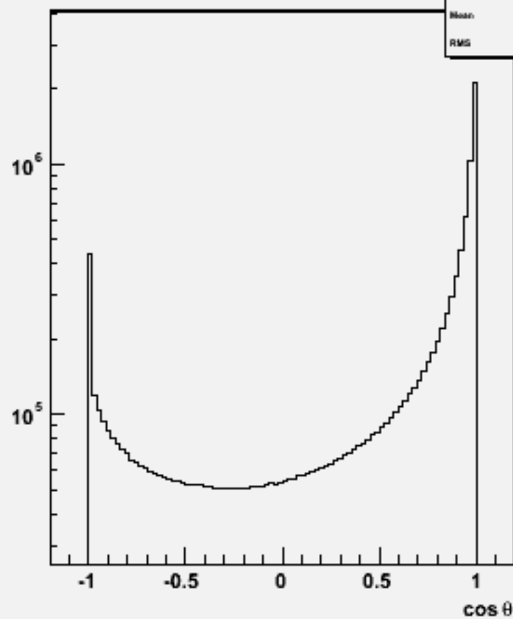
Particle cos \theta : w102801 aa_bb_o
