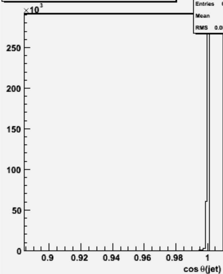
cos \theta for 2-jets :w102801 aa_bb_o
