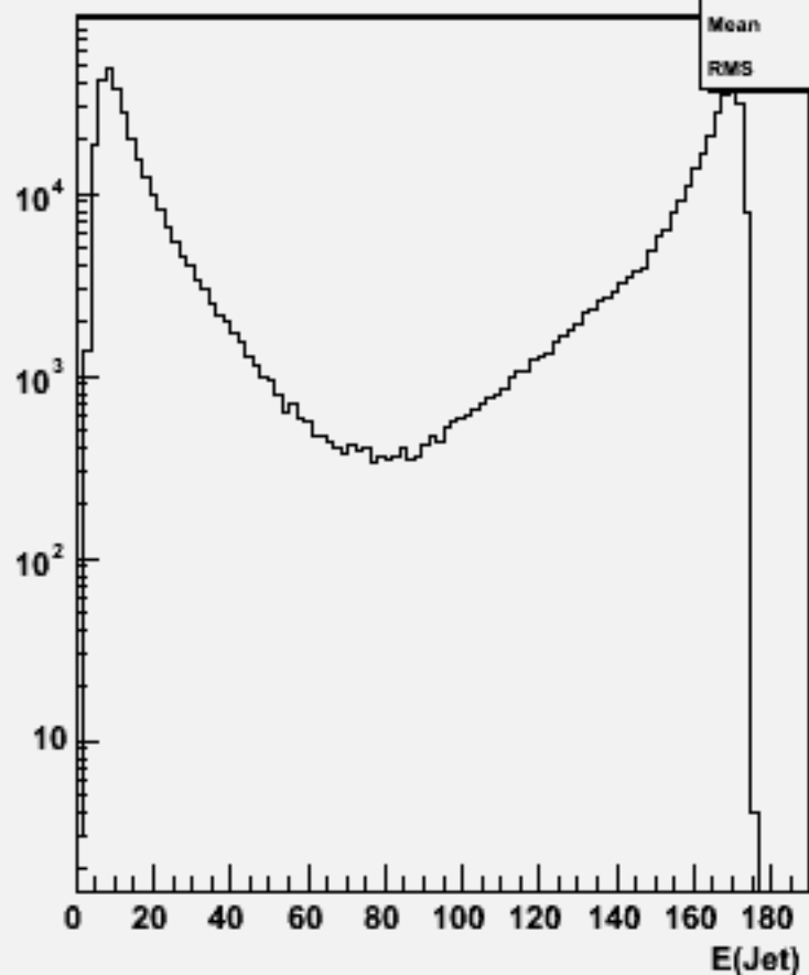
Jet energies(All jets)w102801 aa_bb_o
