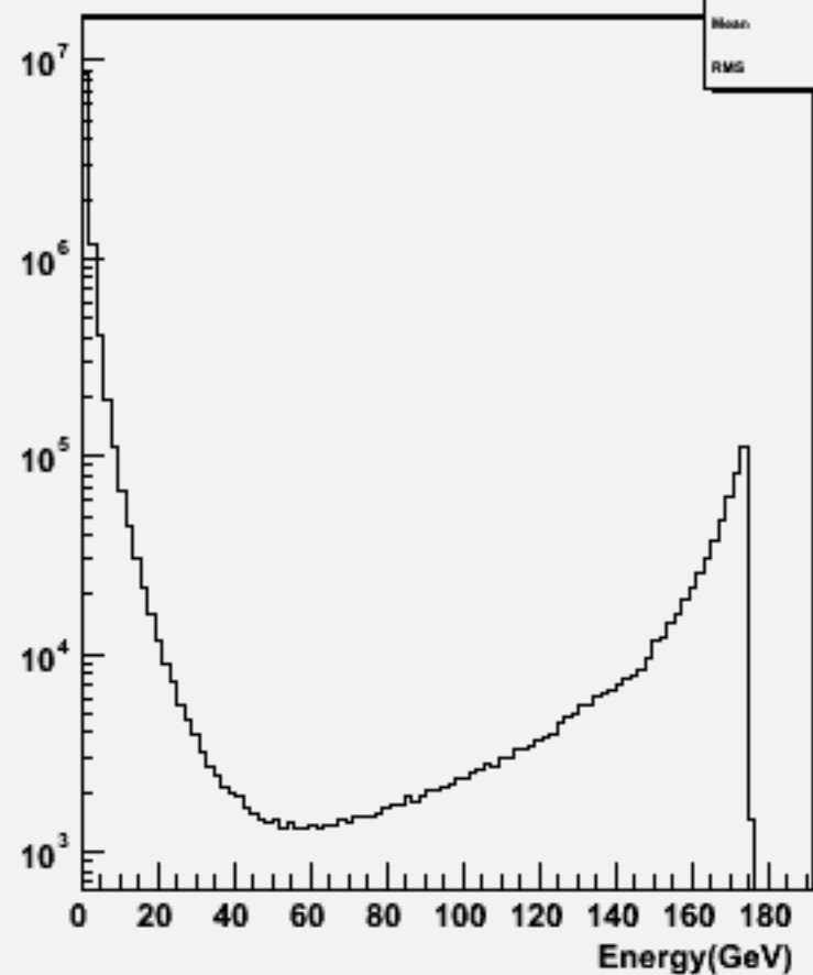
Particle Energy : w102801 aa_bb_o
