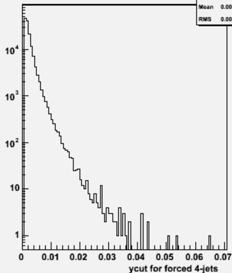
Ycut for 4-jets :w102801 aa_bb_o
