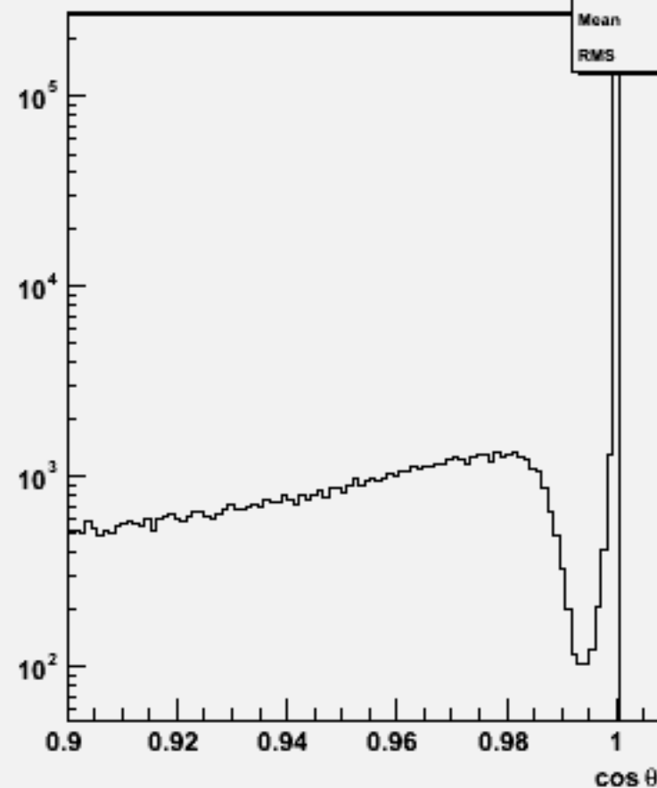
Jet cosθ (All jets)w102801 aa_bb_o
