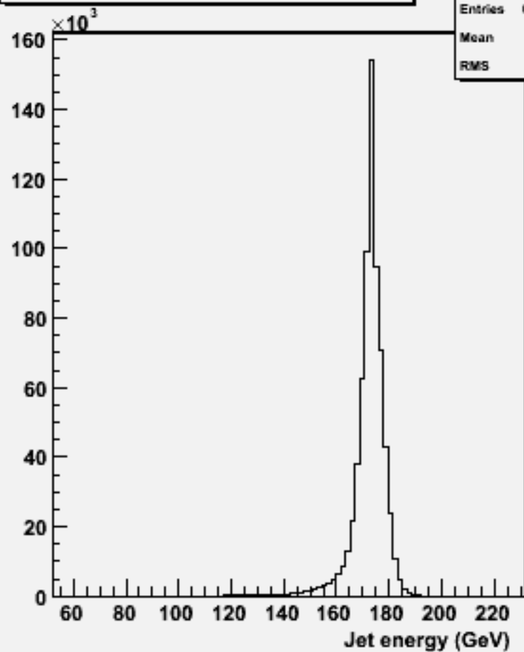
energy for 2-jets :w102801 aa_bb_o
