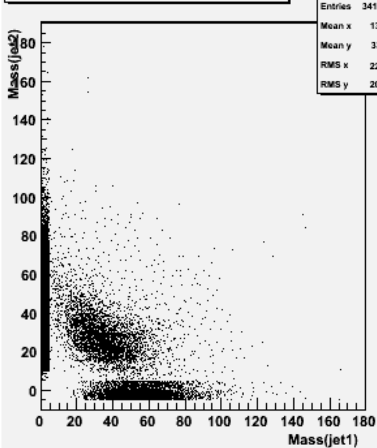
Jet mass for forced 2-jets : w102801 aa_bb_o
