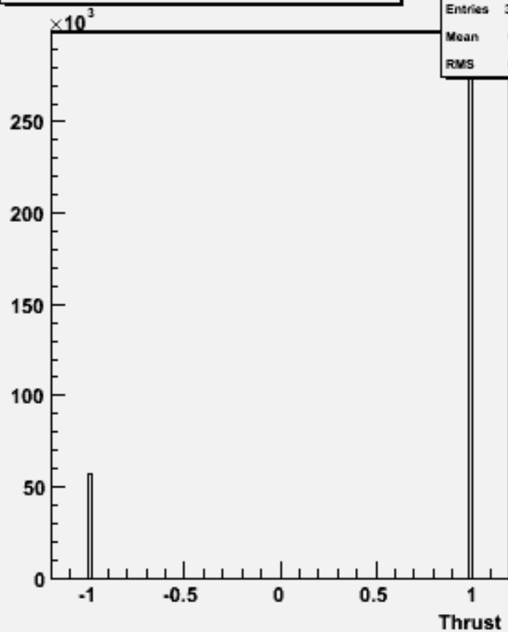
cos \Theta (thrust) w102801 aa_bb_o
