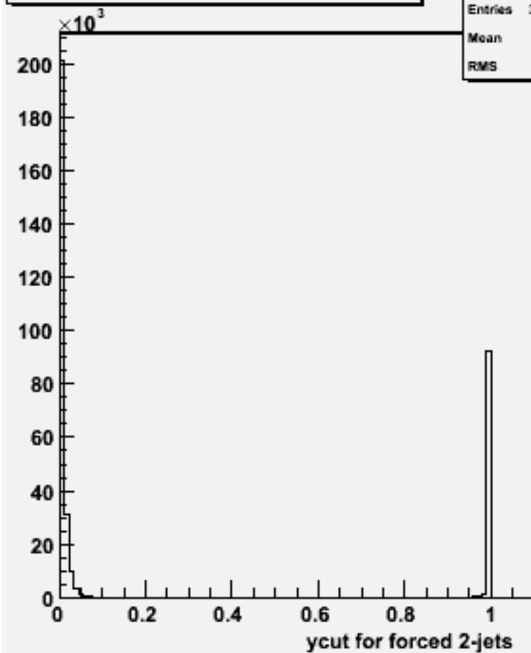
Ycut for 2-jets :w102801 aa_bb_o
