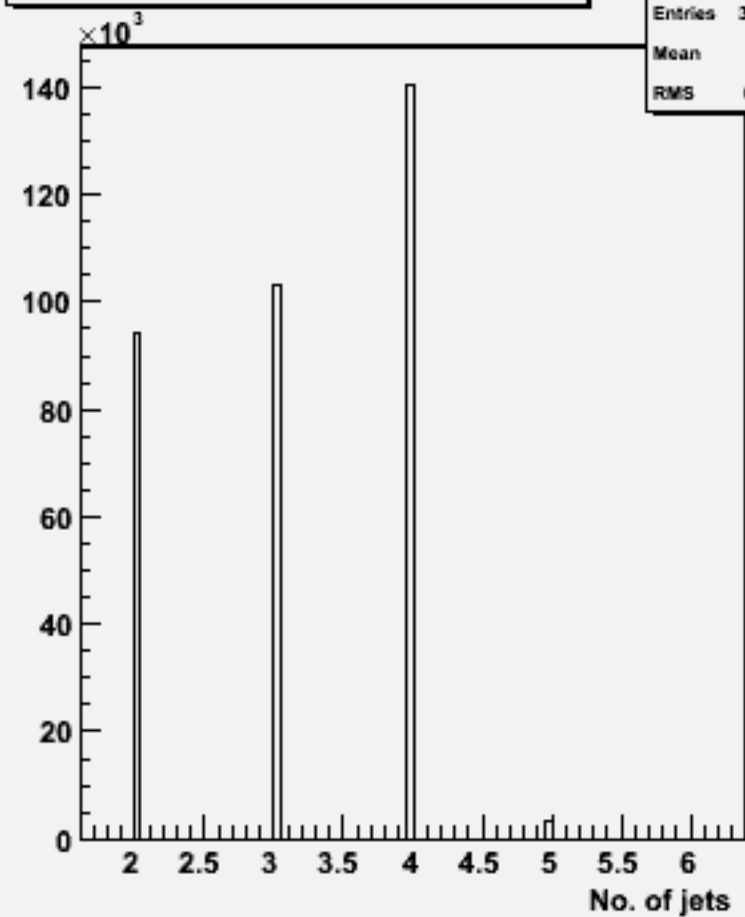
No. jets (ycut=0.001) : w102801 aa_bb_o
