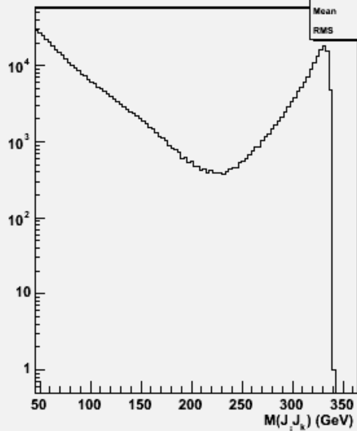
2jets mass(All comb)w102801 aa_bb_o
