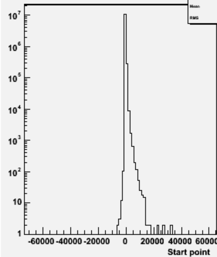
Start point Z : w102801 aa_bb_o
