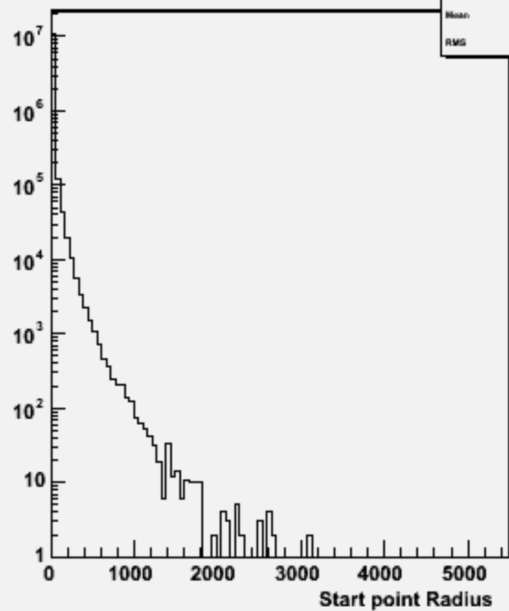
Start point R : w102801 aa_bb_o
