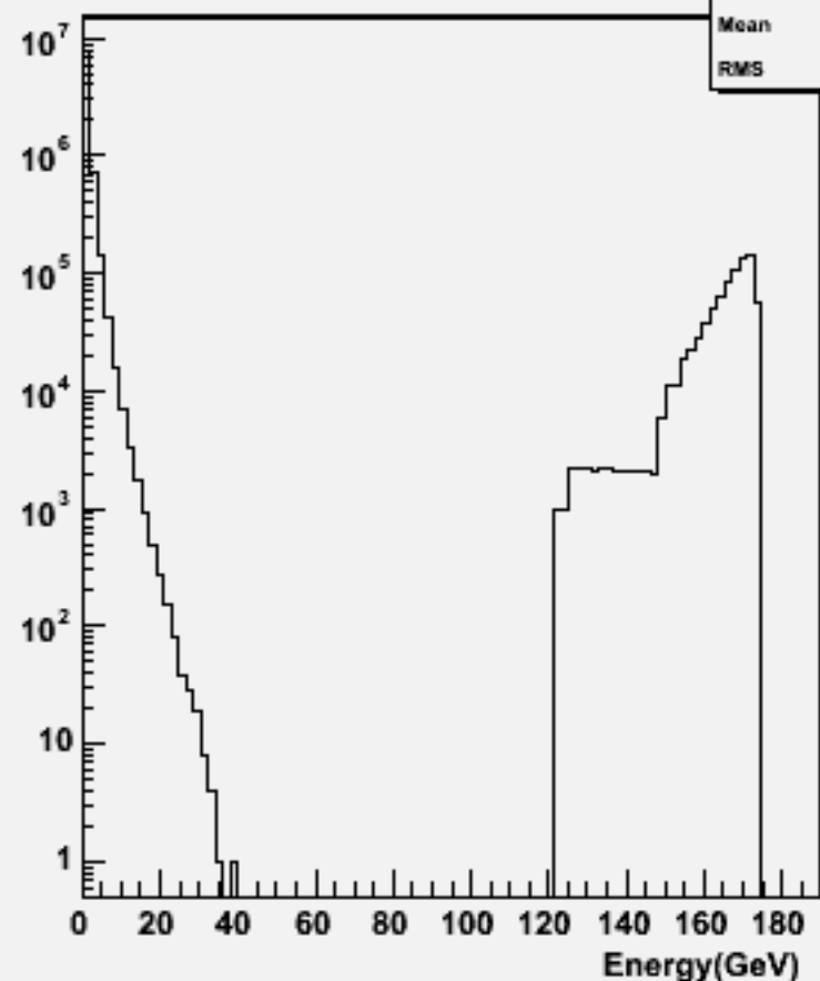
Particle Energy : w102799 aa_cc_o
