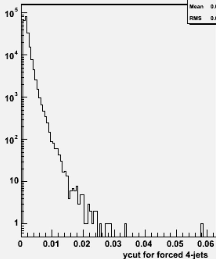
Ycut for 4-jets :w102799 aa_cc_o
