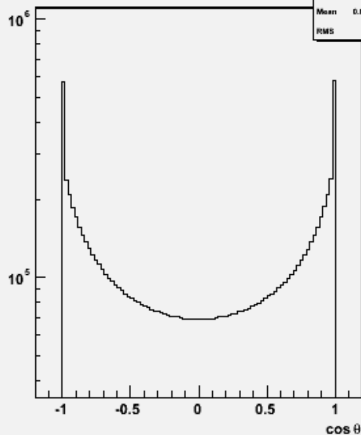
Particle cosθ : w102799 aa_cc_o
