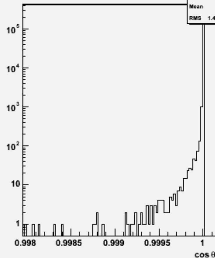
Jet cosθ (All jets)w102799 aa_cc_o
