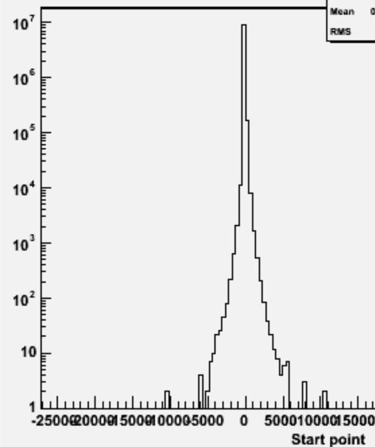
Start point Z : w102799 aa_cc_o
