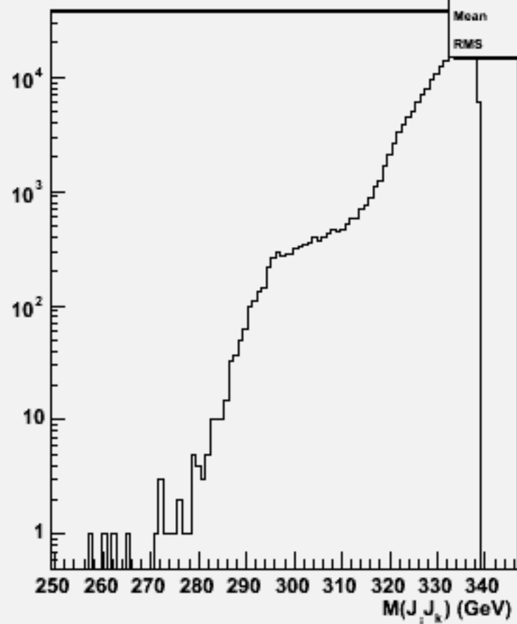
2jets mass(All comb)w102799 aa_cc_o
