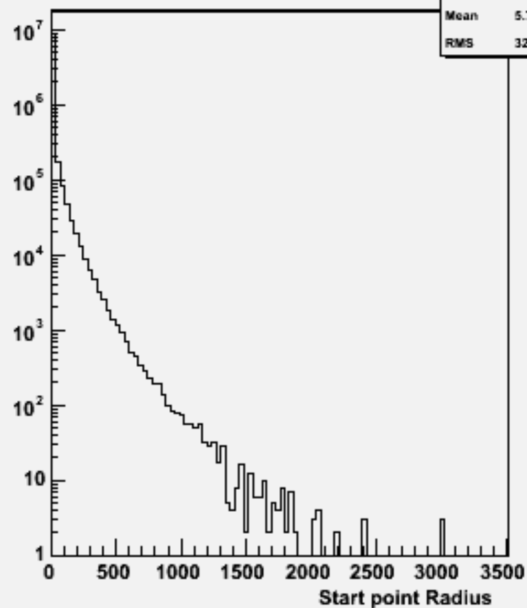
Start point R : w102799 aa_cc_o
