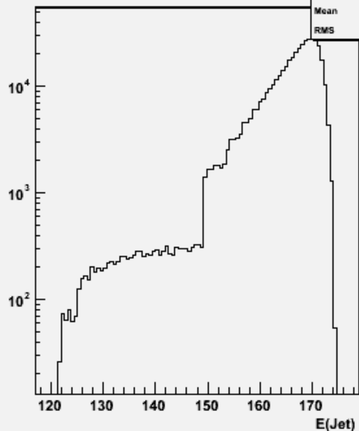
Jet energies(All jets)w102799 aa_cc_o
