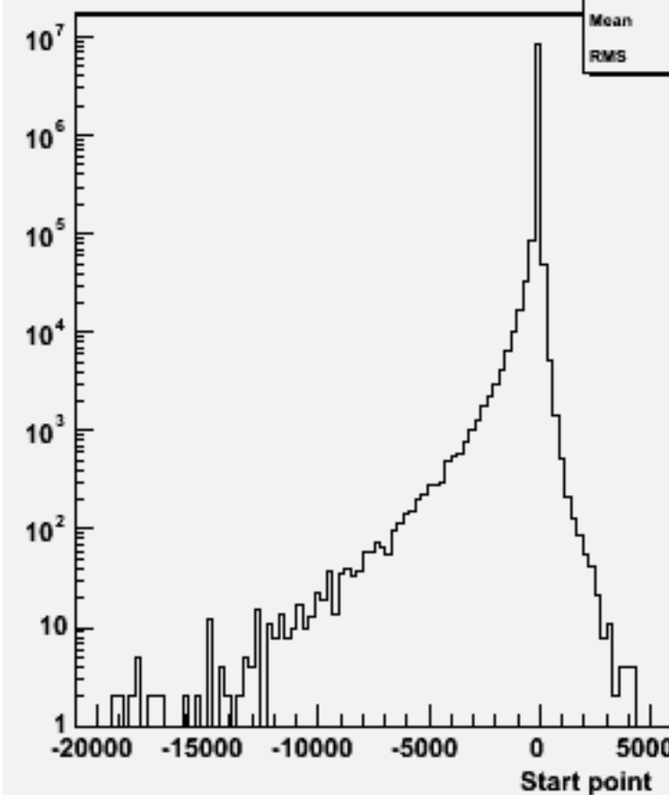
Start point Z : w102798 aa_cc_o
