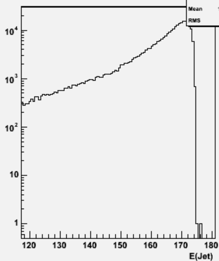
Jet energies(All jets)w102798 aa_cc_o
