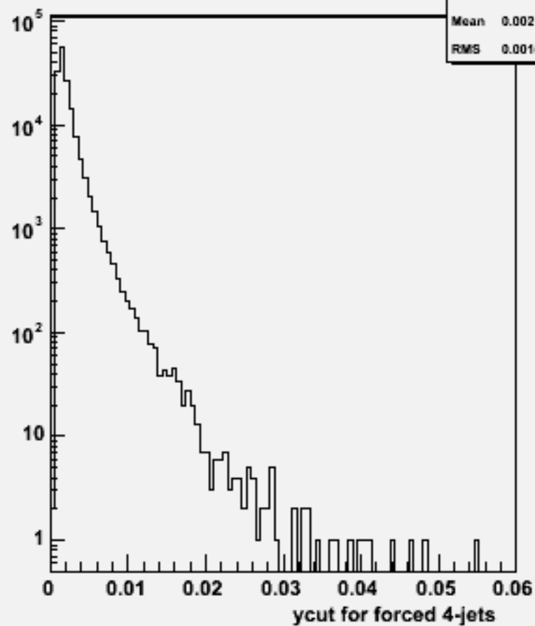
Ycut for 4-jets :w102798 aa_cc_o
