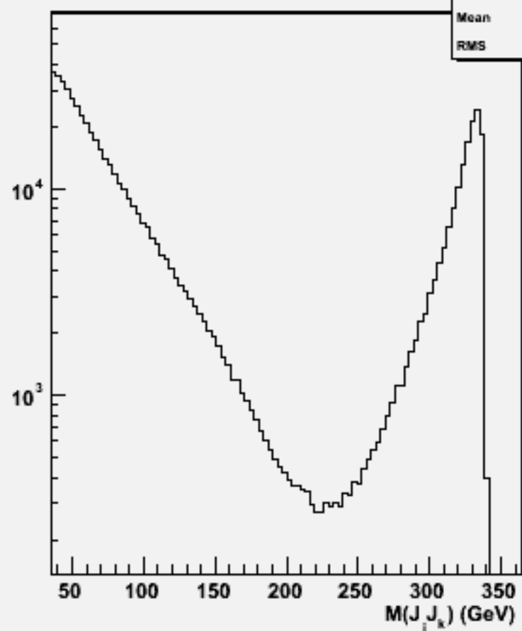
2jets mass(All comb)w102798 aa_cc_o
