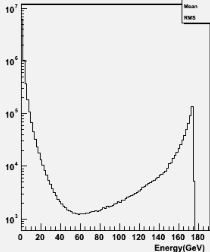
Particle Energy : w102798 aa_cc_o
