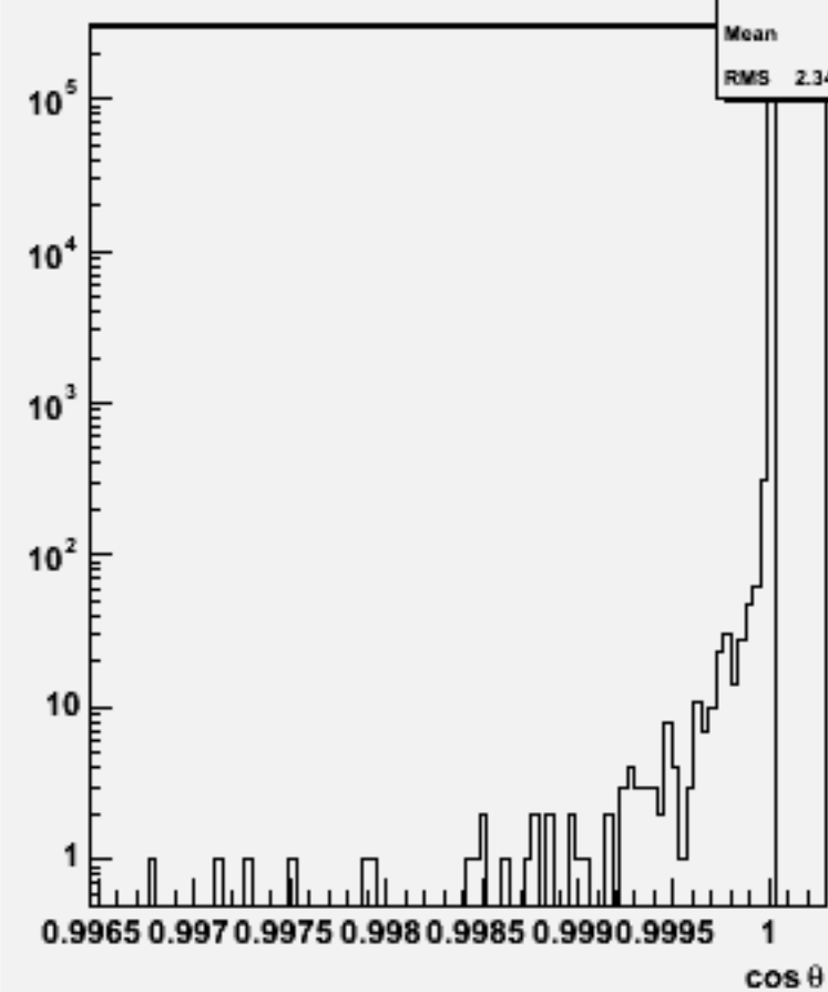
Jet cos \theta (All jets)w102798 aa_cc_o
