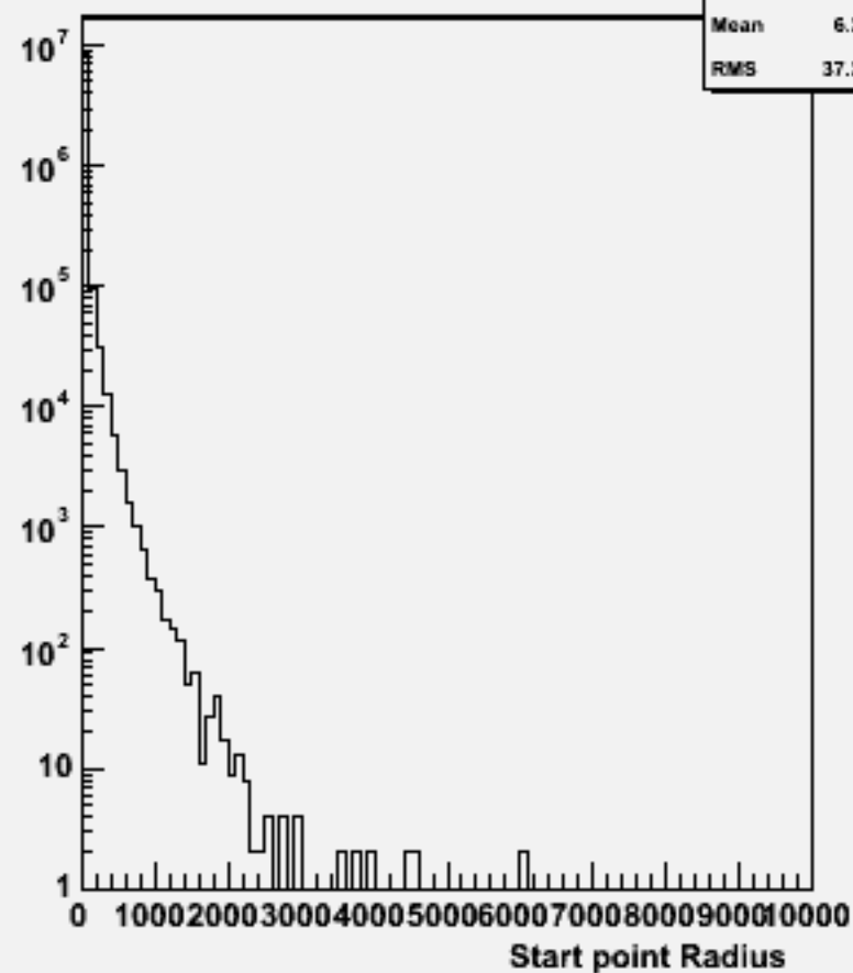
Start point R : w102798 aa_cc_o
