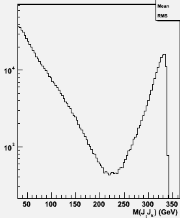
2jets mass(All comb)w102796 aa_cc_o
