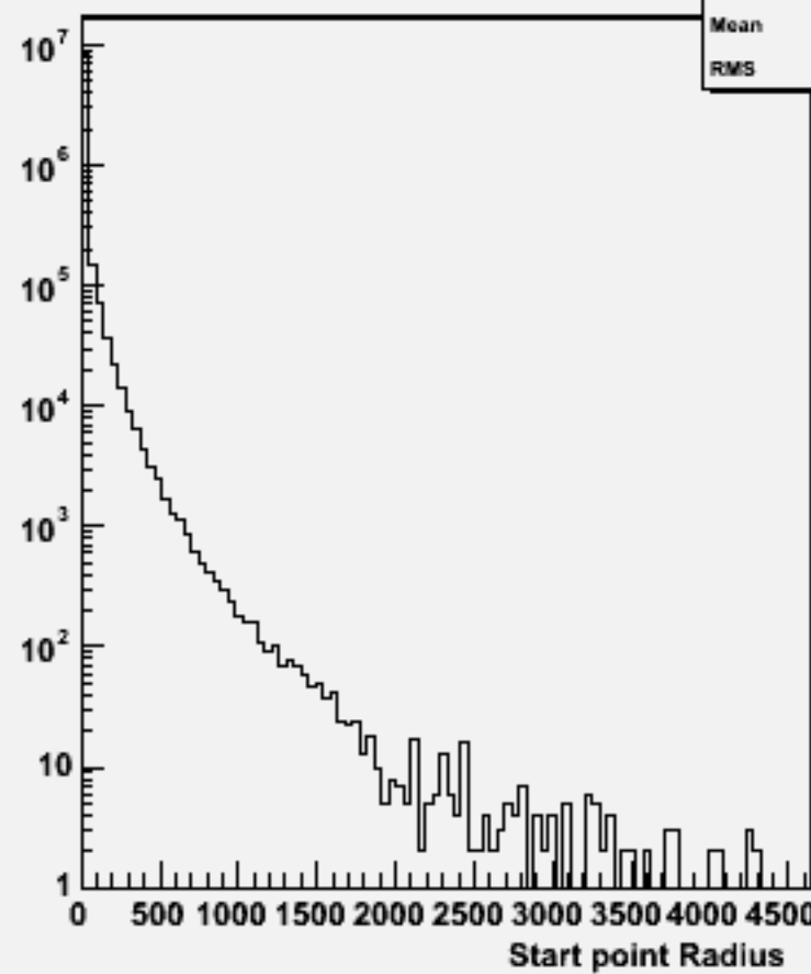
Start point R : w102796 aa_cc_o
