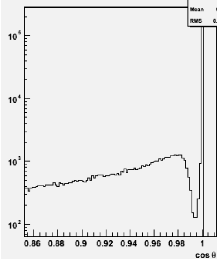
Jet cosθ (All jets)w102796 aa_cc_o
