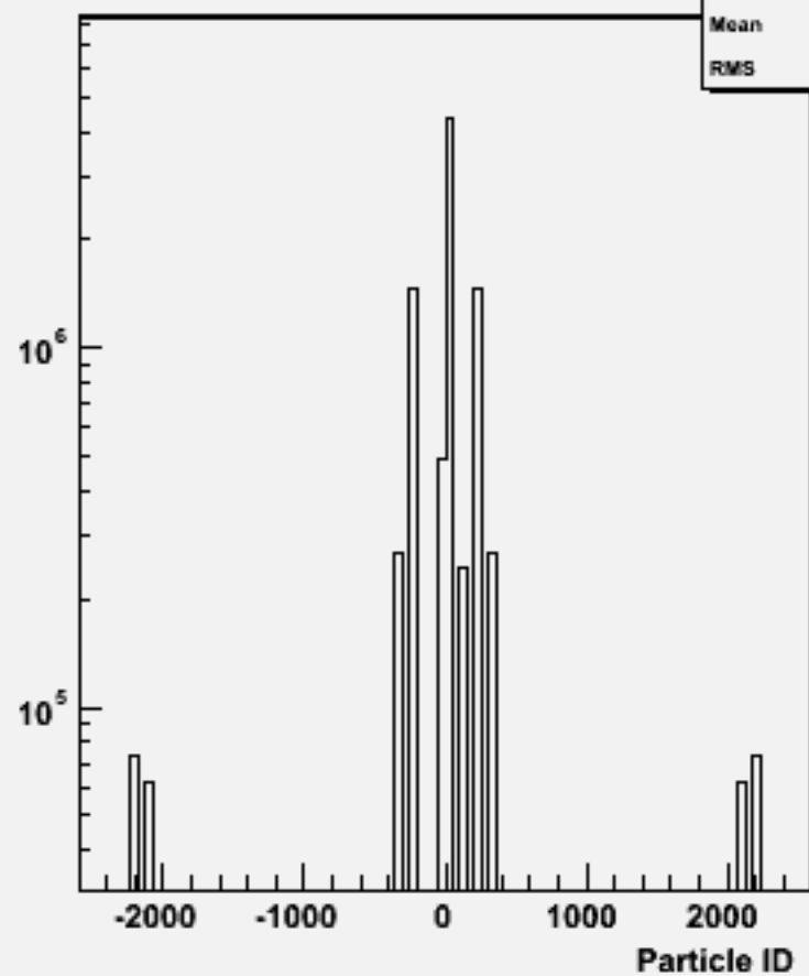
Particle ID : w102796 aa_cc_o
