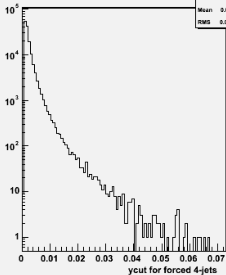
Ycut for 4-jets :w102796 aa_cc_o
