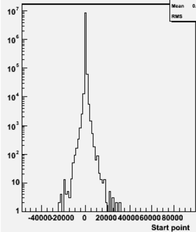
Start point Z : w102796 aa_cc_o
