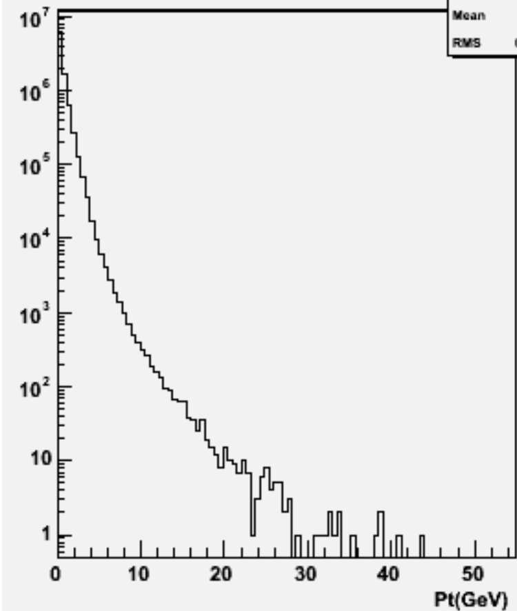
Particle Pt : w102796 aa_cc_o
