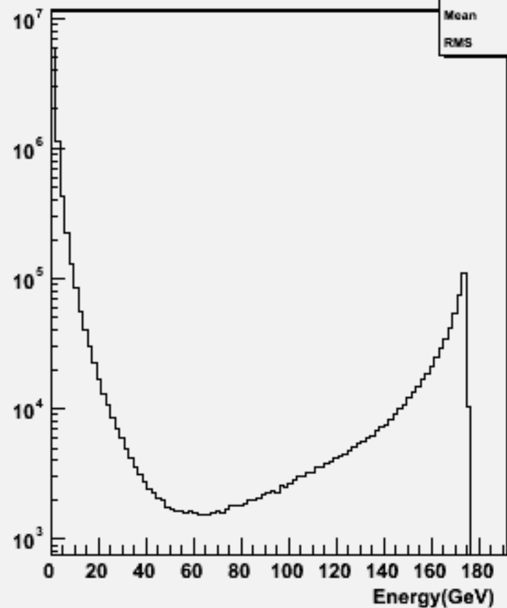
Particle Energy : w102796 aa_cc_o
