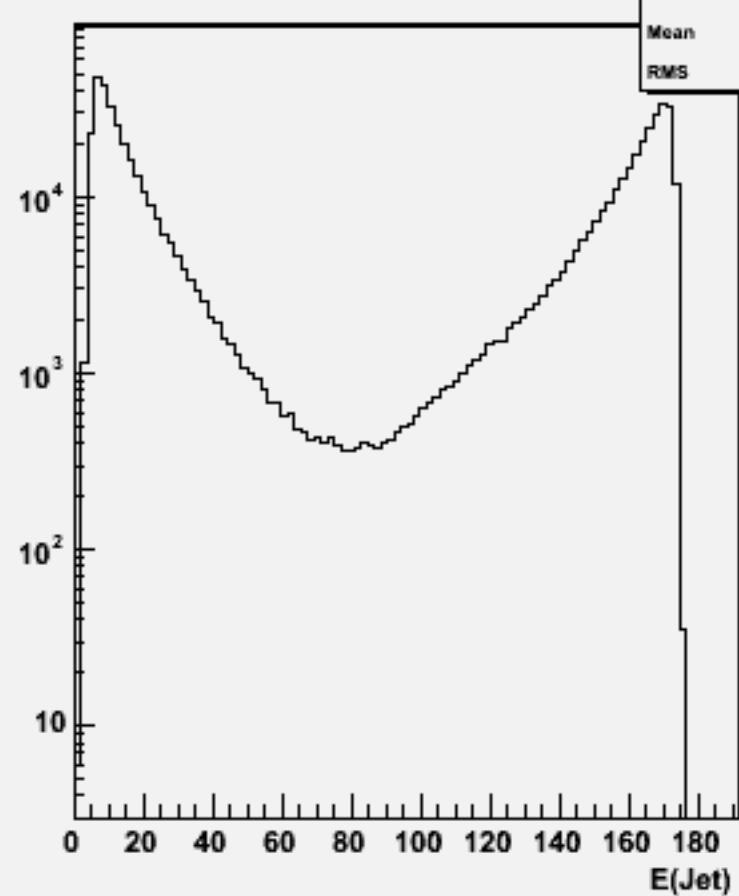
Jet energies(All jets)w102796 aa_cc_o
