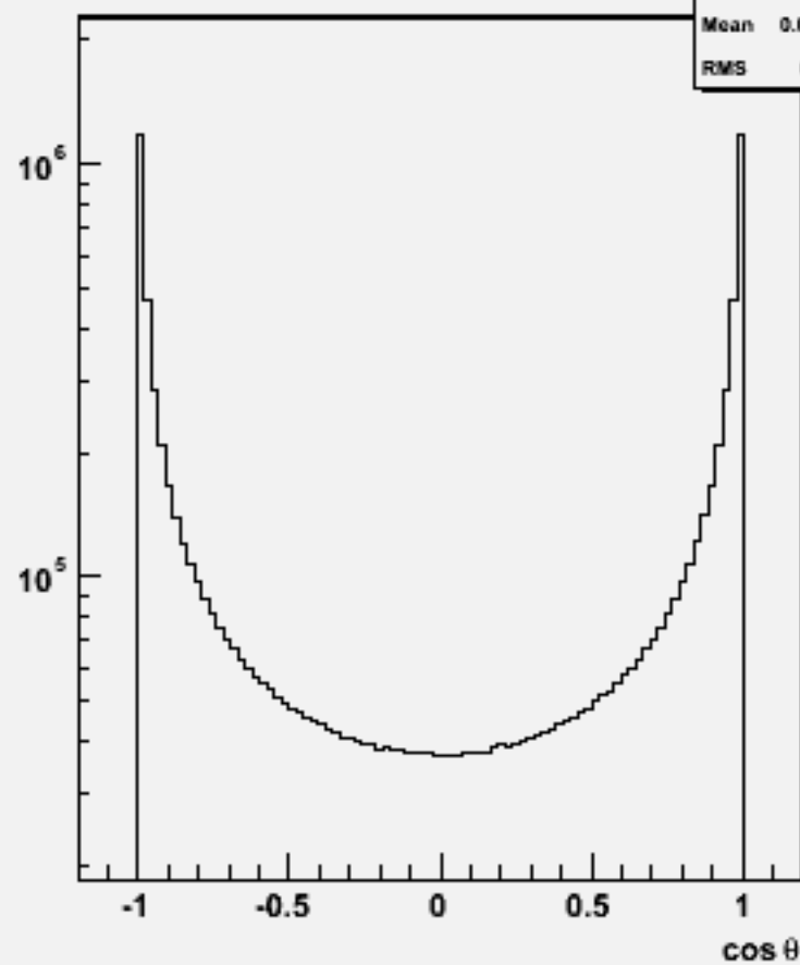
Particle cosθ : w102796 aa_cc_o
