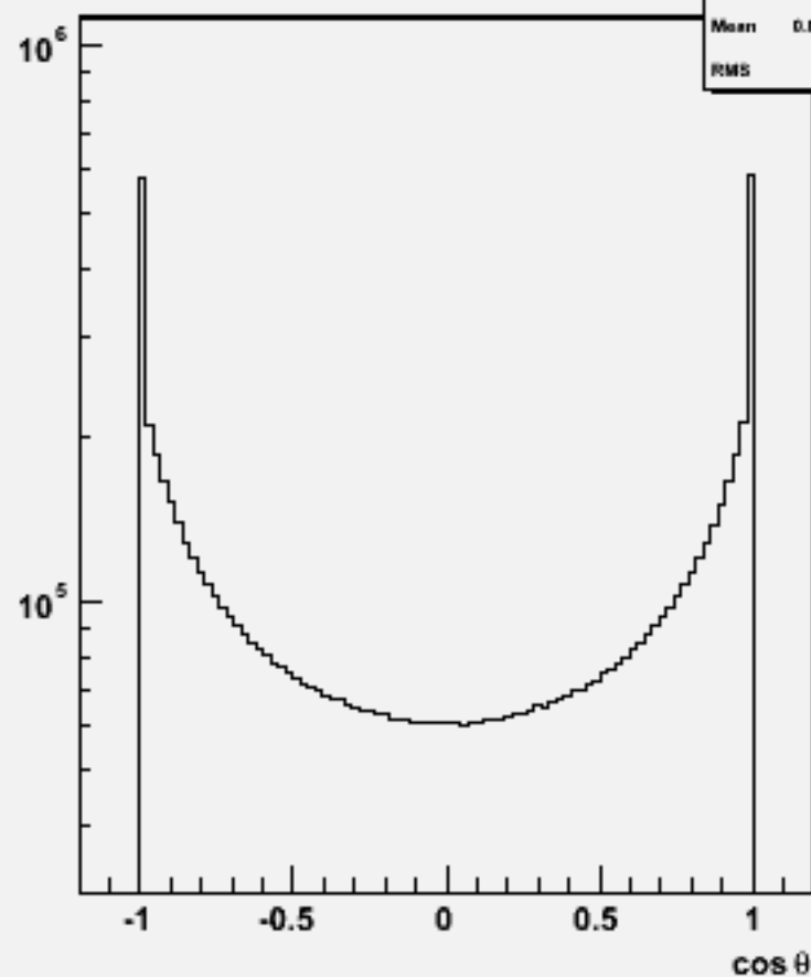
Particle cosθ : w102795 aa_ss_o
