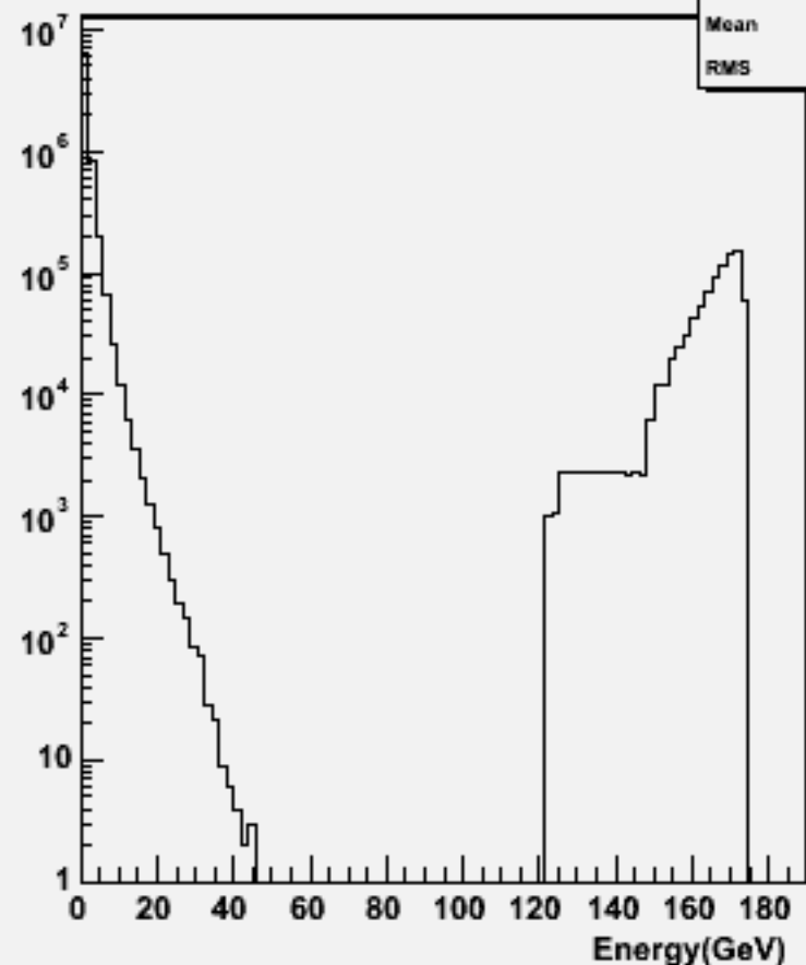
Particle Energy : w102795 aa_ss_o
