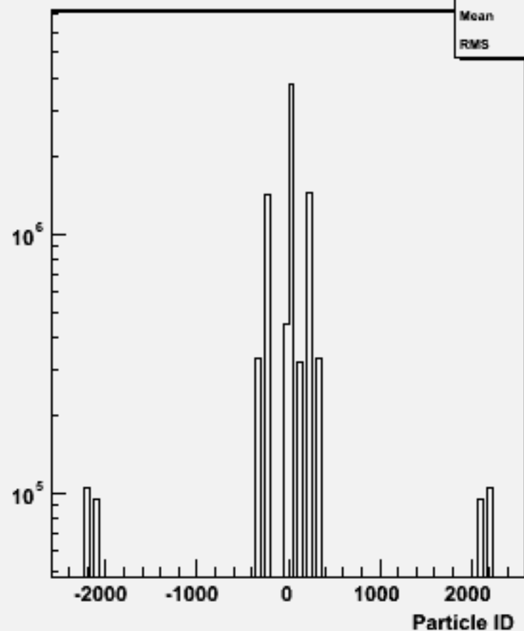
Particle ID : w102795 aa_ss_o
