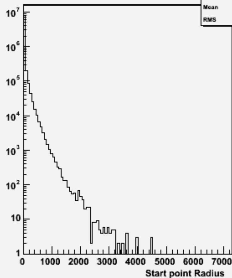
Start point R : w102795 aa_ss_o
