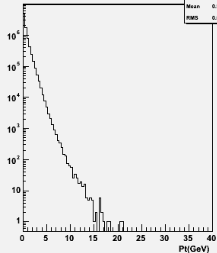
Particle Pt : w102795 aa_ss_o
