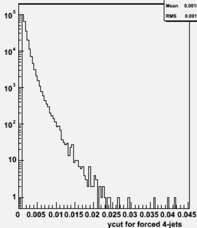
Ycut for 4-jets :w102795 aa_ss_o
