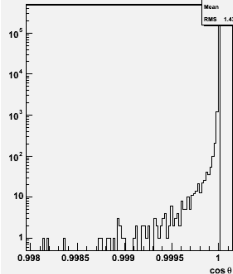
Jet cos \theta (All jets)w102795 aa_ss_o
