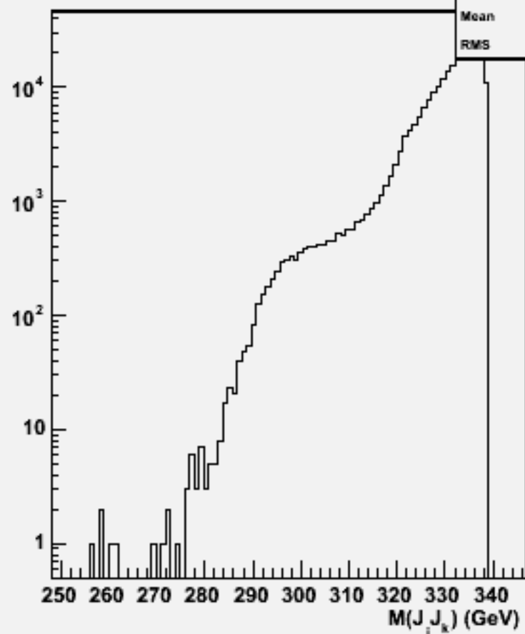
2jets mass(All comb)w102795 aa_ss_o
