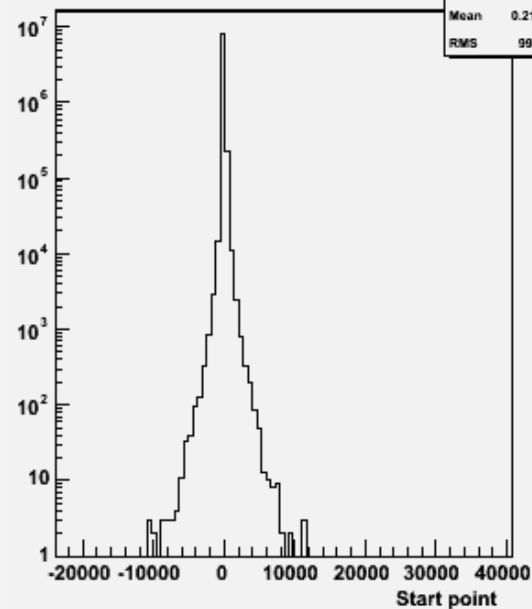
Start point Z : w102795 aa_ss_o
