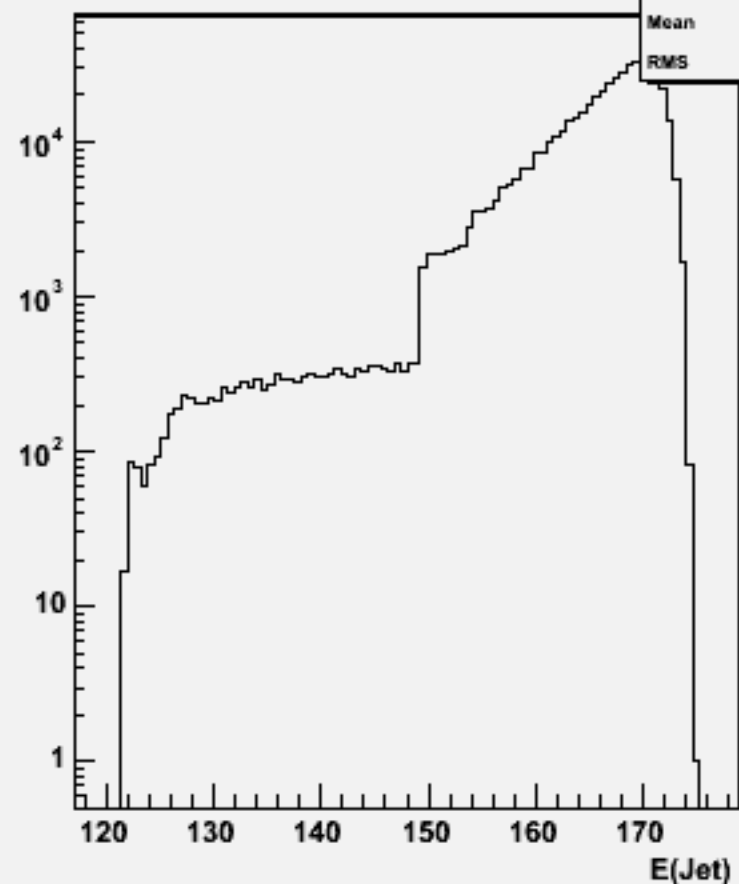
Jet energies(All jets)w102795 aa_ss_o
