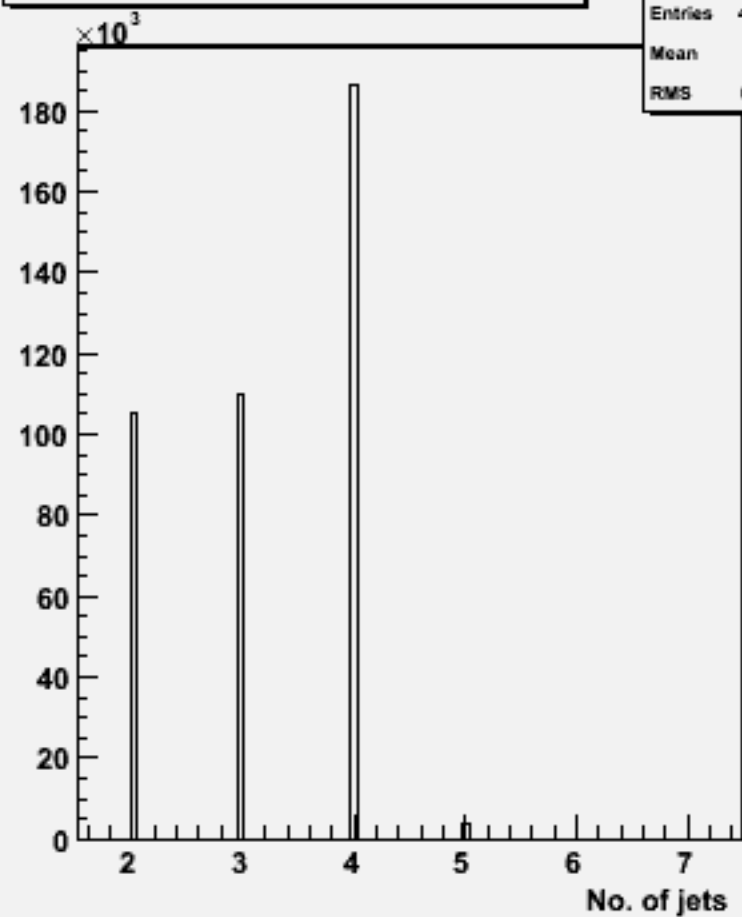
No. jets (ycut=0.001) : w102794 aa_ss_o
