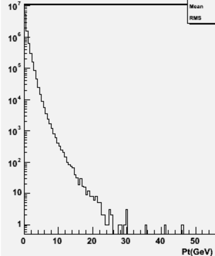
Particle Pt : w102794 aa_ss_o
