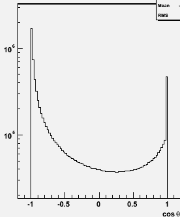
Particle cos \theta : w102794 aa_ss_o
