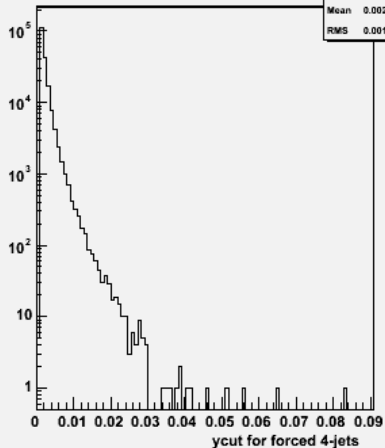
Ycut for 4-jets :w102794 aa_ss_o
