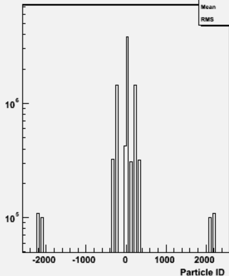
Particle ID : w102794 aa_ss_o
