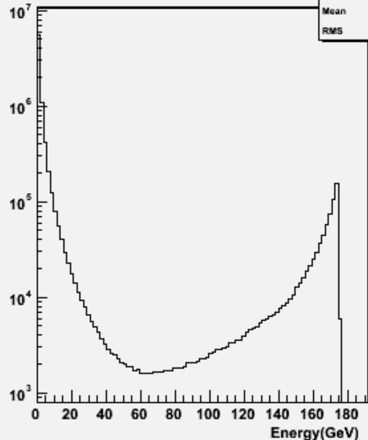
Particle Energy : w102794 aa_ss_o
