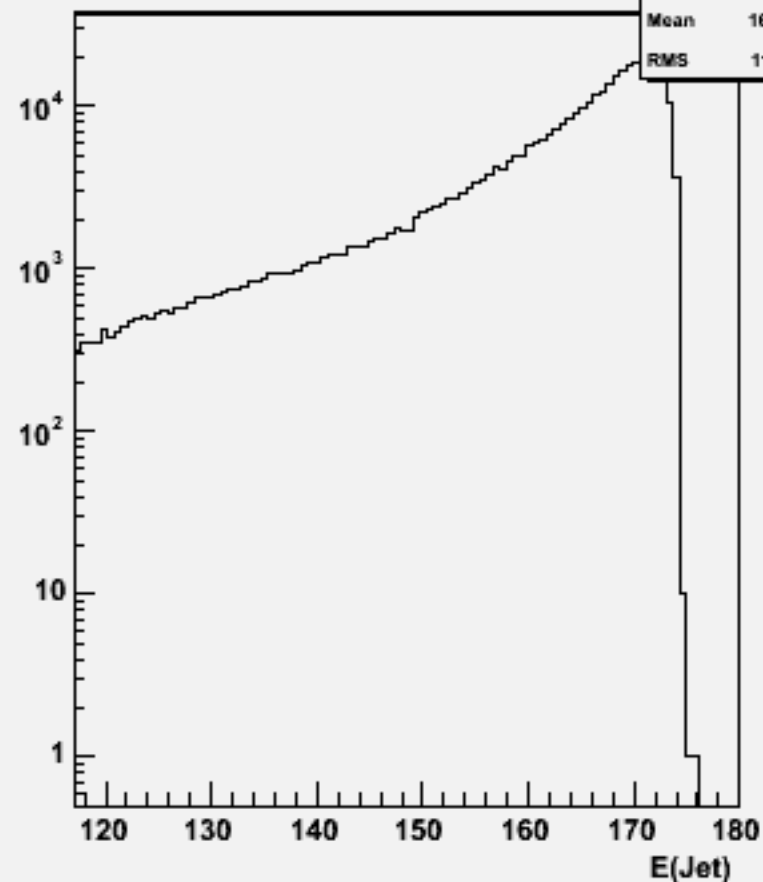
Jet energies(All jets)w102794 aa_ss_o
