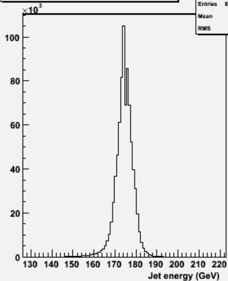
energy for 2-jets :w102794 aa_ss_o
