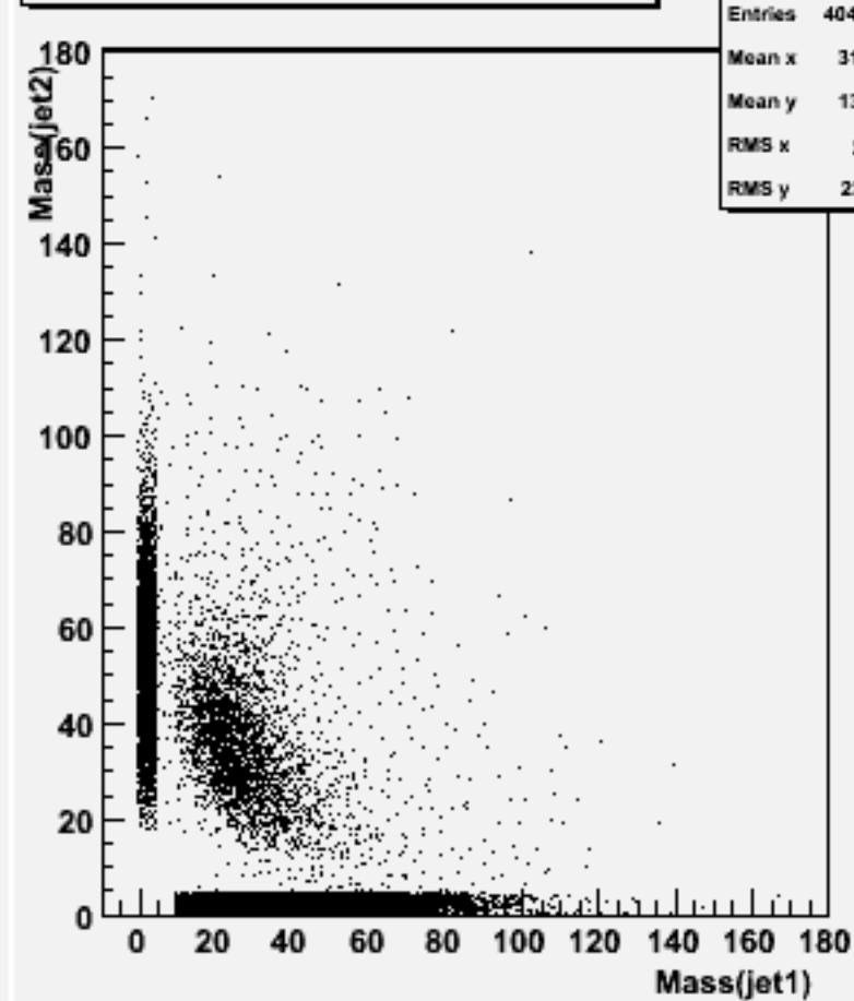
Jet mass for forced 2-jets : w102794 aa_ss_o
