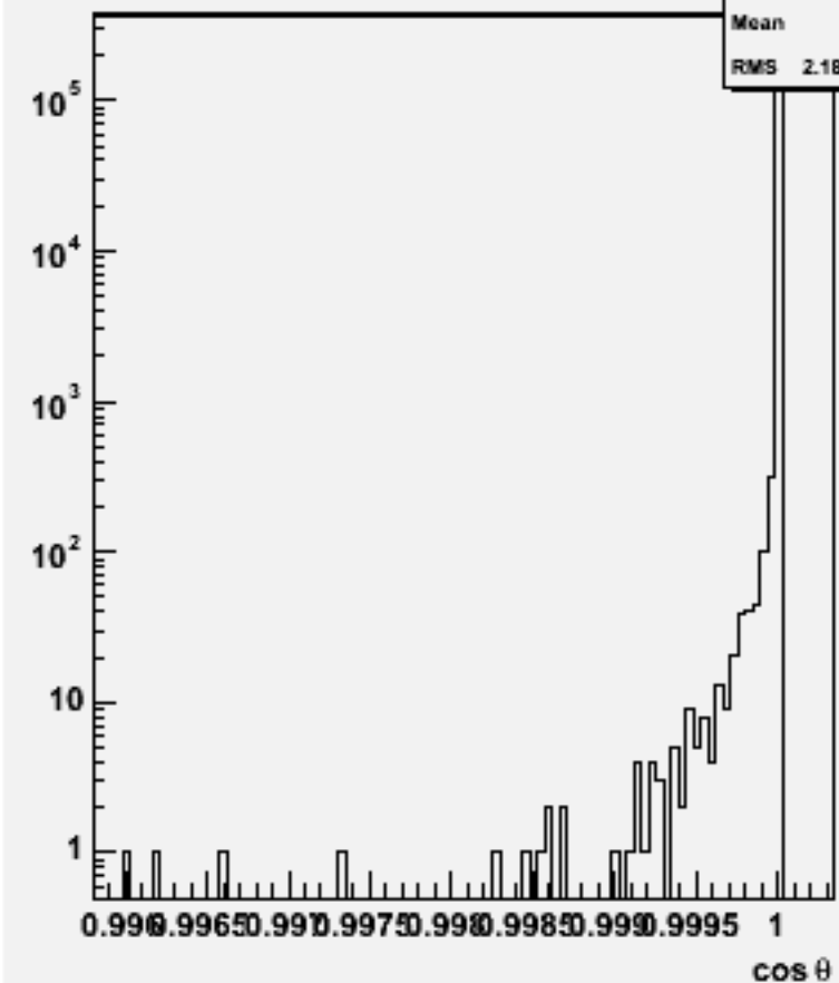
Jet cosθ (All jets)w102794 aa_ss_o
