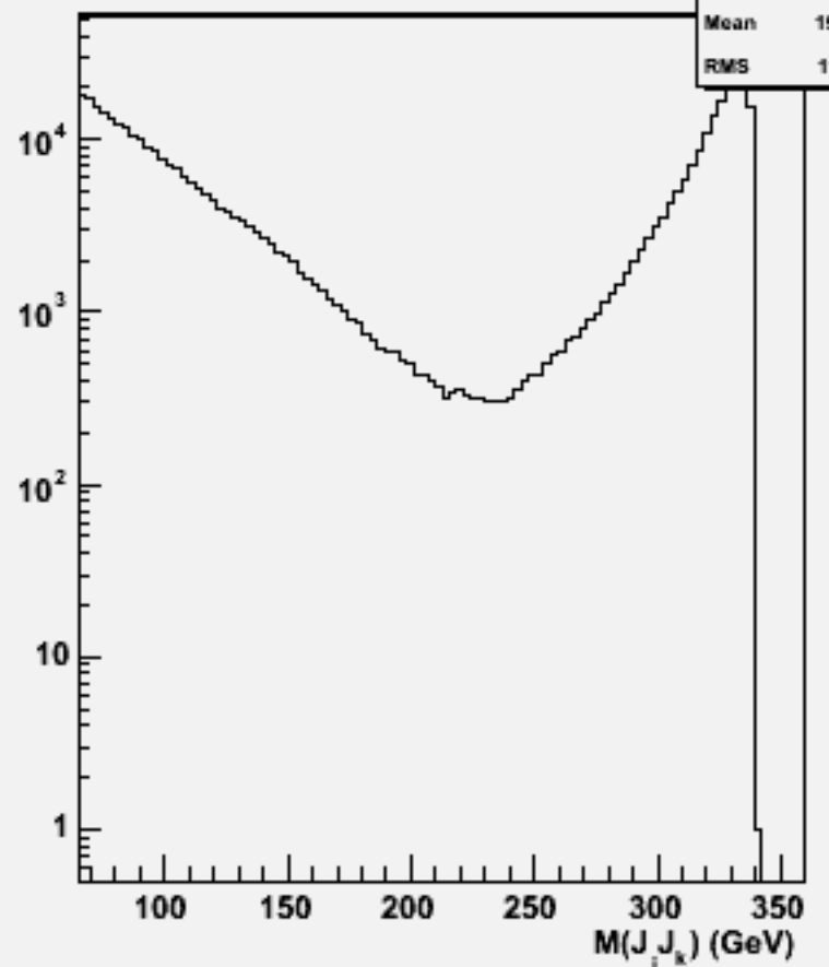
2jets mass(All comb)w102794 aa_ss_o
