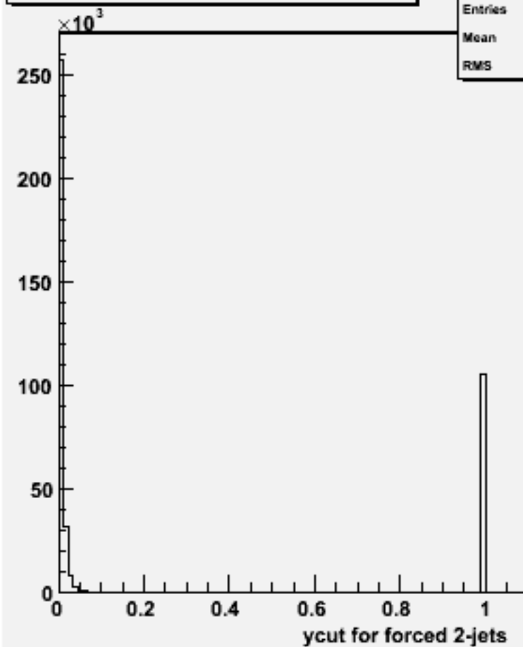
Ycut for 2-jets :w102794 aa_ss_o
