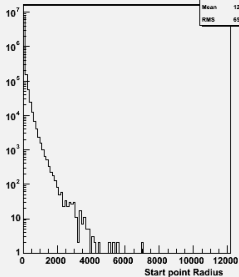
Start point R : w102794 aa_ss_o
