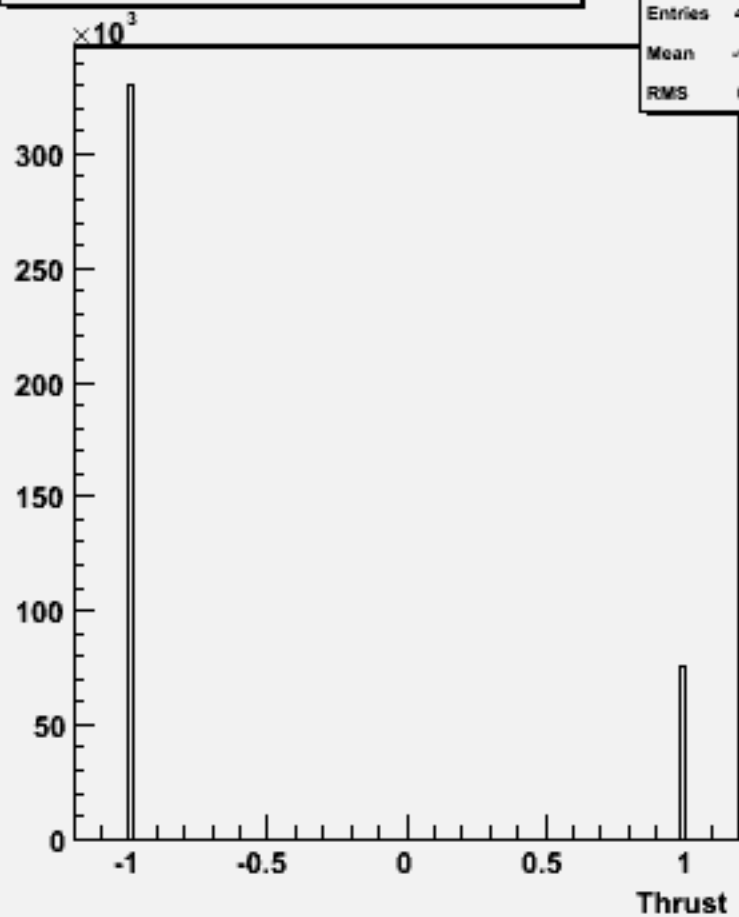
cos \Theta (thrust) w102794 aa_ss_o
