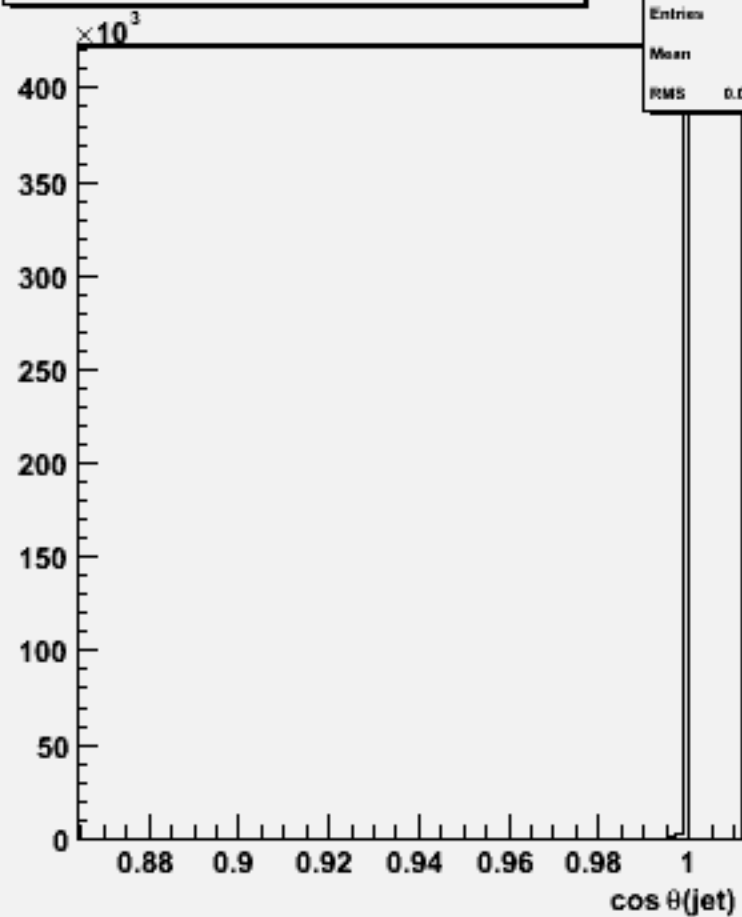
cos \theta for 2-jets :w102794 aa_ss_o
