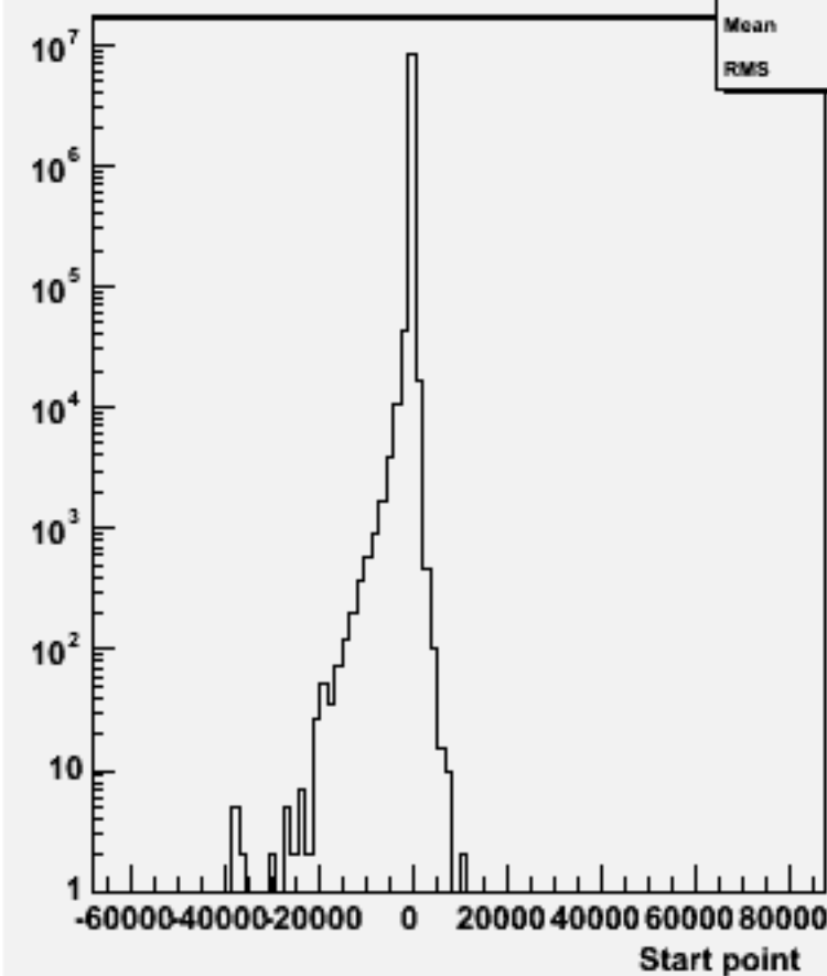
Start point Z : w102794 aa_ss_o
