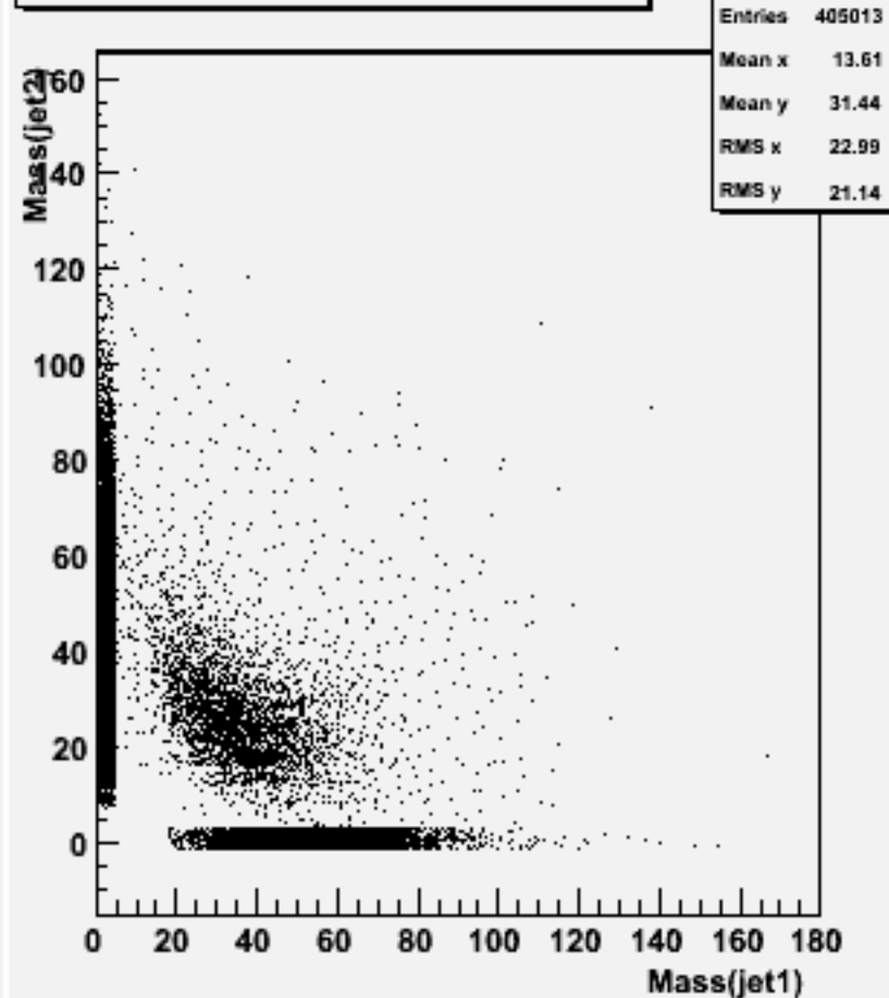
Jet mass for forced 2-jets : w102793 aa_ss_o
