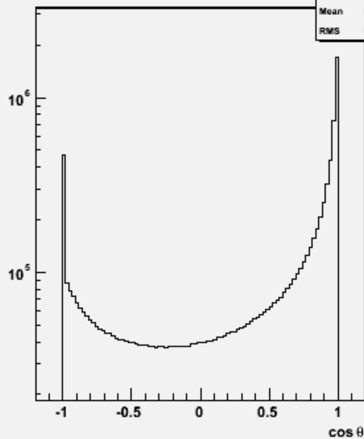
Particle cosθ : w102793 aa_ss_o
