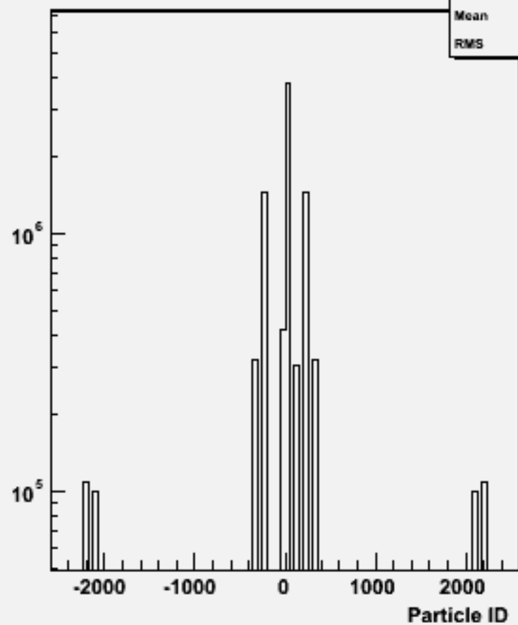
Particle ID : w102793 aa_ss_o
