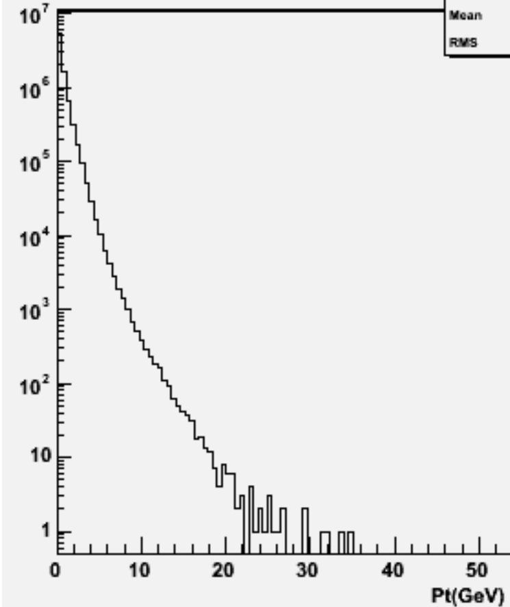
Particle Pt : w102793 aa_ss_o
