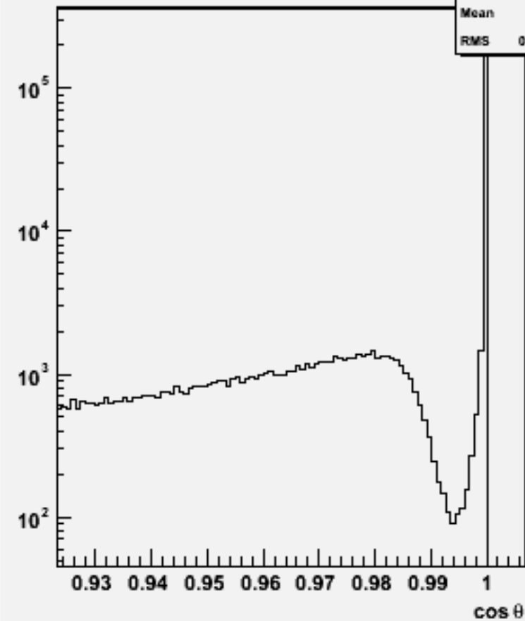
Jet cosθ (All jets)w102793 aa_ss_o
