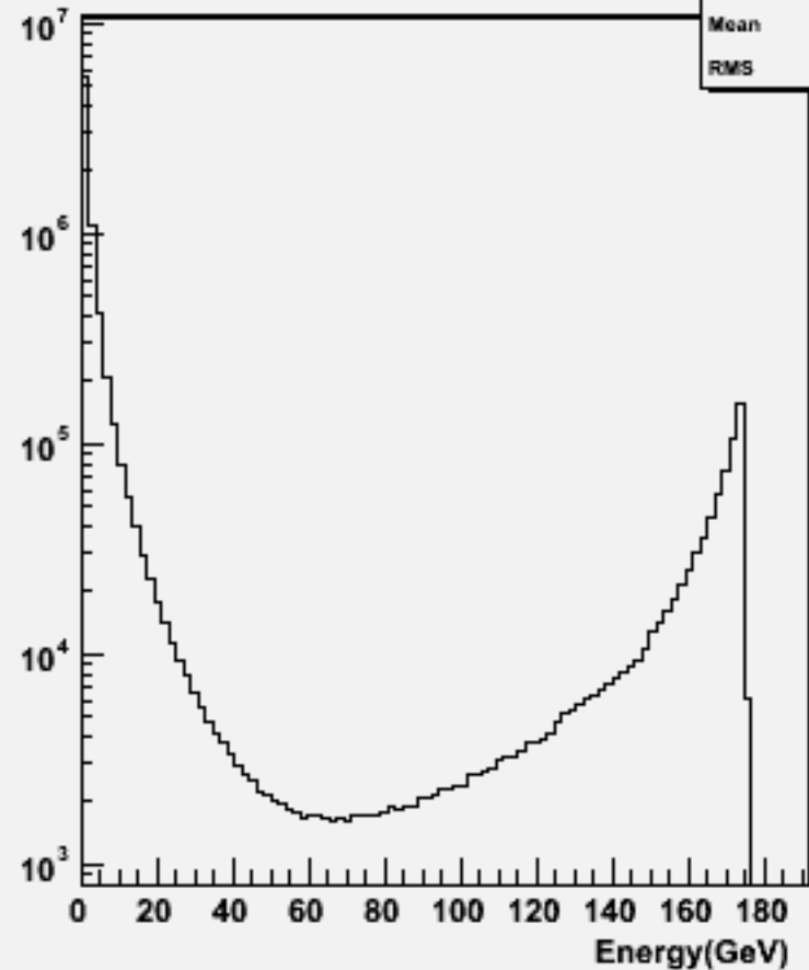
Particle Energy : w102793 aa_ss_o
