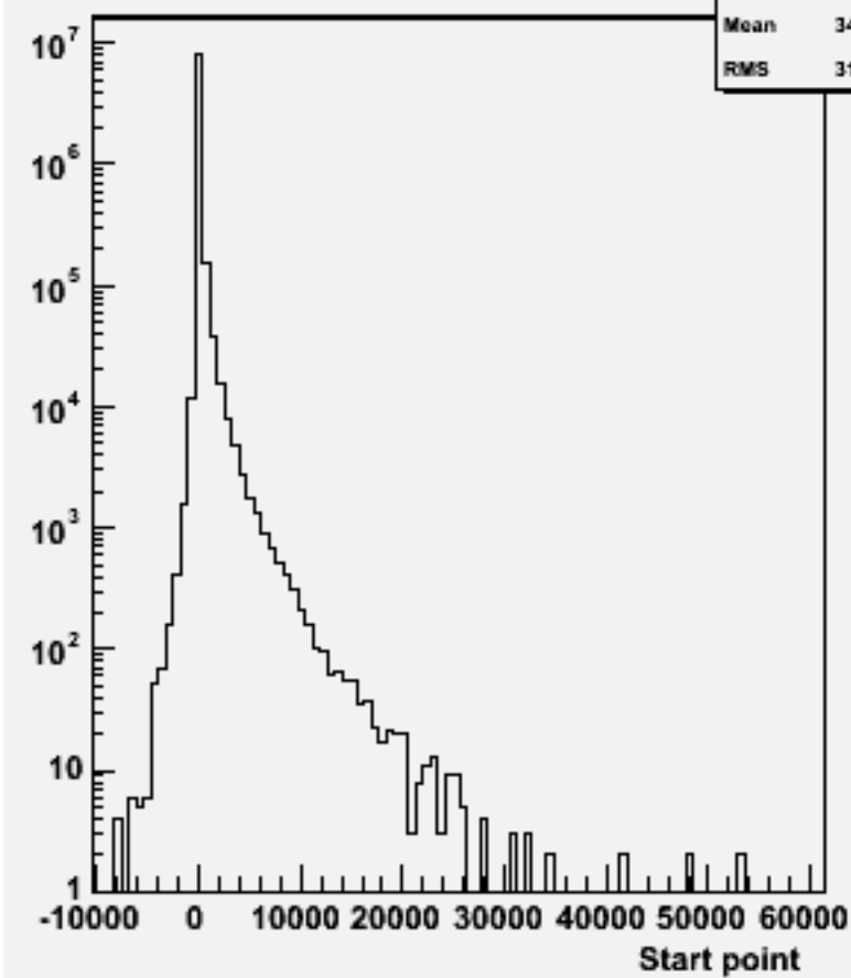
Start point Z : w102793 aa_ss_o
