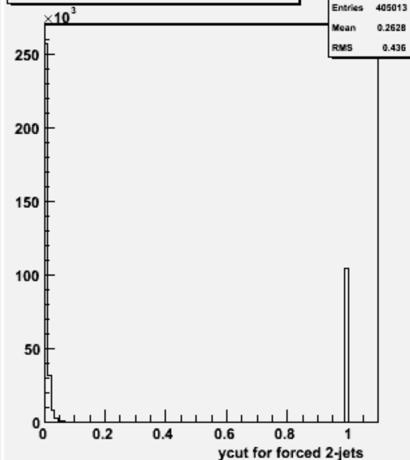
Ycut for 2-jets :w102793 aa_ss_o
