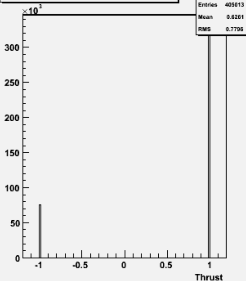
cos \Theta (thrust) w102793 aa_ss_o
