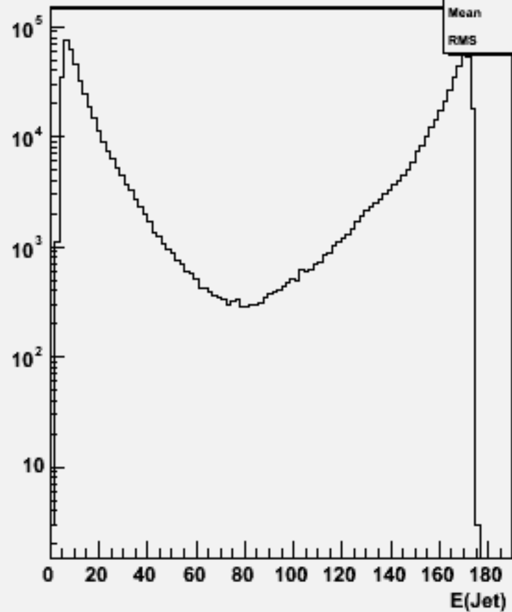
Jet energies(All jets)w102793 aa_ss_o
