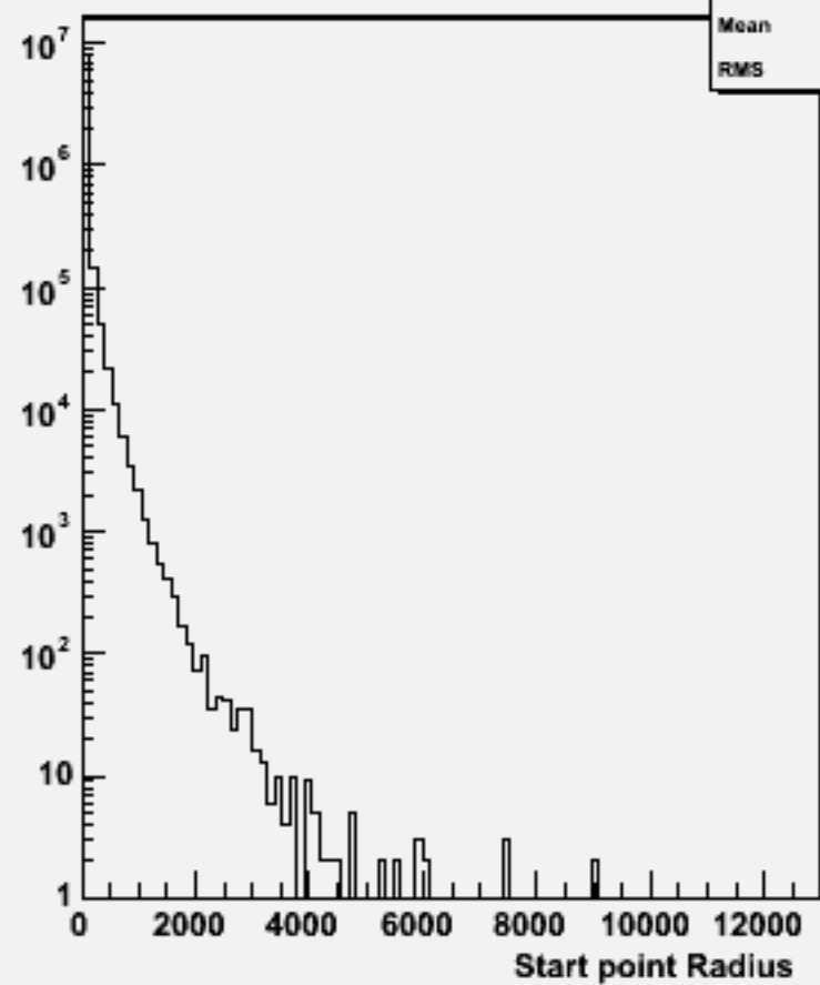
Start point R : w102793 aa_ss_o
