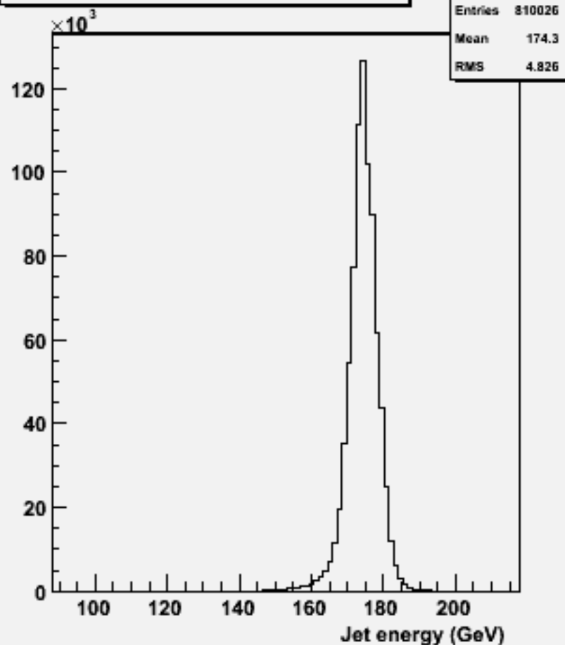
energy for 2-jets :w102793 aa_ss_o
