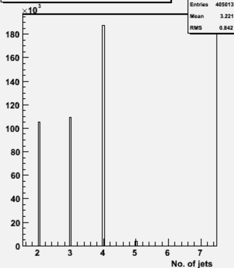
No. jets (ycut=0.001) : w102793 aa_ss_o
