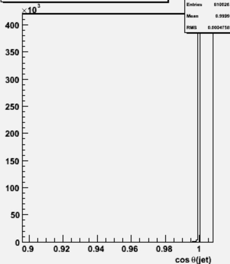
cos \theta for 2-jets :w102793 aa_ss_o
