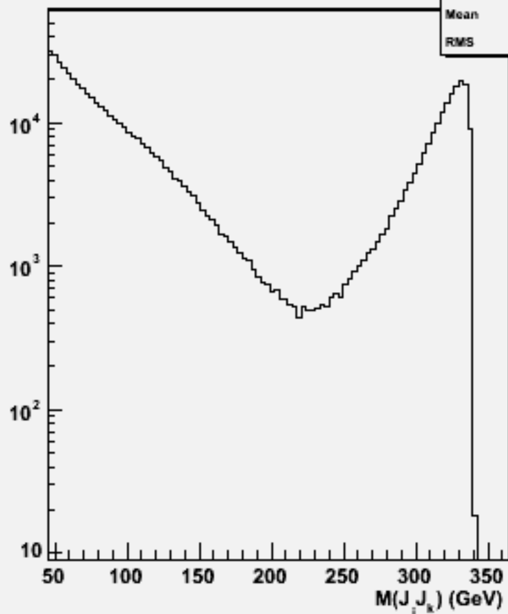
2jets mass(All comb)w102792 aa_ss_o
