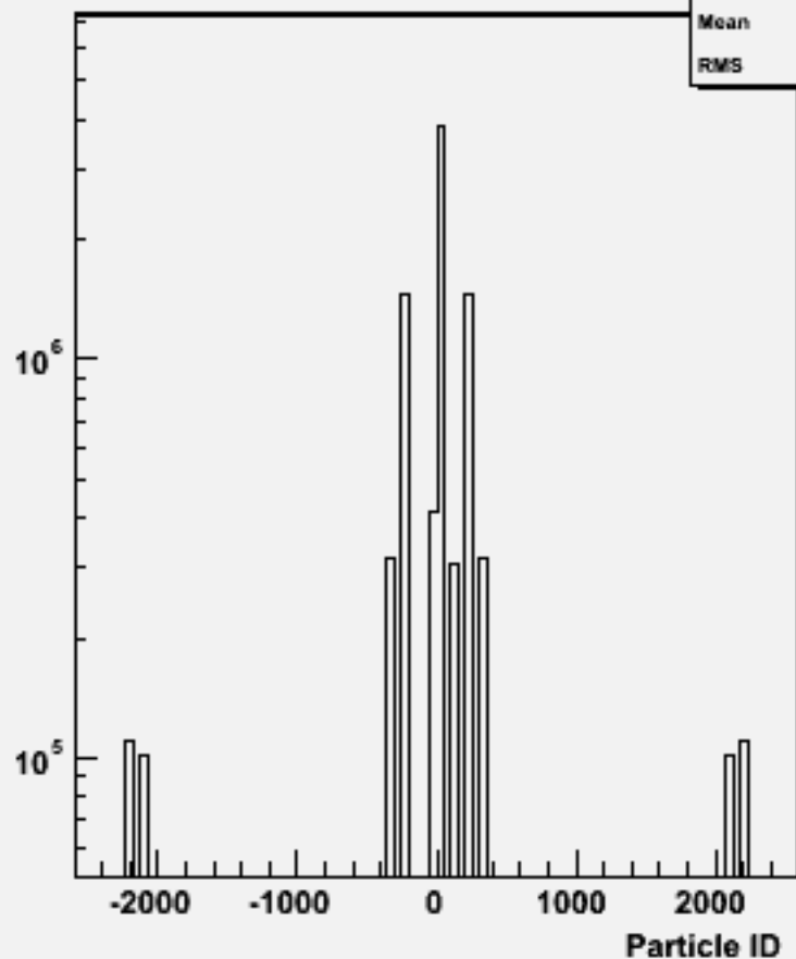
Particle ID : w102792 aa_ss_o
