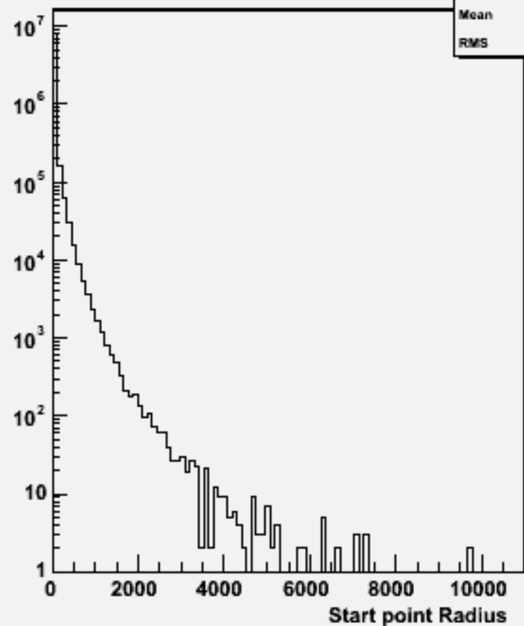
Start point R : w102792 aa_ss_o
