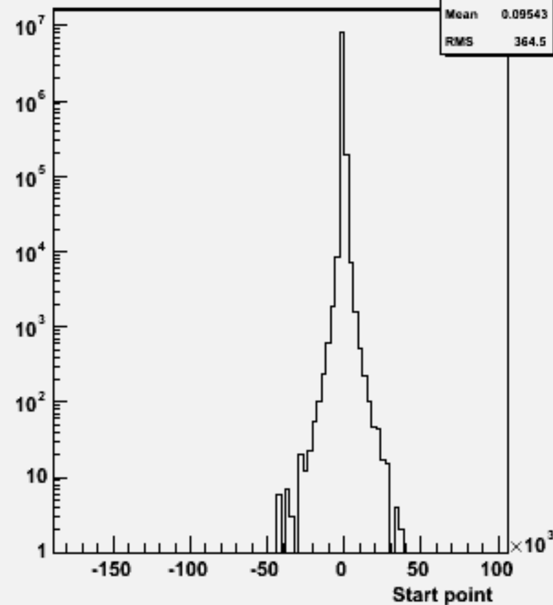
Start point Z : w102792 aa_ss_o
