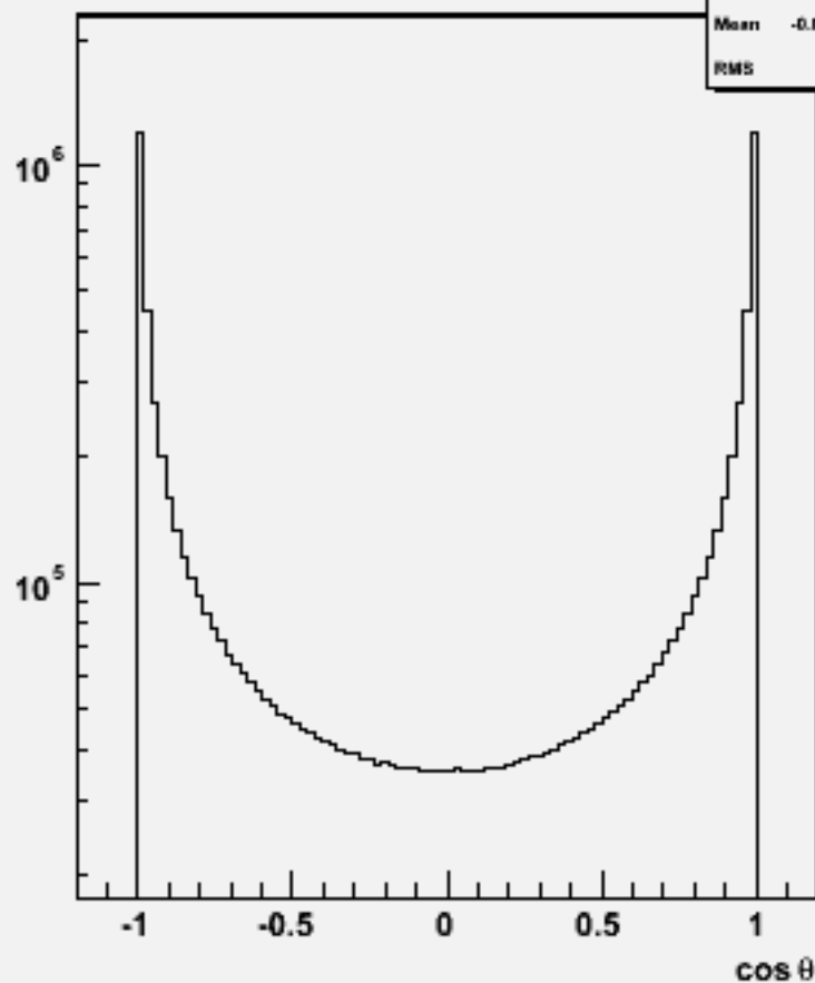
Particle cosθ : w102792 aa_ss_o
