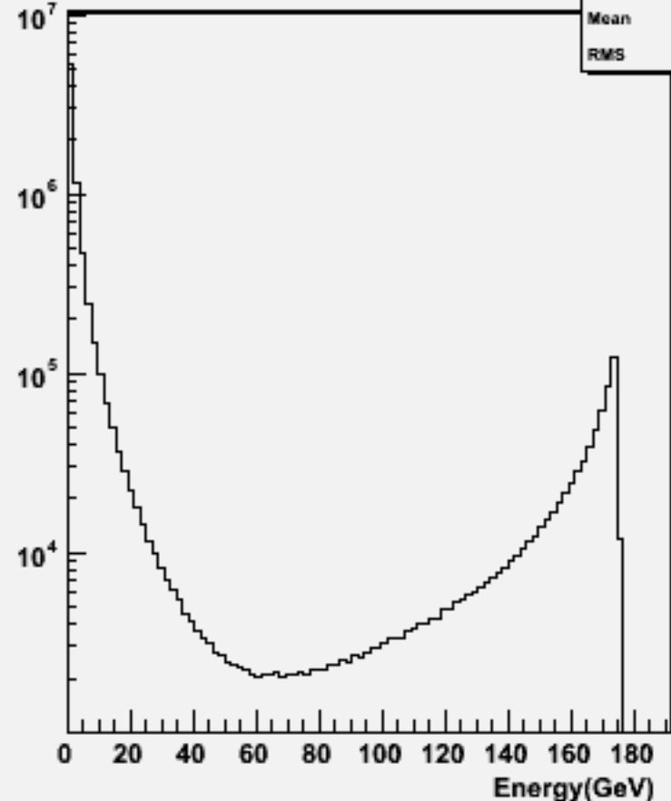
Particle Energy : w102792 aa_ss_o
