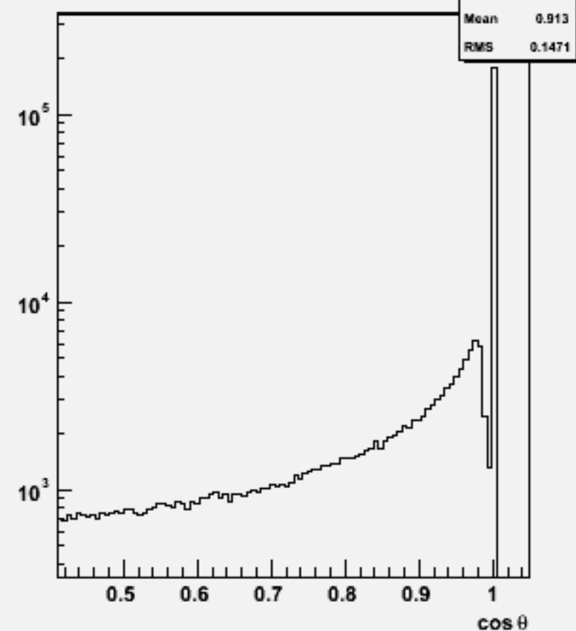
Jet cosθ (All jets)w102792 aa_ss_o
