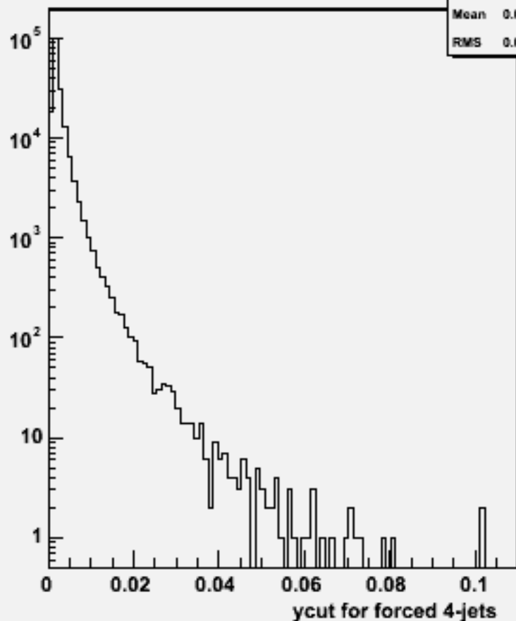
Ycut for 4-jets :w102792 aa_ss_o
