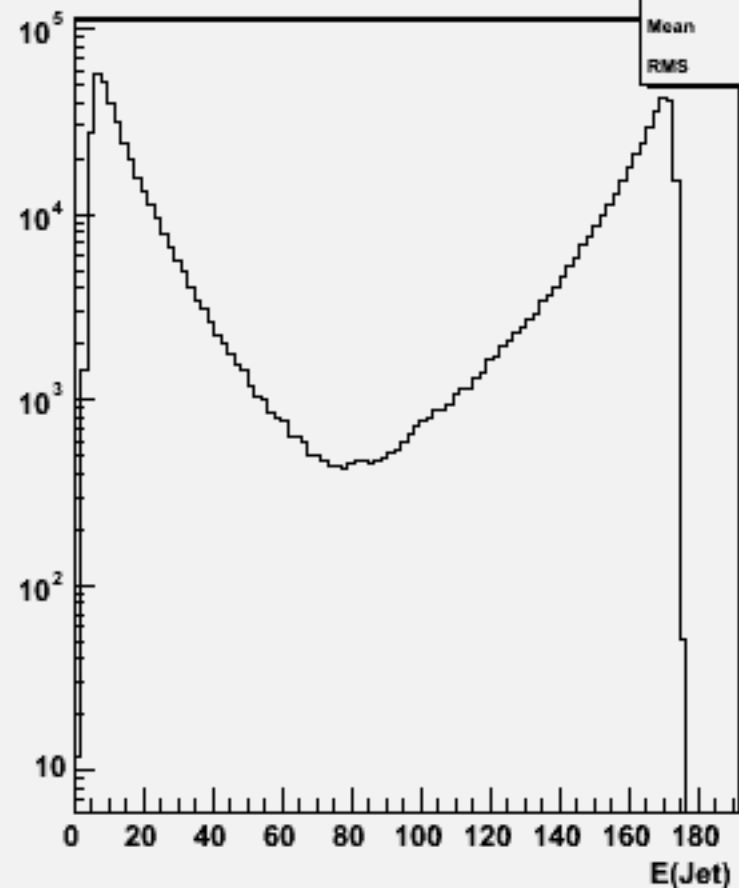
Jet energies(All jets)w102792 aa_ss_o
