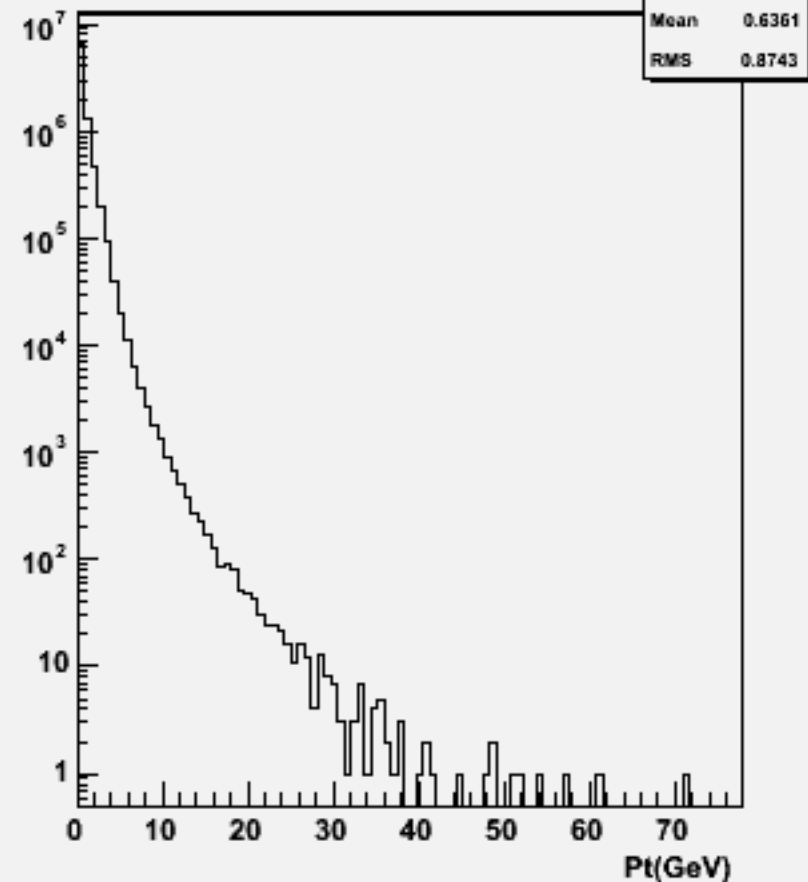
Particle Pt : w102792 aa_ss_o
