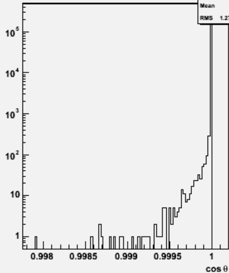
Jet cos \theta (All jets)w102791 aa_dd_o
