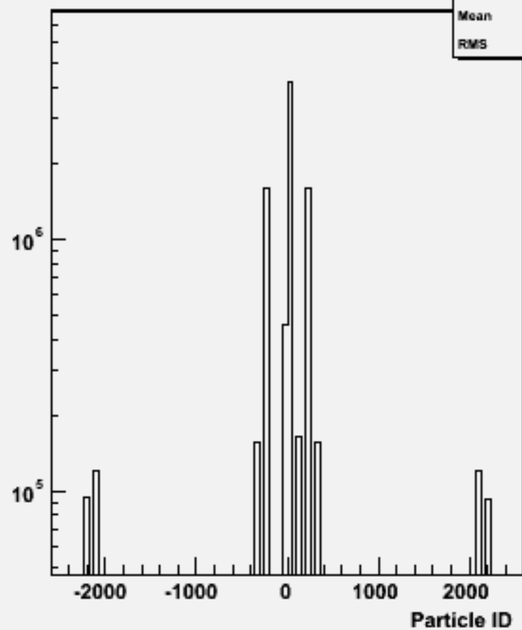
Particle ID : w102791 aa_dd_o
