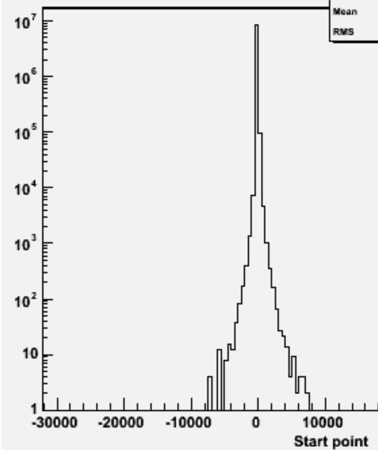
Start point Z : w102791 aa_dd_o
