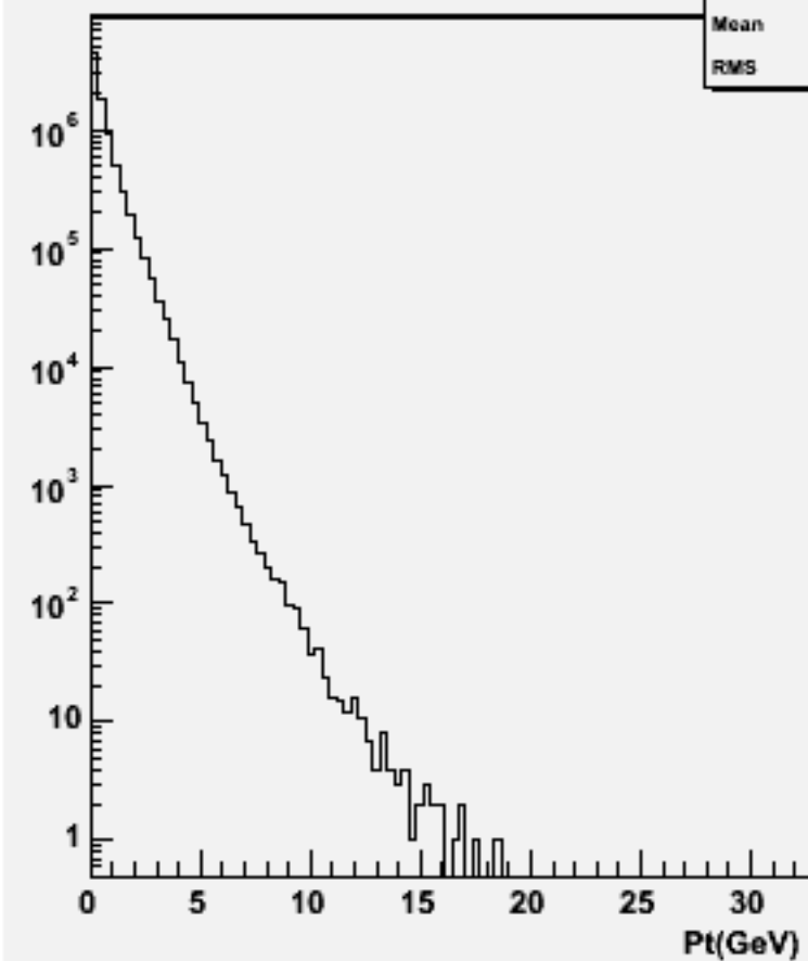
Particle Pt : w102791 aa_dd_o
