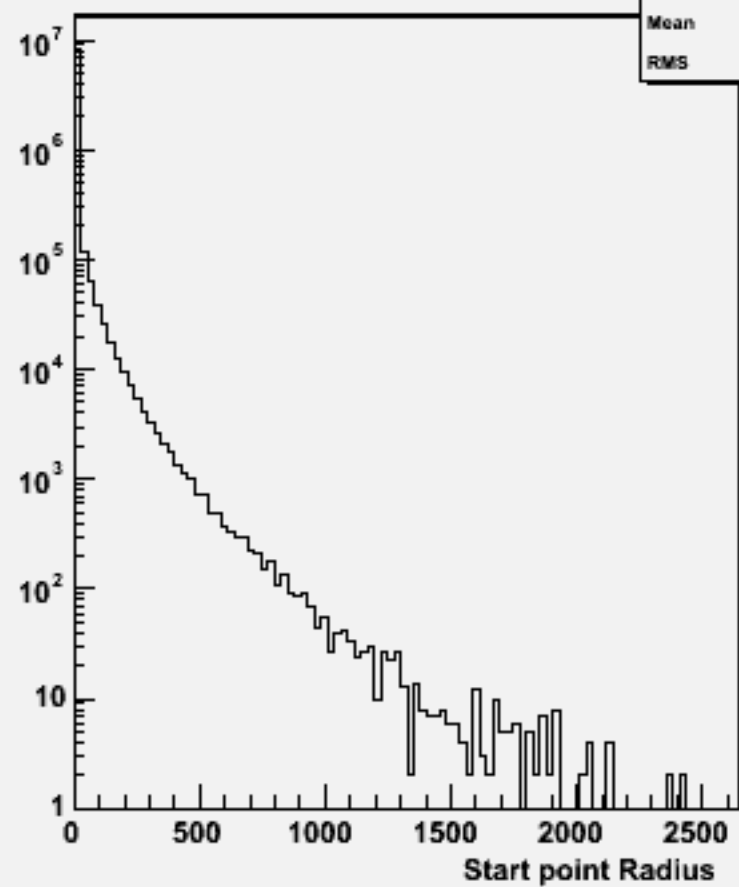
Start point R : w102791 aa_dd_o
