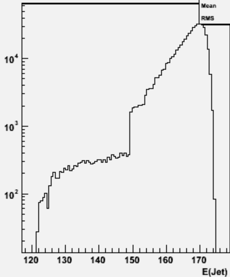
Jet energies(All jets)w102791 aa_dd_o
