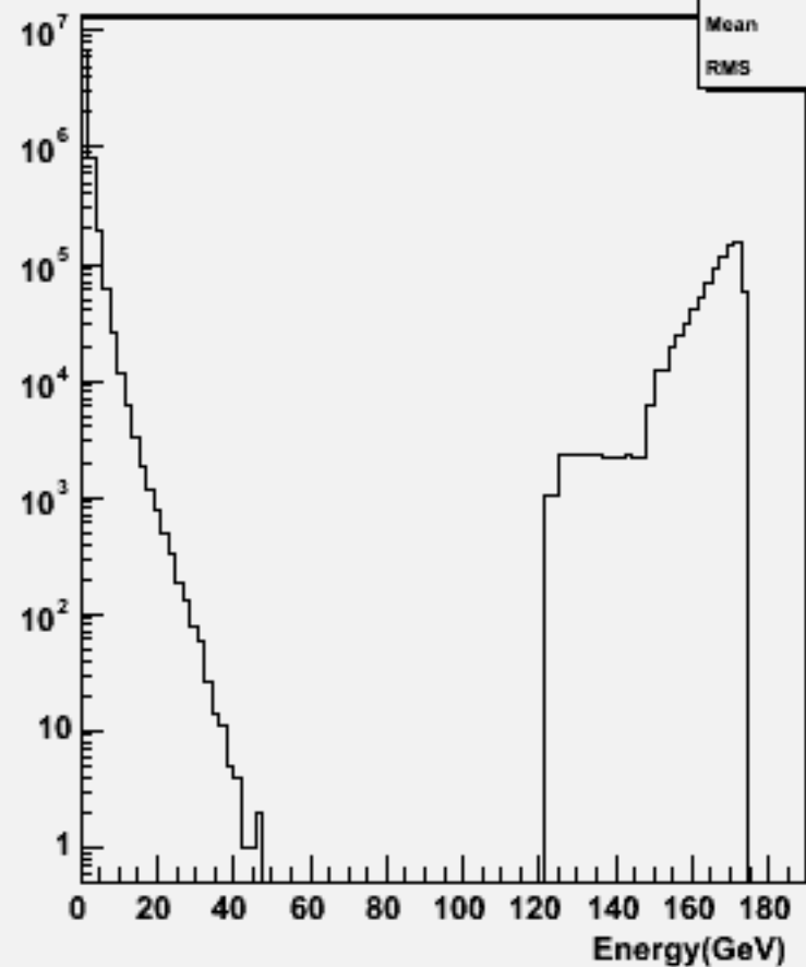
Particle Energy : w102791 aa_dd_o
