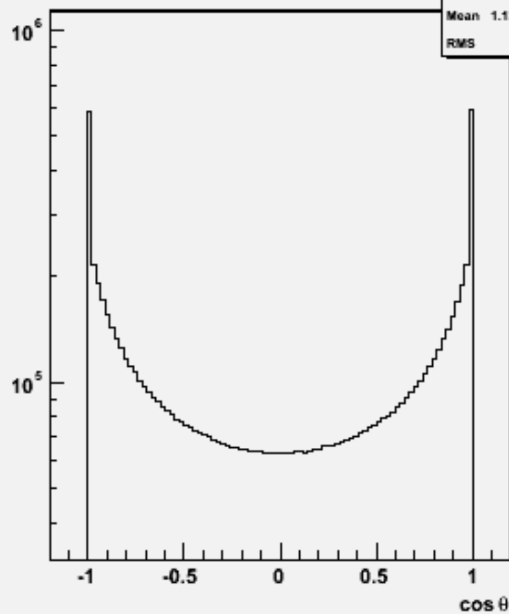
Particle \cos\theta : w102791 aa_dd_o
