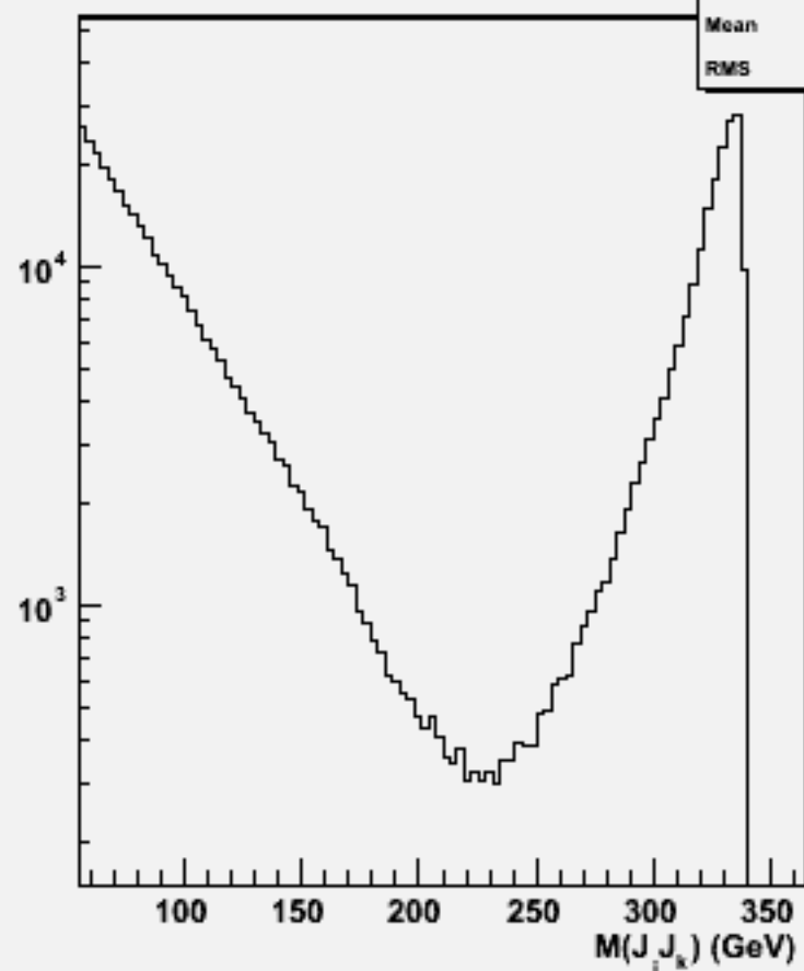
2jets mass(All comb)w102790 aa_dd_o
