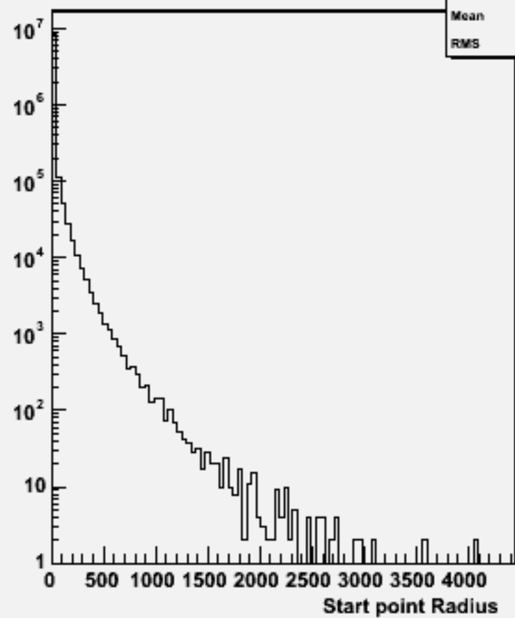
Start point R : w102790 aa_dd_o
