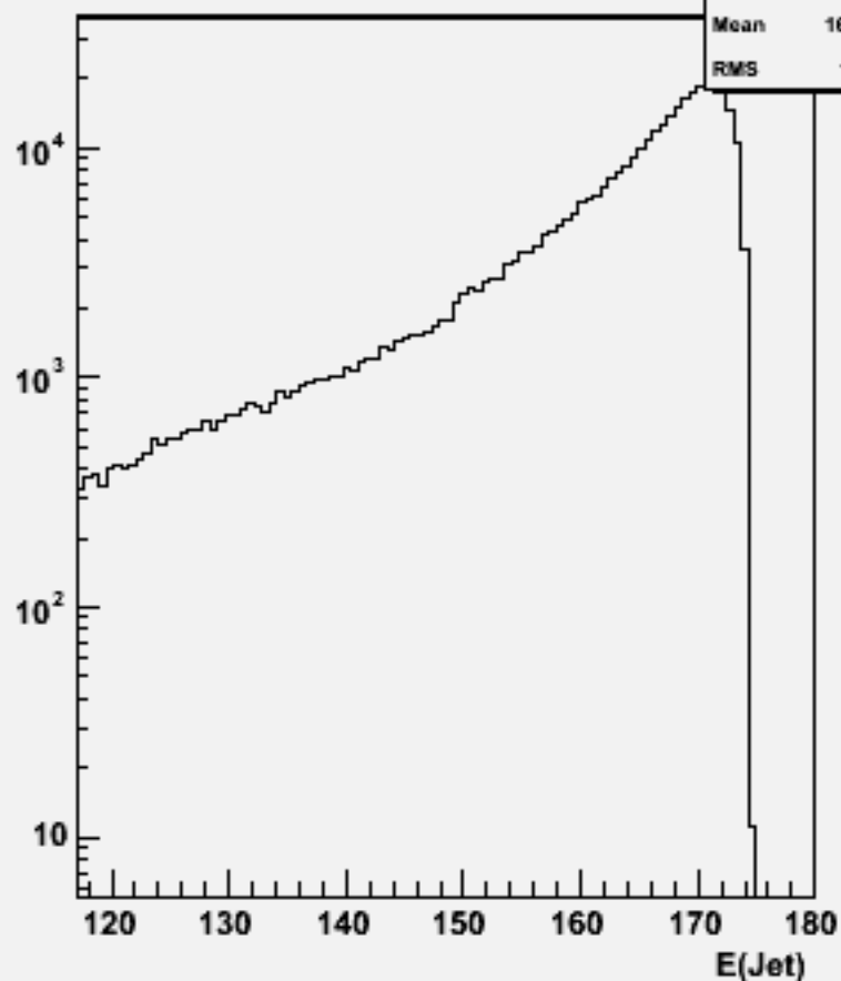
Jet energies(All jets)w102790 aa_dd_o
