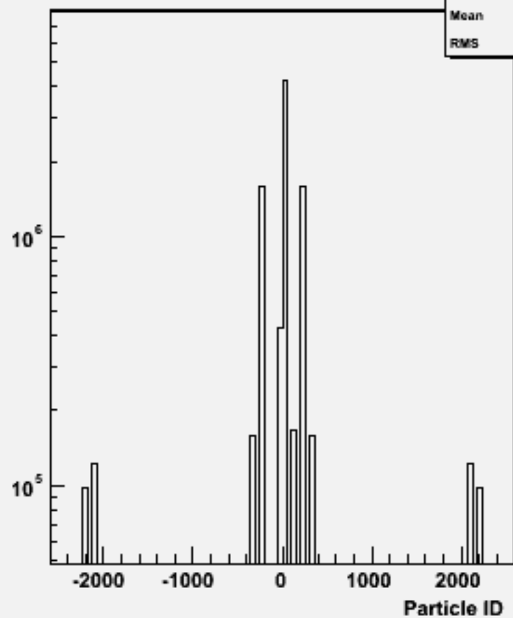
Particle ID : w102790 aa_dd_o
