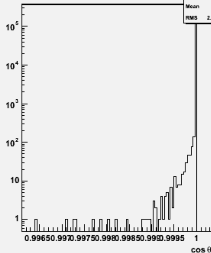
Jet cosθ (All jets)w102790 aa_dd_o
