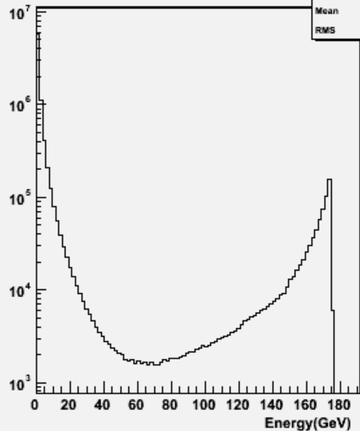
Particle Energy : w102790 aa_dd_o
