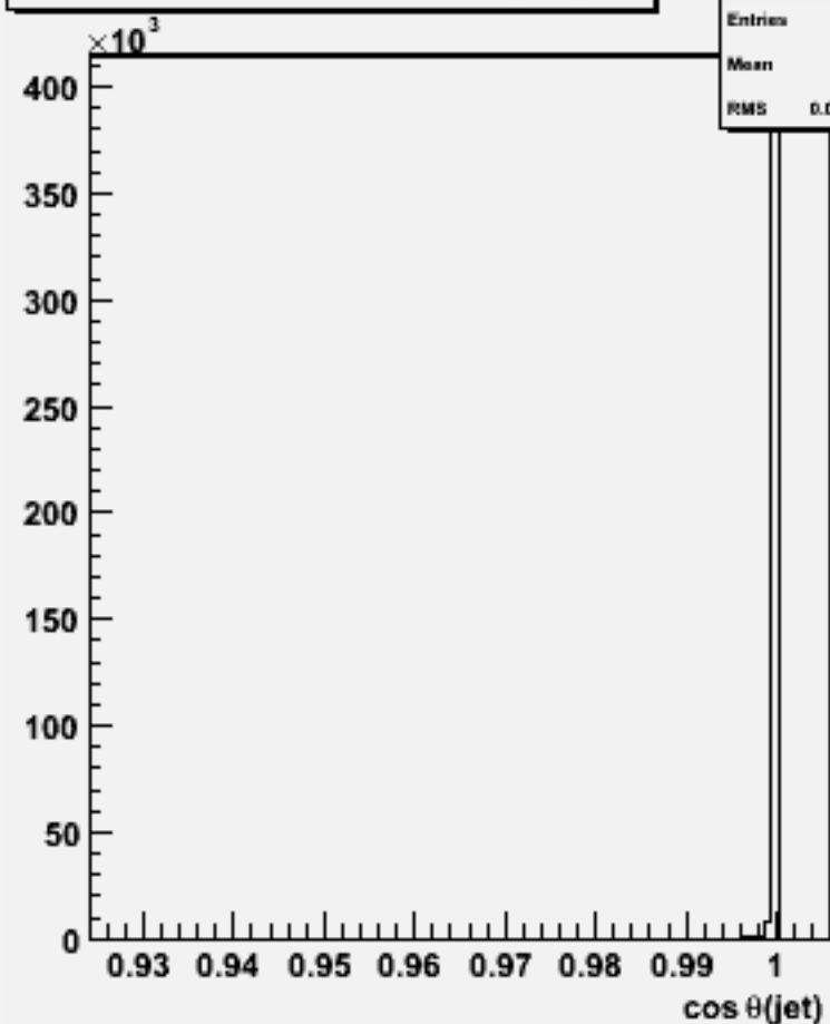
cos \theta for 2-jets :w102790 aa_dd_o
