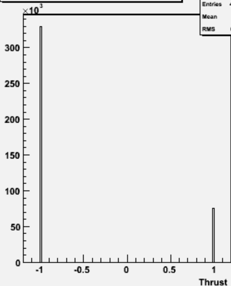
cos \Theta (thrust) w102790 aa_dd_o
