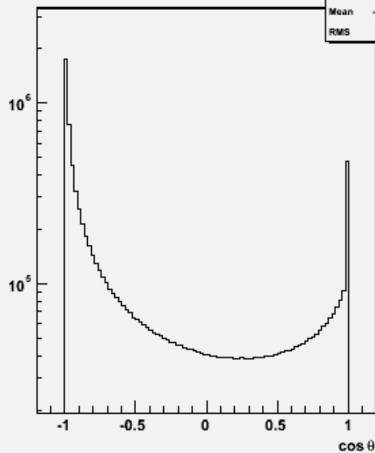
Particle cos \theta : w102790 aa_dd_o
