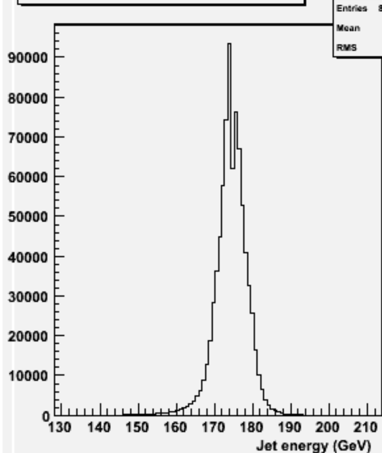
energy for 2-jets :w102790 aa_dd_o
