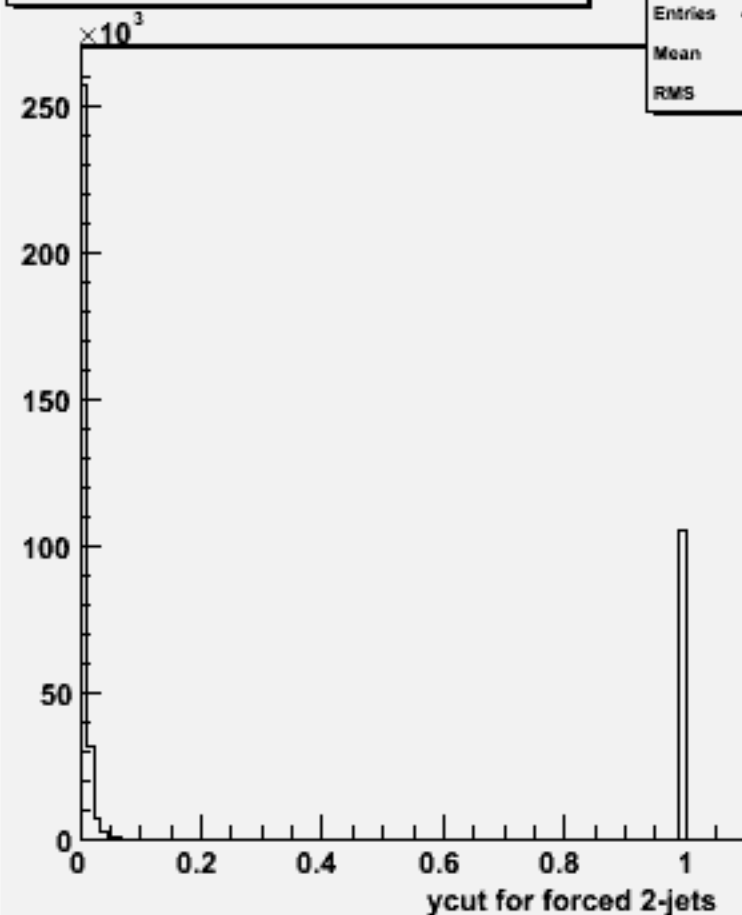
Ycut for 2-jets :w102790 aa_dd_o
