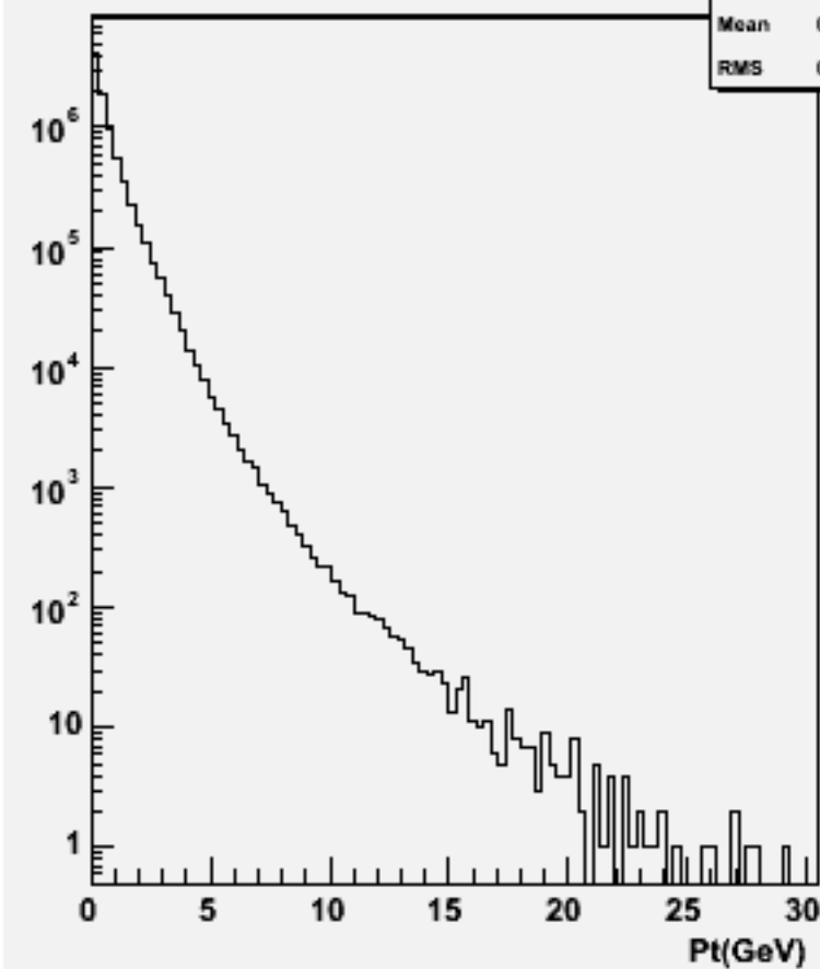
Particle Pt : w102790 aa_dd_o
