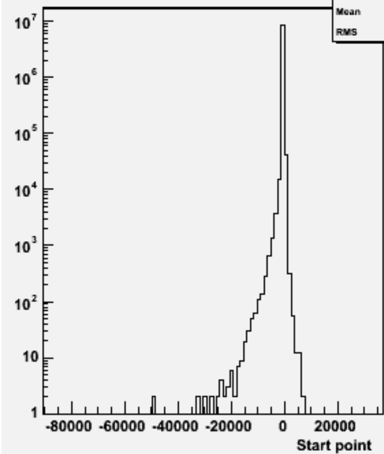
Start point Z : w102790 aa_dd_o
