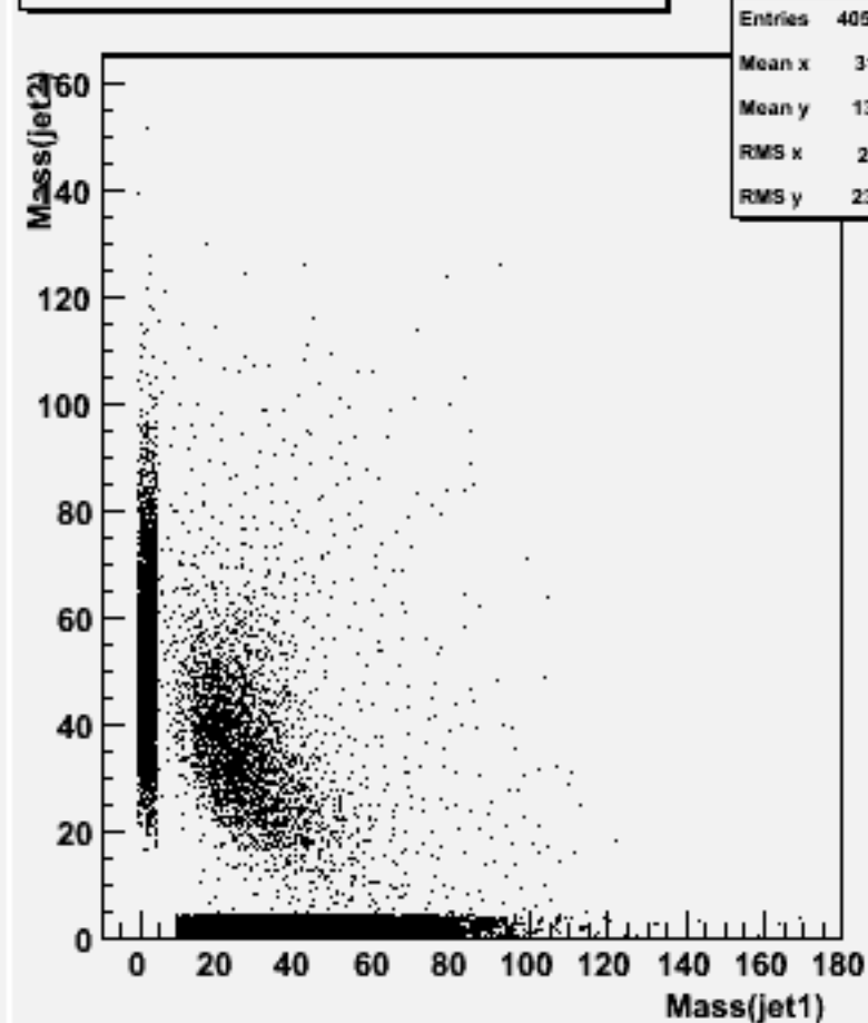
Jet mass for forced 2-jets : w102790 aa_dd_o
