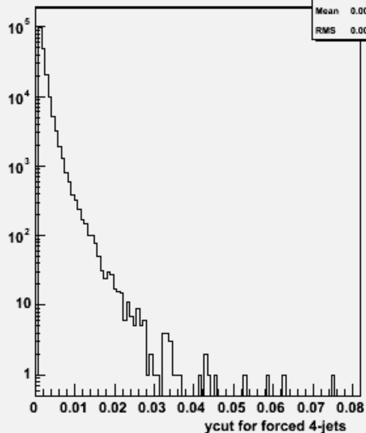
Ycut for 4-jets :w102790 aa_dd_o
