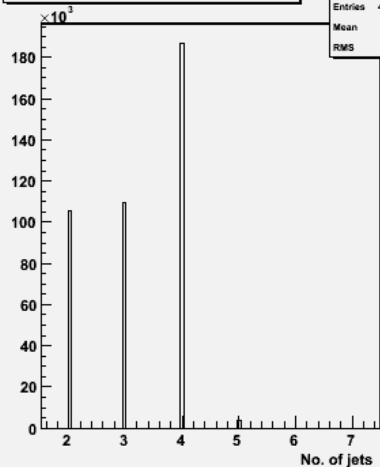
No. jets (ycut=0.001) : w102790 aa_dd_o
